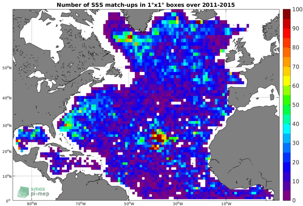
Figure 4: Number of SSS match-ups between Argo SSS and the Aquarius-L3-JPL-V5-7DAY-RUNNING SSS product for the North Atlantic Ocean Pi-MEP region over 1°x1° boxes and for the full satellite product period.
