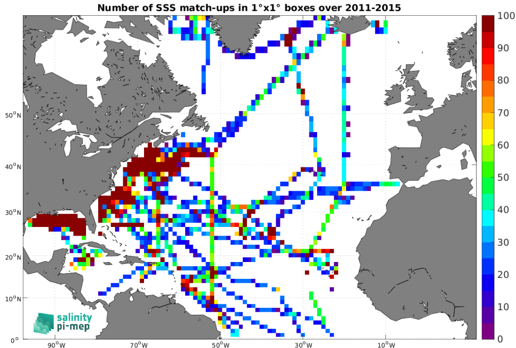
Figure 5: Number of SSS match-ups between TSG (SAMOS) SSS and the Aquarius SSS L3 CAP v5 - Monthly (JPL) SSS product for the North Atlantic Ocean Pi-MEP region over 1^\circ \times 1^\circ boxes and for the full satellite product period.
