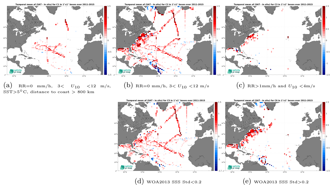
Figure 14: Temporal mean gridded over spatial boxes of size 1^\circ \times 1^\circ of \Delta\text{SSS} (Aquarius SSS L3 CAP v5 - Monthly (JPL) - TSG (SAMOS)) for 5 different subdatasets corresponding to:RR=0 mm/h, 3 < U_{10} < 12 m/s, SST >5^\circ\text{C} , distance to coast > 800 km (a), RR=0 mm/h, 3 < U_{10} < 12 m/s (b), RR >1 mm/h and U_{10} < 4 m/s (c), WOA2013 SSS Std <0.2 (d), WOA2013 SSS Std >0.2 (e).
