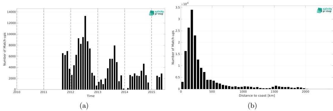
Figure 2: Number of match-ups between TSG (SAMOS) and Aquarius SSS L3 CAP v5 - Monthly (JPL) SSS as a function of time (a) and as function of the distance to coast (b) over the North Atlantic Ocean Pi-MEP region and for the full satellite product period.
