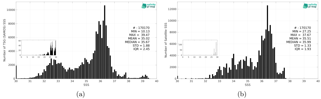
Figure 3: Histograms of SSS from TSG (SAMOS) (a) and Aquarius SSS L3 CAP v5 - Monthly (JPL) (b) considering all match-up pairs per bins of 0.1 over the North Atlantic Ocean Pi-MEP region and for the full satellite product period.
