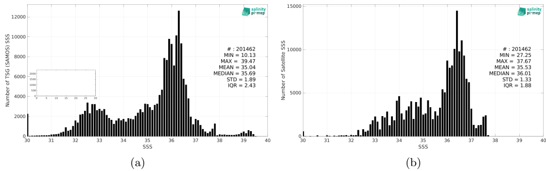
Figure 2: Histograms of SSS from TSG (SAMOS) (a) and Aquarius SSS L3 CAP v5 - Monthly (JPL) (b) considering all match-up pairs per bins of 0.1 over the North Atlantic Ocean Pi-MEP region and for the full satellite product period.
