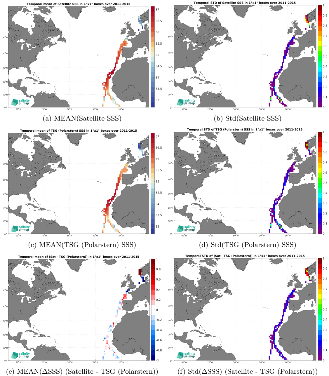
Figure 7: Temporal mean (left) and Std (right) of SSS from Aquarius SSS L3 CAP v5 - Monthly (JPL) (top), TSG (Polarstern) (middle), and of \Delta SSS (Satellite - TSG (Polarstern)). Only match-up pairs are used to generate these maps.
