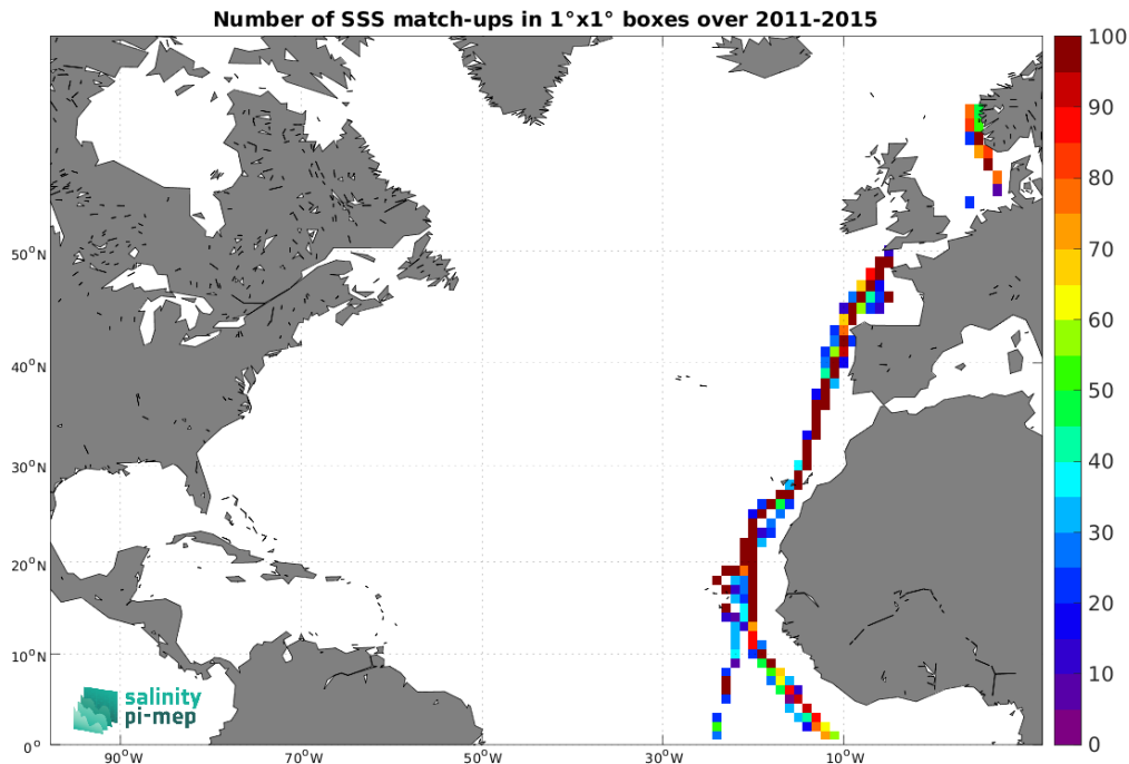
Figure 5: Number of SSS match-ups between TSG (Polarstern) SSS and the Aquarius SSS L3 CAP v5 - Monthly (JPL) SSS product for the North Atlantic Ocean Pi-MEP region over 1^\circ \times 1^\circ boxes and for the full satellite product period.
