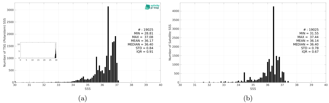
Figure 3: Histograms of SSS from TSG (Polarstern) (a) and Aquarius SSS L3 CAP v5 - Monthly (JPL) (b) considering all match-up pairs per bins of 0.1 over the North Atlantic Ocean Pi-MEP region and for the full satellite product period.
