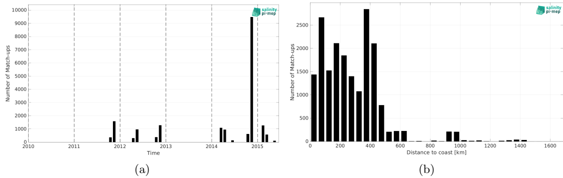
Figure 2: Number of match-ups between TSG (Polarstern) and Aquarius SSS L3 CAP v5 - Monthly (JPL) SSS as a function of time (a) and as function of the distance to coast (b) over the North Atlantic Ocean Pi-MEP region and for the full satellite product period.
