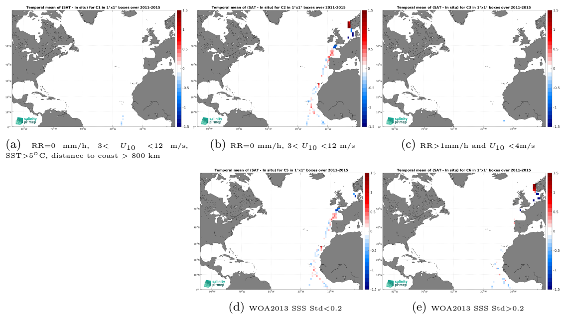
Figure 14: Temporal mean gridded over spatial boxes of size 1^\circ \times 1^\circ of \Delta\text{SSS} (Aquarius SSS L3 CAP v5 - Monthly (JPL) - TSG (Polarstern)) for 5 different subdatasets corresponding to:RR=0 mm/h, 3 < U_{10} < 12 m/s, SST >5^\circ\text{C} , distance to coast > 800 km (a), RR=0 mm/h, 3 < U_{10} < 12 m/s (b), RR >1 mm/h and U_{10} < 4 m/s (c), WOA2013 SSS Std <0.2 (d), WOA2013 SSS Std >0.2 (e).
