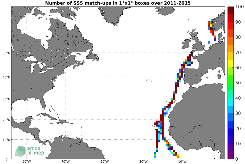
Figure 4: Number of SSS match-ups between TSG (Polarstern) SSS and the Aquarius SSS L3 CAP v5 - Monthly (JPL) SSS product for the North Atlantic Ocean Pi-MEP region over 1°x1° boxes and for the full satellite product period.
