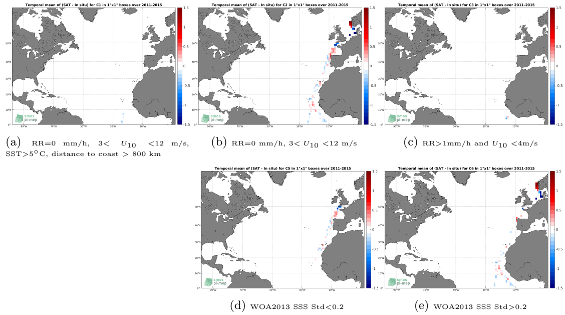
Figure 12: Temporal mean gridded over spatial boxes of size 1^\circ \times 1^\circ of \Delta SSS (Aquarius SSS L3 CAP v5 - Monthly (JPL) - TSG (Polarstern)) for 5 different subdatasets corresponding to: RR=0 mm/h, 3 < U_{10} < 12 m/s, SST > 5^\circ\text{C} , distance to coast > 800 km (a), RR=0 mm/h, 3 < U_{10} < 12 m/s (b), RR > 1 mm/h and U_{10} < 4 m/s (c), WOA2013 SSS Std < 0.2 (d), WOA2013 SSS Std > 0.2 (e).
