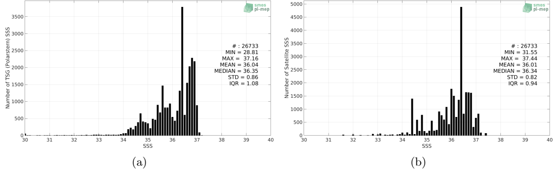
Figure 2: Histograms of SSS from TSG (Polarstern) (a) and Aquarius SSS L3 CAP v5 - Monthly (JPL) (b) considering all match-up pairs per bins of 0.1 over the North Atlantic Ocean Pi-MEP region and for the full satellite product period.
