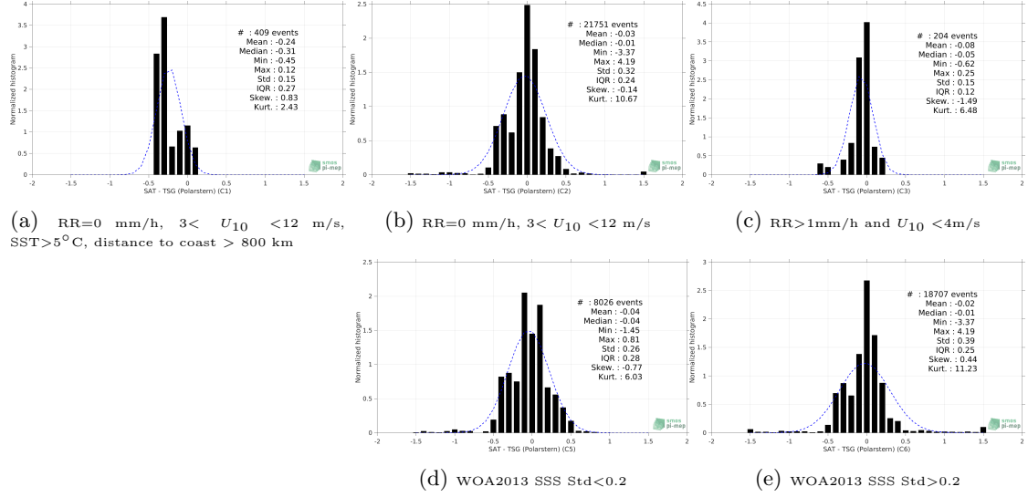
Figure 13: Normalized histogram of \Delta SSS (Aquarius SSS L3 CAP v5 - Monthly (JPL) - TSG (Polarstern)) for 5 different subdatasets corresponding to: RR=0 mm/h, 3 < U_{10} < 12 m/s, SST>5°C, distance to coast > 800 km (a), RR=0 mm/h, 3 < U_{10} < 12 m/s (b), RR>1mm/h and U_{10} < 4 m/s (c), WOA2013 SSS Std<0.2 (d), WOA2013 SSS Std>0.2 (e).
