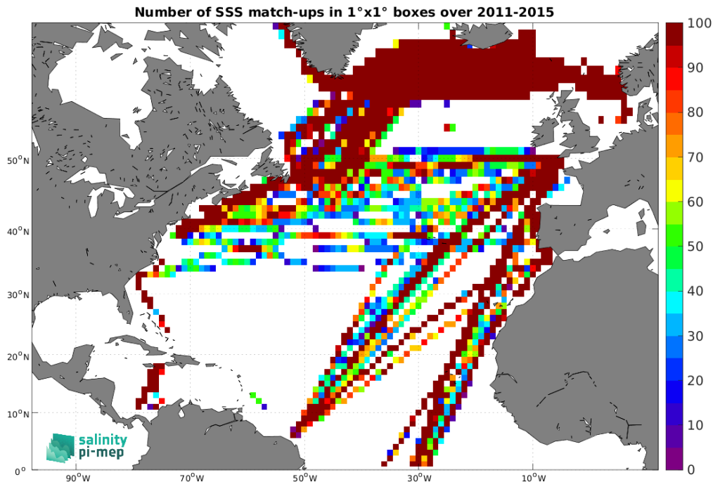
Figure 5: Number of SSS match-ups between TSG (LEGOS-DM) SSS and the Aquarius SSS L3 CAP v5 - Monthly (JPL) SSS product for the North Atlantic Ocean Pi-MEP region over 1^\circ \times 1^\circ boxes and for the full satellite product period.
