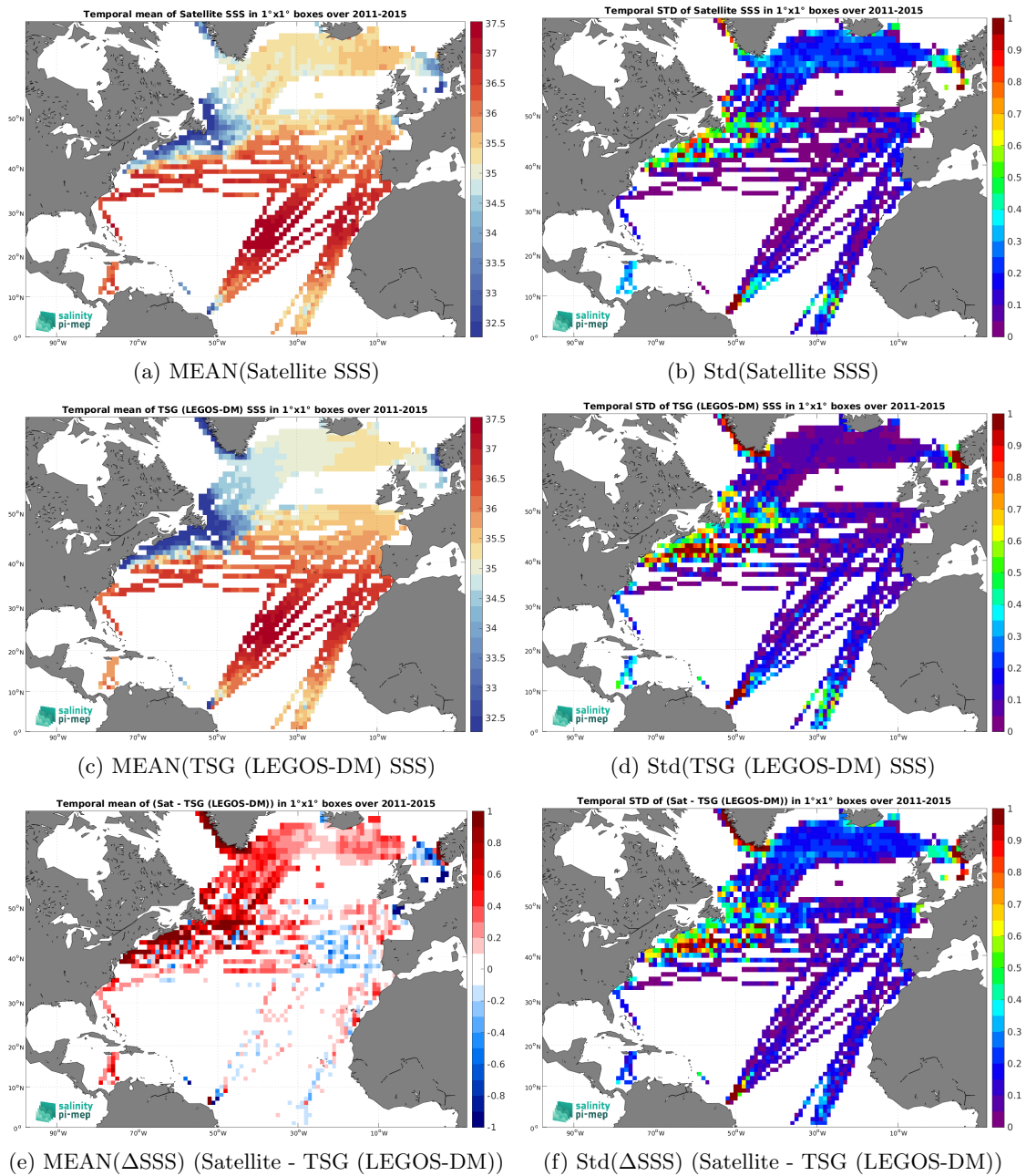
Figure 7: Temporal mean (left) and Std (right) of SSS from Aquarius SSS L3 CAP v5 - Monthly (JPL) (top), TSG (LEGOS-DM) (middle), and of \Delta SSS (Satellite - TSG (LEGOS-DM)). Only match-up pairs are used to generate these maps.
