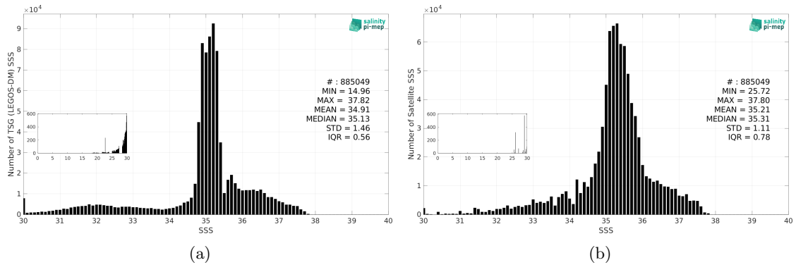
Figure 3: Histograms of SSS from TSG (LEGOS-DM) (a) and Aquarius SSS L3 CAP v5 - Monthly (JPL) (b) considering all match-up pairs per bins of 0.1 over the North Atlantic Ocean Pi-MEP region and for the full satellite product period.
