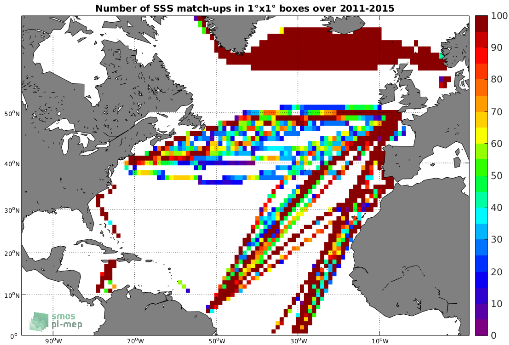
Figure 4: Number of SSS match-ups between TSG-LEGOS-DM SSS and the Aquarius-L3-JPL-V5-MONTHLY SSS product for the North Atlantic Ocean Pi-MEP region over 1^\circ \times 1^\circ boxes and for the full satellite product period.
