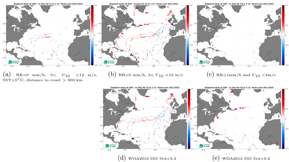
Figure 14: Temporal mean gridded over spatial boxes of size 1^\circ \times 1^\circ of \Delta\text{SSS} (Aquarius SSS L3 CAP v5 - Monthly (JPL) - TSG (GOSUD-Sailing-ship)) for 5 different subdatasets corresponding to:RR=0 mm/h, 3 < U_{10} < 12 m/s, SST >5^\circ\text{C} , distance to coast > 800 km (a), RR=0 mm/h, 3 < U_{10} < 12 m/s (b), RR >1 mm/h and U_{10} < 4 m/s (c), WOA2013 SSS Std <0.2 (d), WOA2013 SSS Std >0.2 (e).
