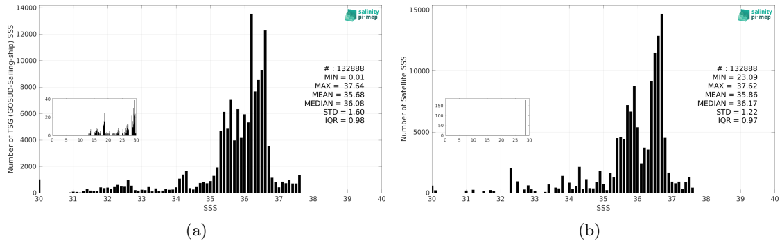
Figure 3: Histograms of SSS from TSG (GOSUD-Sailing-ship) (a) and Aquarius SSS L3 CAP v5 - Monthly (JPL) (b) considering all match-up pairs per bins of 0.1 over the North Atlantic Ocean Pi-MEP region and for the full satellite product period.
