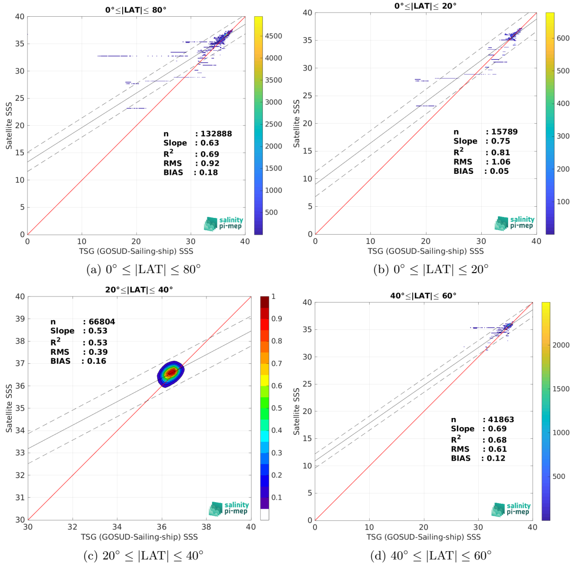
Figure 10: Contour maps of the concentration of Aquarius SSS L3 CAP v5 - Monthly (JPL) SSS (y-axis) versus TSG (GOSUD-Sailing-ship) SSS (x-axis) at match-up pairs for different latitude bands. For each plot, the red line shows x=y . The black thin and dashed lines indicate a linear fit through the data cloud and the \pm 95\% confidence levels, respectively. The number match-up pairs n , the slope and R^2 coefficient of the linear fit, the root mean square (RMS) and the mean bias between satellite and in situ data are indicated for each latitude band in each plots.
