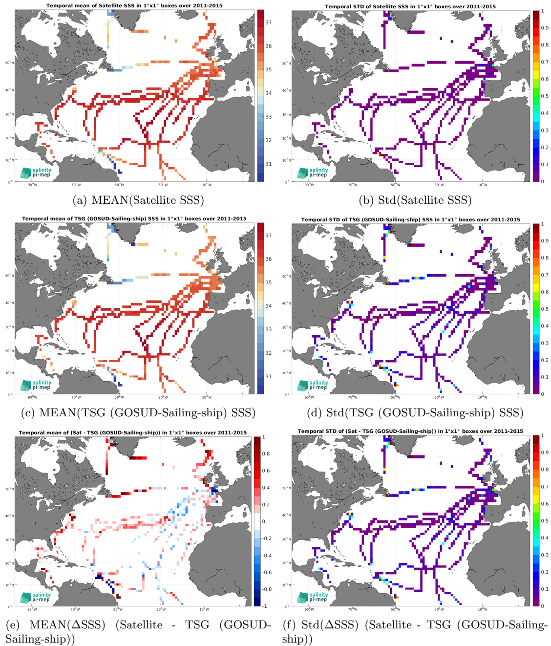
Figure 7: Temporal mean (left) and Std (right) of SSS from Aquarius SSS L3 CAP v5 - Monthly (JPL) (top), TSG (GOSUD-Sailing-ship) (middle), and of \Delta SSS (Satellite - TSG (GOSUD-Sailing-ship)). Only match-up pairs are used to generate these maps.
