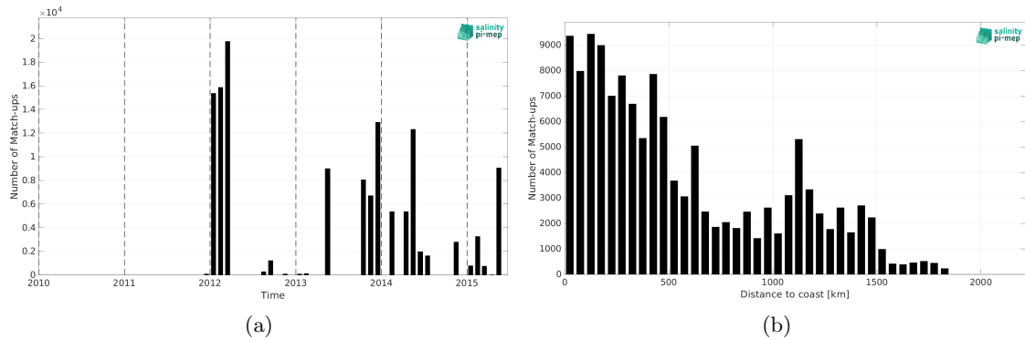
Figure 2: Number of match-ups between TSG (GOSUD-Sailing-ship) and Aquarius SSS L3 CAP v5 - Monthly (JPL) SSS as a function of time (a) and as function of the distance to coast (b) over the North Atlantic Ocean Pi-MEP region and for the full satellite product period.
