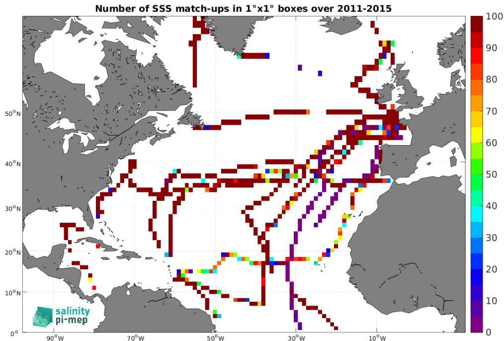
Figure 5: Number of SSS match-ups between TSG (GOSUD-Sailing-ship) SSS and the Aquarius SSS L3 CAP v5 - Monthly (JPL) SSS product for the North Atlantic Ocean Pi-MEP region over 1^\circ \times 1^\circ boxes and for the full satellite product period.
