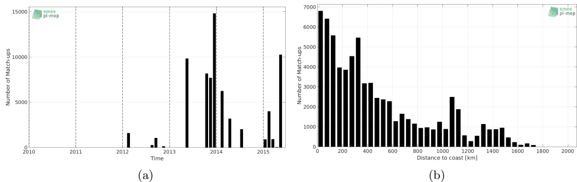
Figure 1: Number of match-ups between TSG-GOSUD-Sailing-ship and Aquarius-L3-JPL-V5-MONTHLY SSS as a function of time (a) and as function of the distance to coast (b) over the North Atlantic Ocean Pi-MEP region and for the full satellite product period.
