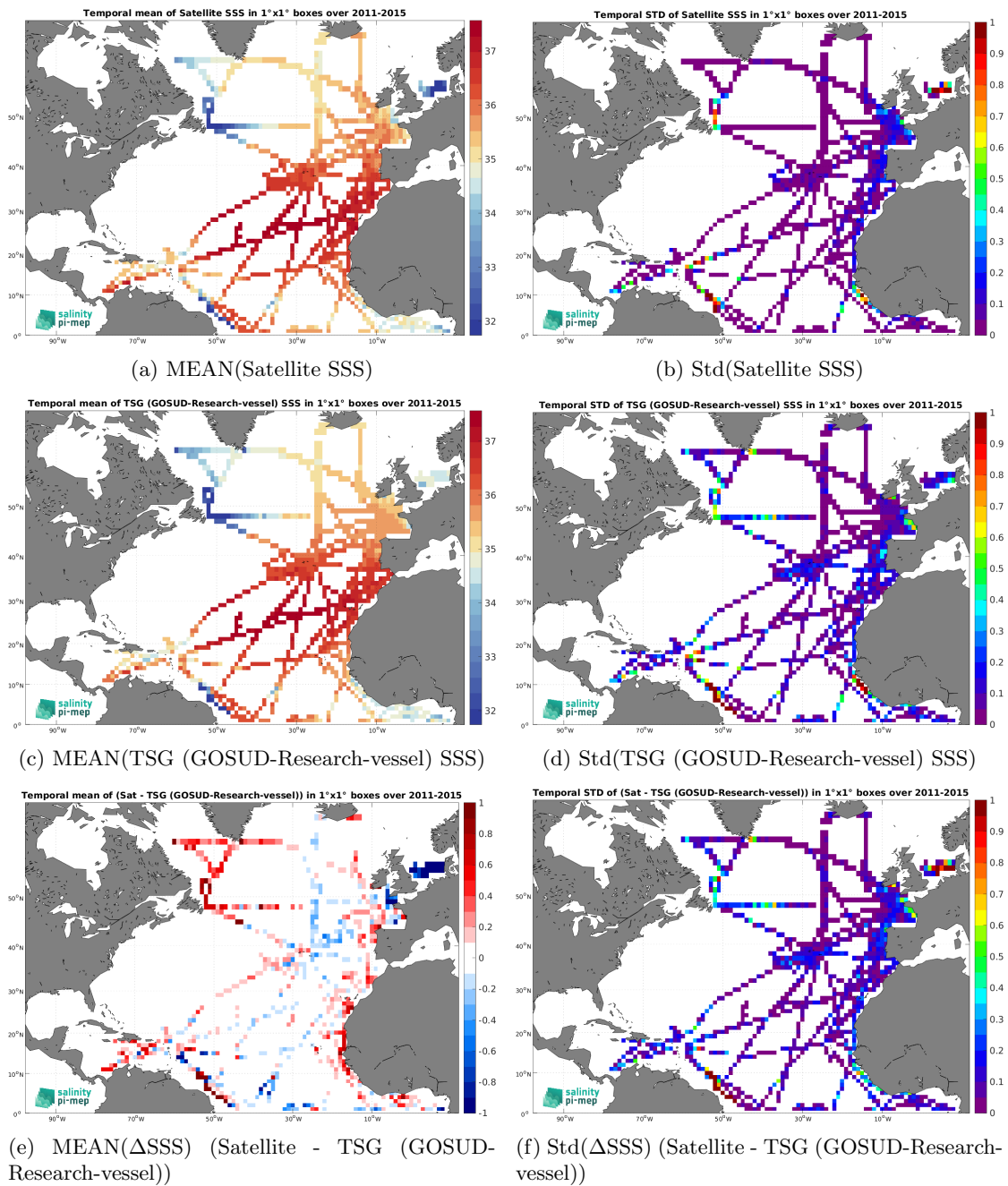
Figure 7: Temporal mean (left) and Std (right) of SSS from Aquarius SSS L3 CAP v5 - Monthly (JPL) (top), TSG (GOSUD-Research-vessel) (middle), and of \Delta SSS (Satellite - TSG (GOSUD-Research-vessel)). Only match-up pairs are used to generate these maps.
