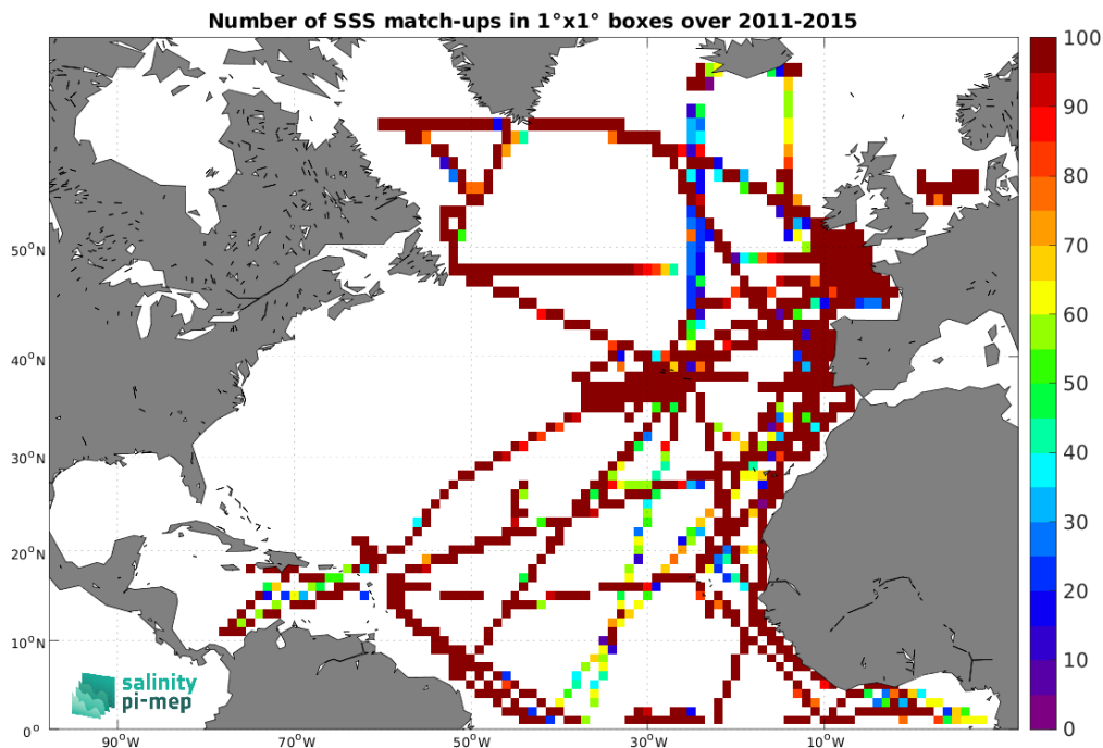
Figure 5: Number of SSS match-ups between TSG (GOSUD-Research-vessel) SSS and the Aquarius SSS L3 CAP v5 - Monthly (JPL) SSS product for the North Atlantic Ocean Pi-MEP region over 1^\circ \times 1^\circ boxes and for the full satellite product period.
