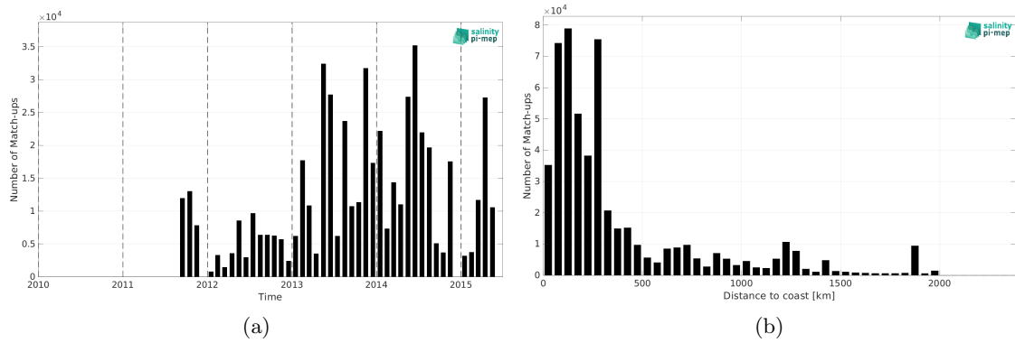
Figure 2: Number of match-ups between TSG (GOSUD-Research-vessel) and Aquarius SSS L3 CAP v5 - Monthly (JPL) SSS as a function of time (a) and as function of the distance to coast (b) over the North Atlantic Ocean Pi-MEP region and for the full satellite product period.
