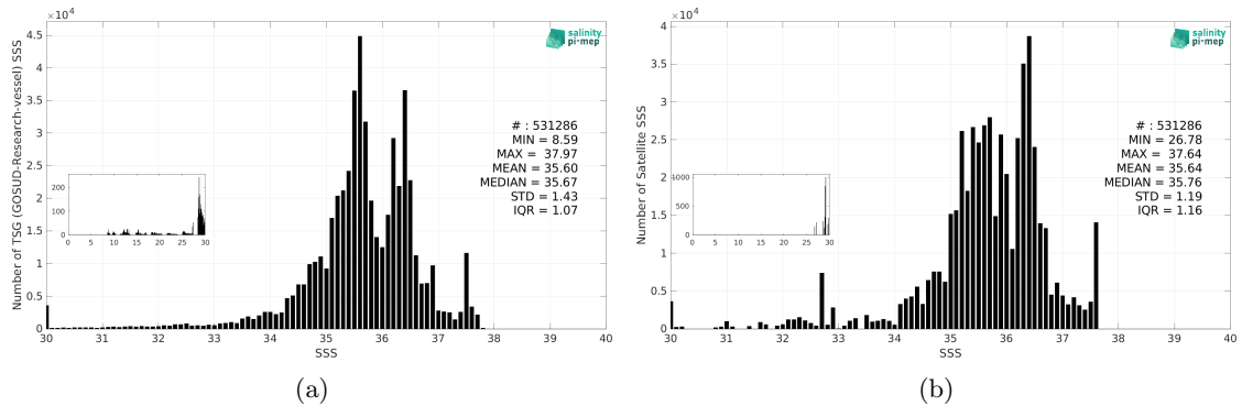
Figure 3: Histograms of SSS from TSG (GOSUD-Research-vessel) (a) and Aquarius SSS L3 CAP v5 - Monthly (JPL) (b) considering all match-up pairs per bins of 0.1 over the North Atlantic Ocean Pi-MEP region and for the full satellite product period.
