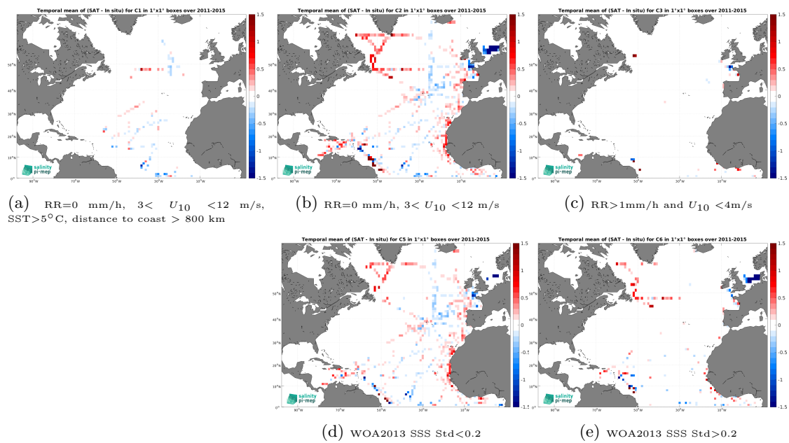
Figure 14: Temporal mean gridded over spatial boxes of size 1^\circ \times 1^\circ of \Delta\text{SSS} (Aquarius SSS L3 CAP v5 - Monthly (JPL) - TSG (GOSUD-Research-vessel)) for 5 different subdatasets corresponding to:RR=0 mm/h, 3 < U_{10} < 12 m/s, SST > 5°C, distance to coast > 800 km (a), RR=0 mm/h, 3 < U_{10} < 12 m/s (b), RR > 1mm/h and U_{10} < 4 m/s (c), WOA2013 SSS Std < 0.2 (d), WOA2013 SSS Std > 0.2 (e).
