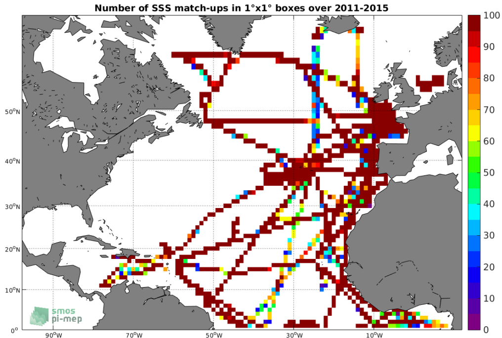
Figure 4: Number of SSS match-ups between TSG-GOSUD-Research-vessel SSS and the Aquarius-L3-JPL-V5-MONTHLY SSS product for the North Atlantic Ocean Pi-MEP region over 1^\circ \times 1^\circ boxes and for the full satellite product period.
