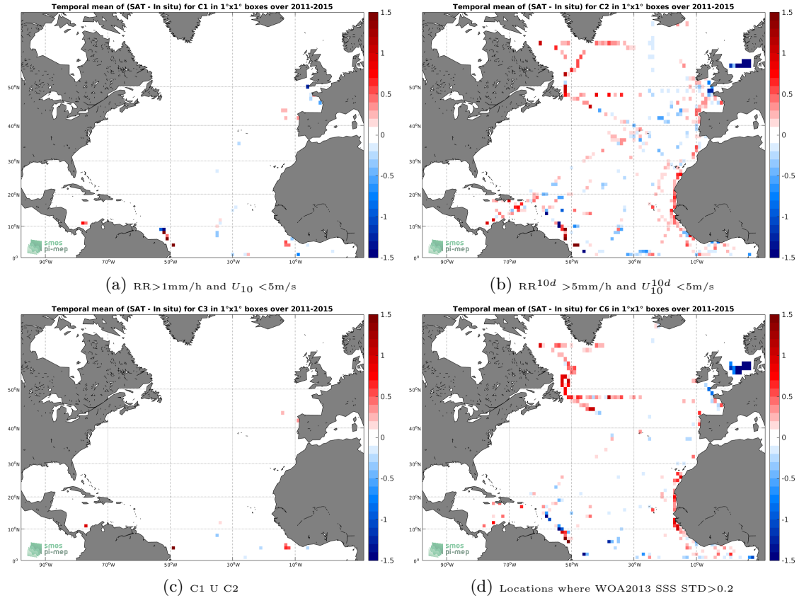
Figure 12: Temporal mean gridded over spatial boxes of size 1^\circ \times 1^\circ of \Delta SSS (Aquarius-L3-JPL-V5-MONTHLY - TSG-GOSUD-Research-vessel) for 4 different subdatasets corresponding to: RR > 1\text{mm/h} and U_{10} < 5\text{m/s} (a), RR^{10d} > 5\text{mm/h} and U_{10}^{10d} < 5\text{m/s} (b), C1 U C2 (c), Locations where WOA2013 SSS STD > 0.2 (d).
