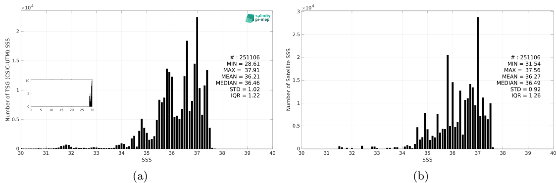
Figure 3: Histograms of SSS from TSG (CSIC-UTM) (a) and Aquarius SSS L3 CAP v5 - Monthly (JPL) (b) considering all match-up pairs per bins of 0.1 over the North Atlantic Ocean Pi-MEP region and for the full satellite product period.
