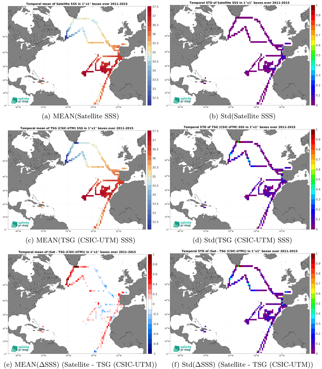
Figure 7: Temporal mean (left) and Std (right) of SSS from Aquarius SSS L3 CAP v5 - Monthly (JPL) (top), TSG (CSIC-UTM) (middle), and of \Delta SSS (Satellite - TSG (CSIC-UTM)). Only match-up pairs are used to generate these maps.
