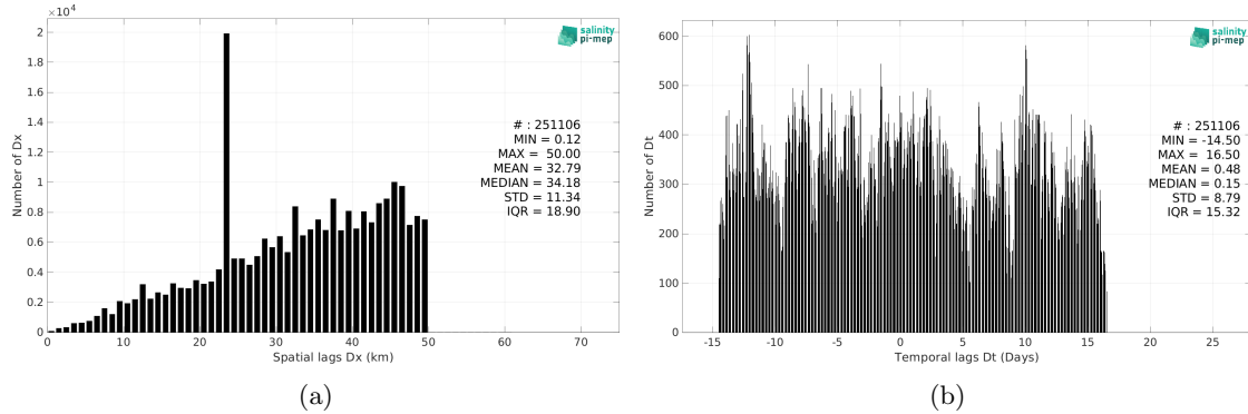
Figure 6: Histograms of the spatial (a) and temporal (b) lags between the location/time of the TSG (CSIC-UTM) measurement and the date of the corresponding Aquarius SSS L3 CAP v5 - Monthly (JPL) SSS pixel.
