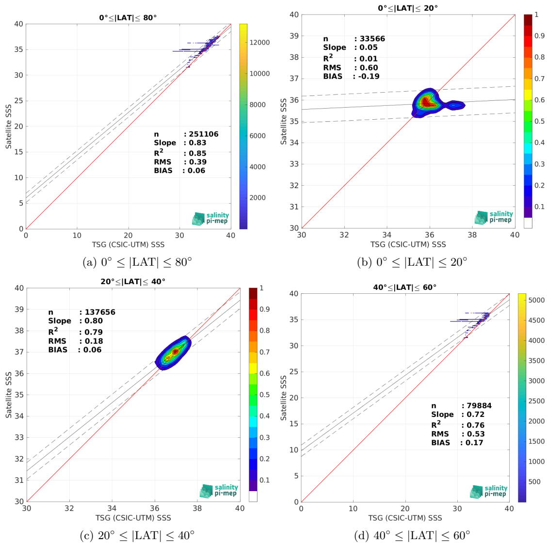
Figure 10: Contour maps of the concentration of Aquarius SSS L3 CAP v5 - Monthly (JPL) SSS (y-axis) versus TSG (CSIC-UTM) SSS (x-axis) at match-up pairs for different latitude bands. For each plot, the red line shows x=y . The black thin and dashed lines indicate a linear fit through the data cloud and the \pm 95\% confidence levels, respectively. The number match-up pairs n , the slope and R^2 coefficient of the linear fit, the root mean square (RMS) and the mean bias between satellite and in situ data are indicated for each latitude band in each plots.
