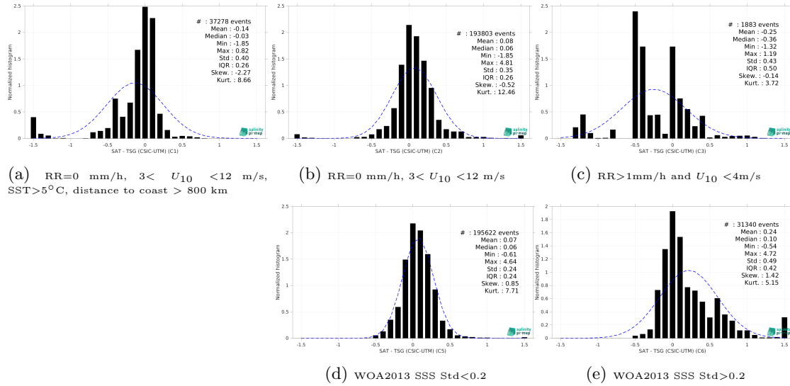
Figure 15: Normalized histogram of \Delta SSS (Aquarius SSS L3 CAP v5 - Monthly (JPL) - TSG (CSIC-UTM)) for 5 different subdatasets corresponding to: RR=0 mm/h, 3 < U_{10} < 12 m/s, SST>5°C, distance to coast > 800 km (a), RR=0 mm/h, 3 < U_{10} < 12 m/s (b), RR>1mm/h and U_{10} < 4 m/s (c), WOA2013 SSS Std<0.2 (d), WOA2013 SSS Std>0.2 (e).
