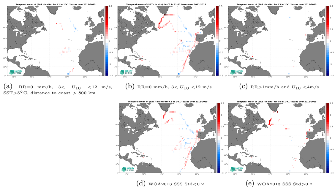
Figure 14: Temporal mean gridded over spatial boxes of size 1^\circ \times 1^\circ of \Delta\text{SSS} (Aquarius SSS L3 CAP v5 - Monthly (JPL) - TSG (CSIC-UTM)) for 5 different subdatasets corresponding to:RR=0 mm/h, 3 < U_{10} < 12 m/s, SST >5^\circ\text{C} , distance to coast > 800 km (a), RR=0 mm/h, 3 < U_{10} < 12 m/s (b), RR >1 mm/h and U_{10} < 4 m/s (c), WOA2013 SSS Std <0.2 (d), WOA2013 SSS Std >0.2 (e).
