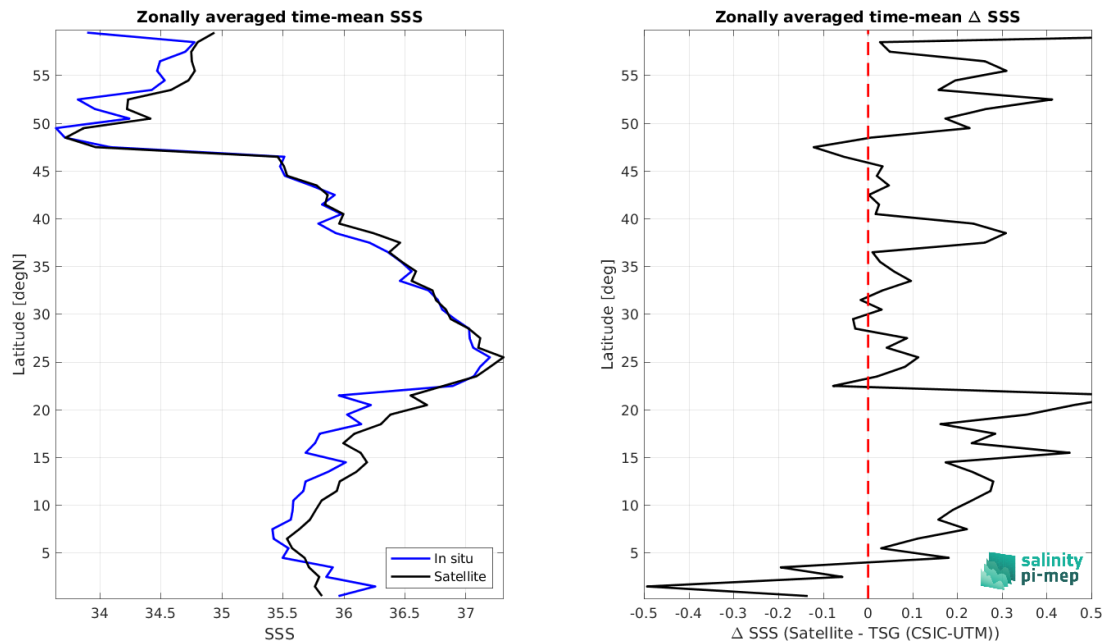
Figure 9: Left panel: Zonal mean SSS from Aquarius SSS L3 CAP v5 - Monthly (JPL) satellite product (black) and from TSG (CSIC-UTM) (blue). Right panel: Zonal mean of \Delta SSS (Satellite - TSG (CSIC-UTM)) for all the collected Pi-MEP match-up pairs estimated over the full satellite product period.
