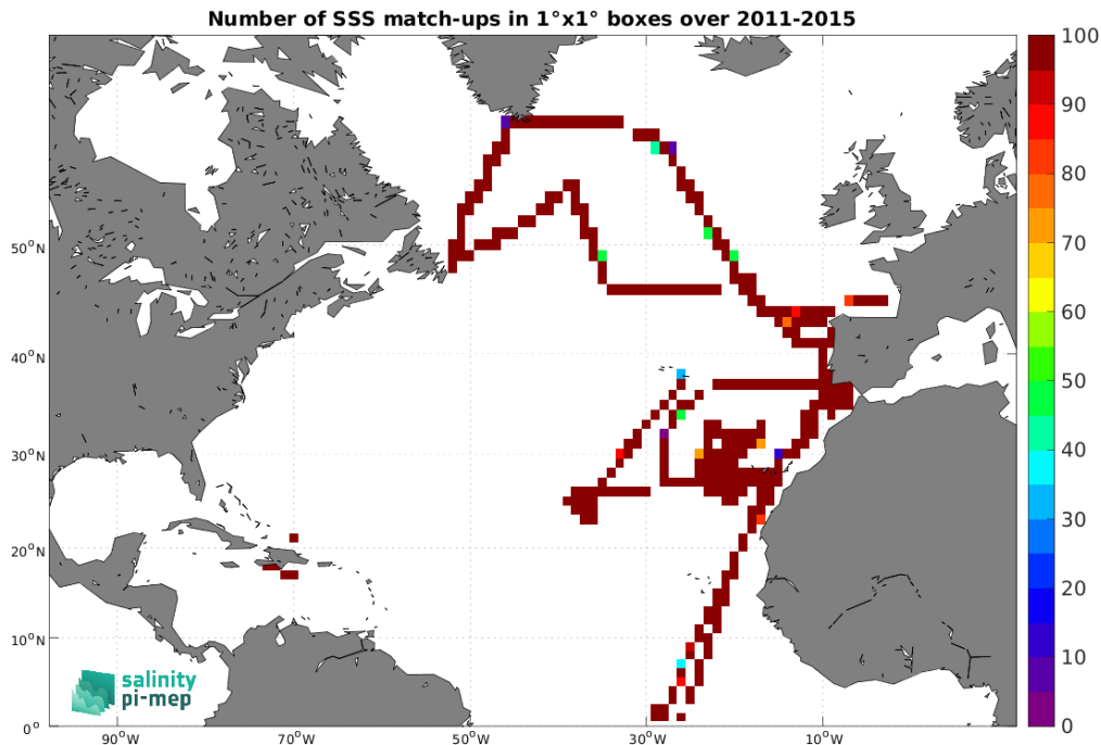
Figure 5: Number of SSS match-ups between TSG (CSIC-UTM) SSS and the Aquarius SSS L3 CAP v5 - Monthly (JPL) SSS product for the North Atlantic Ocean Pi-MEP region over 1^\circ \times 1^\circ boxes and for the full satellite product period.
