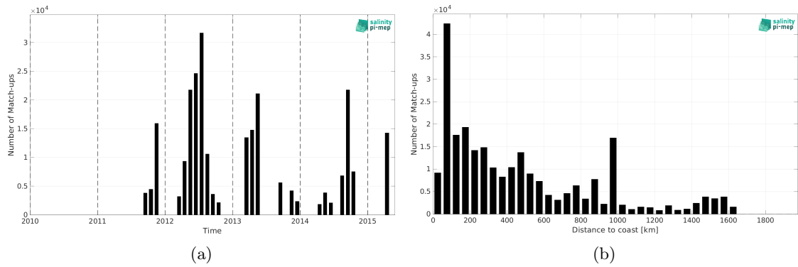
Figure 2: Number of match-ups between TSG (CSIC-UTM) and Aquarius SSS L3 CAP v5 - Monthly (JPL) SSS as a function of time (a) and as function of the distance to coast (b) over the North Atlantic Ocean Pi-MEP region and for the full satellite product period.
