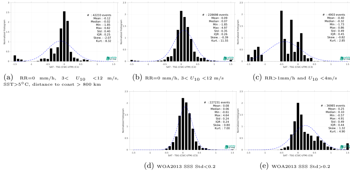
Figure 13: Normalized histogram of \Delta SSS (Aquarius SSS L3 CAP v5 - Monthly (JPL) - TSG (CSIC-UTM)) for 5 different subdatasets corresponding to: RR=0 mm/h, 3 < U_{10} < 12 m/s, SST > 5°C, distance to coast > 800 km (a), RR=0 mm/h, 3 < U_{10} < 12 m/s (b), RR > 1mm/h and U_{10} < 4 m/s (c), WOA2013 SSS Std < 0.2 (d), WOA2013 SSS Std > 0.2 (e).
