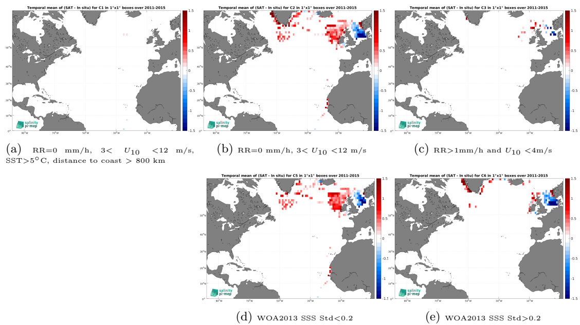
Figure 14: Temporal mean gridded over spatial boxes of size 1^\circ \times 1^\circ of \Delta\text{SSS} (Aquarius SSS L3 CAP v5 - Monthly (JPL) - ICES) for 5 different subdatasets corresponding to: RR=0 mm/h, 3 < U_{10} < 12 m/s, SST > 5^\circ\text{C} , distance to coast > 800 km (a), RR=0 mm/h, 3 < U_{10} < 12 m/s (b), RR > 1 mm/h and U_{10} < 4 m/s (c), WOA2013 SSS Std < 0.2 (d), WOA2013 SSS Std > 0.2 (e).
