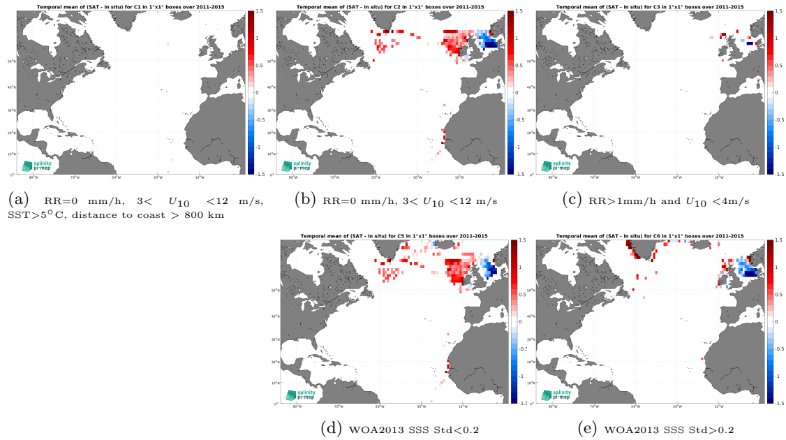
Figure 12: Temporal mean gridded over spatial boxes of size 1^\circ \times 1^\circ of \Delta\text{SSS} (Aquarius SSS L3 CAP v5 - Monthly (JPL) - ICES) for 5 different subdatasets corresponding to:RR=0 mm/h, 3 < U_{10} < 12 m/s, SST >5^\circ\text{C} , distance to coast > 800 km (a), RR=0 mm/h, 3 < U_{10} < 12 m/s (b), RR >1 mm/h and U_{10} < 4 m/s (c), WOA2013 SSS Std <0.2 (d), WOA2013 SSS Std >0.2 (e).
