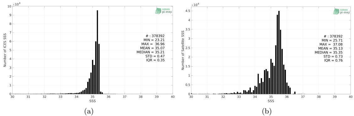
Figure 2: Histograms of SSS from ICES (a) and Aquarius SSS L3 CAP v5 - Monthly (JPL) (b) considering all match-up pairs per bins of 0.1 over the North Atlantic Ocean Pi-MEP region and for the full satellite product period.
