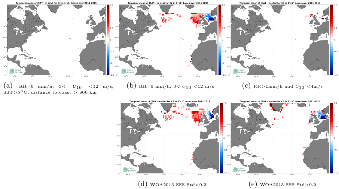
Figure 12: Temporal mean gridded over spatial boxes of size 1^\circ \times 1^\circ of \Delta SSS (Aquarius SSS L3 CAP v5 - Monthly (JPL) - ICES) for 5 different subdatasets corresponding to:RR=0 mm/h, 3 < U_{10} < 12 m/s, SST >5^\circ\text{C} , distance to coast > 800 km (a), RR=0 mm/h, 3 < U_{10} < 12 m/s (b), RR >1 mm/h and U_{10} < 4 m/s (c), WOA2013 SSS Std <0.2 (d), WOA2013 SSS Std >0.2 (e).
