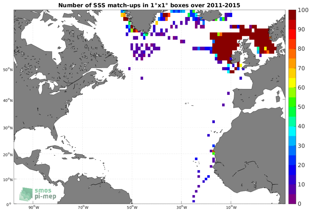
Figure 4: Number of SSS match-ups between ICES SSS and the Aquarius SSS L3 CAP v5 - Monthly (JPL) SSS product for the North Atlantic Ocean Pi-MEP region over 1^\circ \times 1^\circ boxes and for the full satellite product period.
