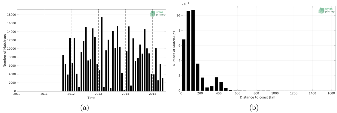
Figure 1: Number of match-ups between ICES and Aquarius SSS L3 CAP v5 - Monthly (JPL) SSS as a function of time (a) and as function of the distance to coast (b) over the North Atlantic Ocean Pi-MEP region and for the full satellite product period.
