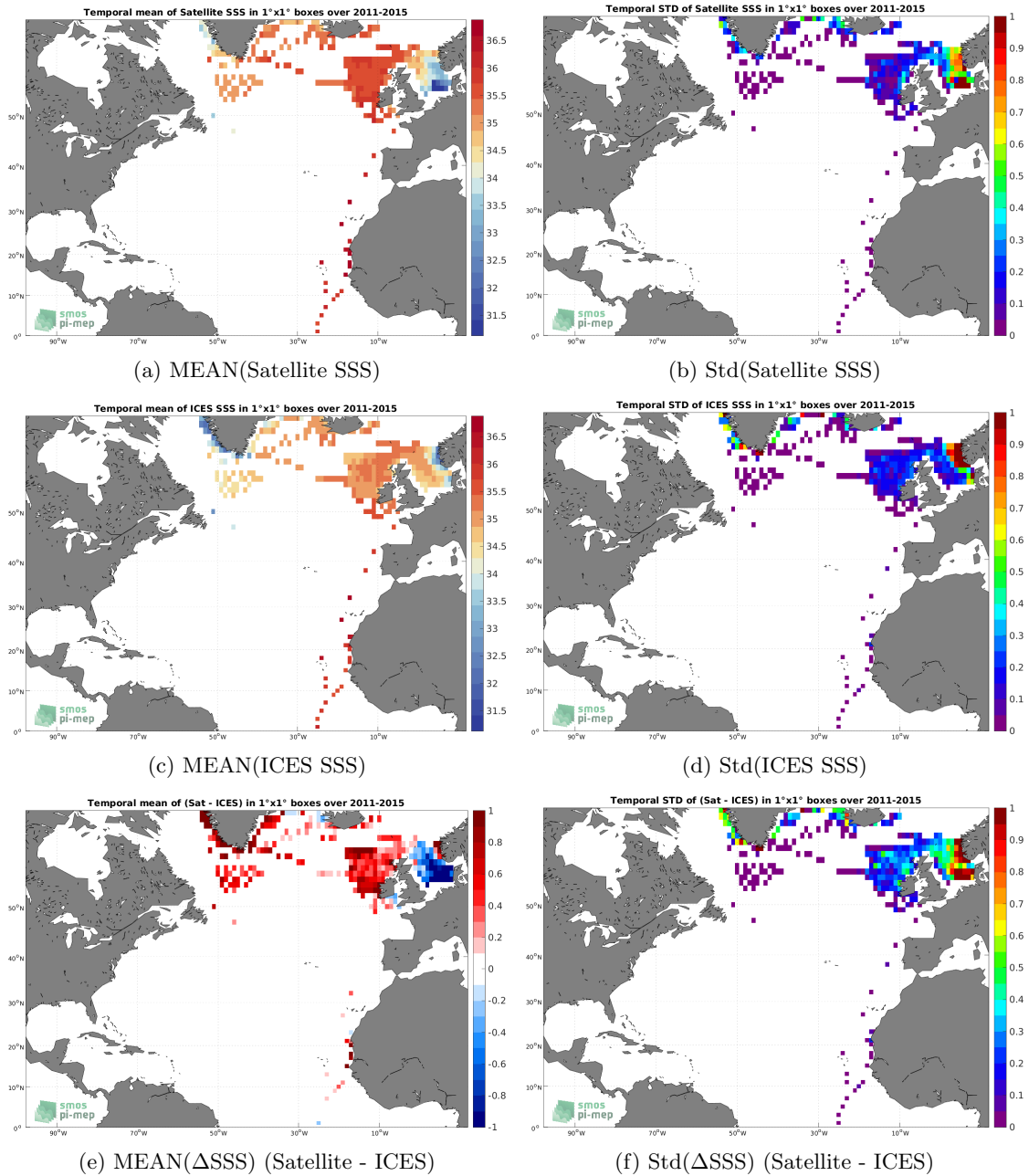
Figure 6: Temporal mean (left) and Std (right) of SSS from Aquarius SSS L3 CAP v5 - Monthly (JPL) (top), ICES (middle), and of \Delta SSS (Satellite - ICES). Only match-up pairs are used to generate these maps.
