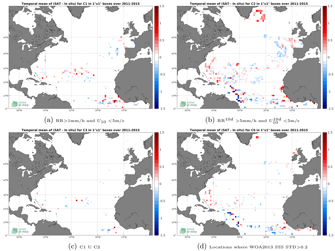
Figure 11: Temporal mean gridded over spatial boxes of size 1^\circ \times 1^\circ of \Delta SSS (Aquarius-L3-JPL-V5-MONTHLY - Surface drifters) for 4 different subdatasets corresponding to:RR>1mm/h and U_{10} < 5 m/s (a), RR^{10d} > 5 mm/h and U_{10}^{10d} < 5 m/s (b), C1 U C2 (c),Locations where WOA2013 SSS STD>0.2 (d).
