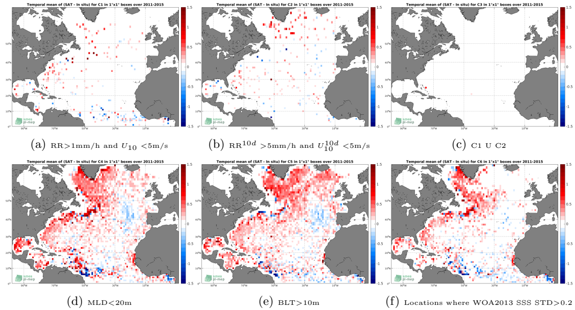
Figure 12: Temporal mean gridded over spatial boxes of size 1^\circ \times 1^\circ of \Delta\text{SSS} (Aquarius-L3-JPL-V5-MONTHLY - Argo) for 6 different subdatasets corresponding to: RR > 1\text{mm/h} and U_{10} < 5\text{m/s} (a), RR^{10d} > 5\text{mm/h} and U_{10}^{10d} < 5\text{m/s} (b), C1 U C2 (c), MLD < 20\text{m} (d), BLT > 10\text{m} (e), Locations where WOA2013 SSS STD > 0.2 (f).
