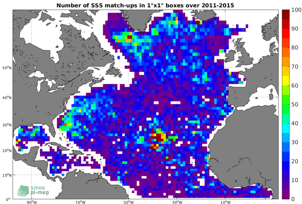
Figure 4: Number of SSS match-ups between Argo SSS and the Aquarius-L3-JPL-V5-MONTHLY SSS product for the North Atlantic Ocean Pi-MEP region over 1^\circ \times 1^\circ boxes and for the full satellite product period.
