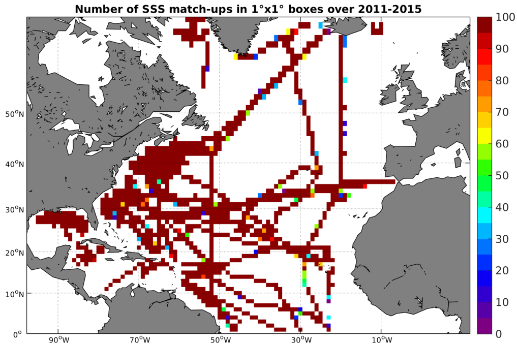
Figure 4: Number of SSS match-ups between TSG-SAMOS SSS and the Aquarius-L3-JPL-V4-7DAY-RUNNING SSS product for the North Atlantic Ocean Pi-MEP region over 1^\circ \times 1^\circ boxes and for the full satellite product period.
