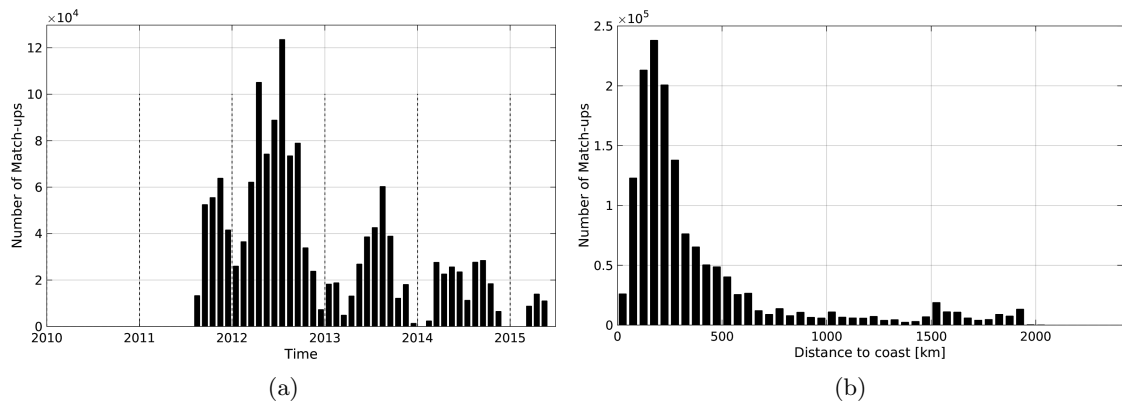
Figure 1: Number of match-ups between TSG-SAMOS and Aquarius-L3-JPL-V4-7DAY-RUNNING SSS as a function of time (a) and as function of the distance to coast (b) over the North Atlantic Ocean Pi-MEP region and for the full satellite product period.
