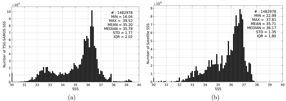
Figure 2: Histograms of SSS from TSG-SAMOS (a) and Aquarius-L3-JPL-V4-7DAY-RUNNING (b) considering all match-up pairs per bins of 0.1 over the North Atlantic Ocean Pi-MEP region and for the full satellite product period.
