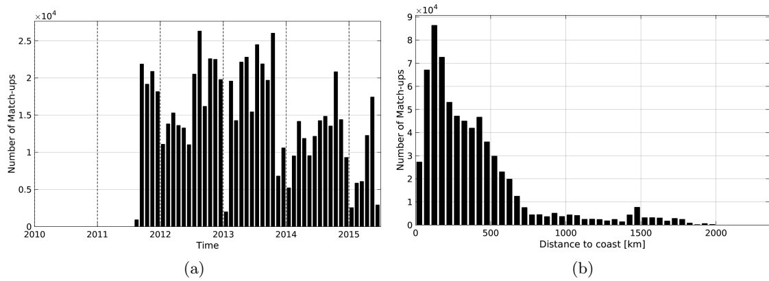
Figure 1: Number of match-ups between TSG-LEGOS-DM and Aquarius-L3-JPL-V4-7DAY-RUNNING SSS as a function of time (a) and as function of the distance to coast (b) over the North Atlantic Ocean Pi-MEP region and for the full satellite product period.
