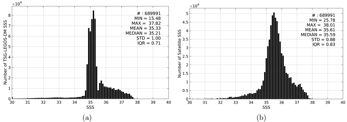
Figure 2: Histograms of SSS from TSG-LEGOS-DM (a) and Aquarius-L3-JPL-V4-7DAY-RUNNING (b) considering all match-up pairs per bins of 0.1 over the North Atlantic Ocean Pi-MEP region and for the full satellite product period.
