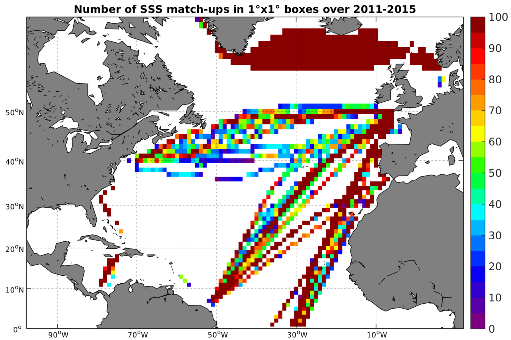
Figure 4: Number of SSS match-ups between TSG-LEGOS-DM SSS and the Aquarius-L3-JPL-V4-7DAY-RUNNING SSS product for the North Atlantic Ocean Pi-MEP region over 1^\circ \times 1^\circ boxes and for the full satellite product period.
