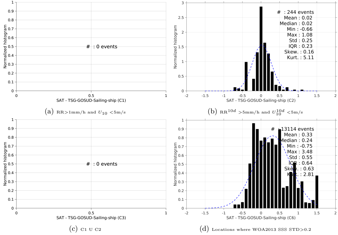
Figure 13: Normalized histogram of \Delta SSS (Aquarius-L3-JPL-V4-7DAY-RUNNING - TSG-GOSUD-Sailing-ship) for 6 different subdatasets corresponding to: RR > 1\text{mm/h} and U_{10} < 5\text{m/s} (a), RR^{10d} > 5\text{mm/h} and U_{10}^{10d} < 5\text{m/s} (b), C1 \cup C2 (c), Locations where WOA2013 SSS STD > 0.2 (d).
