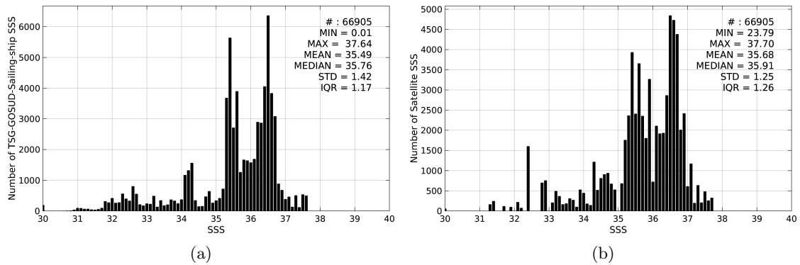
Figure 2: Histograms of SSS from TSG-GOSUD-Sailing-ship (a) and Aquarius-L3-JPL-V4-7DAY-RUNNING (b) considering all match-up pairs per bins of 0.1 over the North Atlantic Ocean Pi-MEP region and for the full satellite product period.
