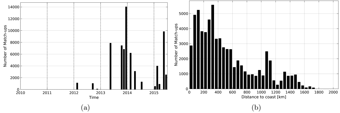
Figure 1: Number of match-ups between TSG-GOSUD-Sailing-ship and Aquarius-L3-JPL-V4-7DAY-RUNNING SSS as a function of time (a) and as function of the distance to coast (b) over the North Atlantic Ocean Pi-MEP region and for the full satellite product period.
