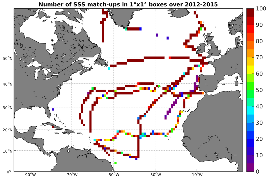
Figure 4: Number of SSS match-ups between TSG-GOSUD-Sailing-ship SSS and the Aquarius-L3-JPL-V4-7DAY-RUNNING SSS product for the North Atlantic Ocean Pi-MEP region over 1^\circ \times 1^\circ boxes and for the full satellite product period.
