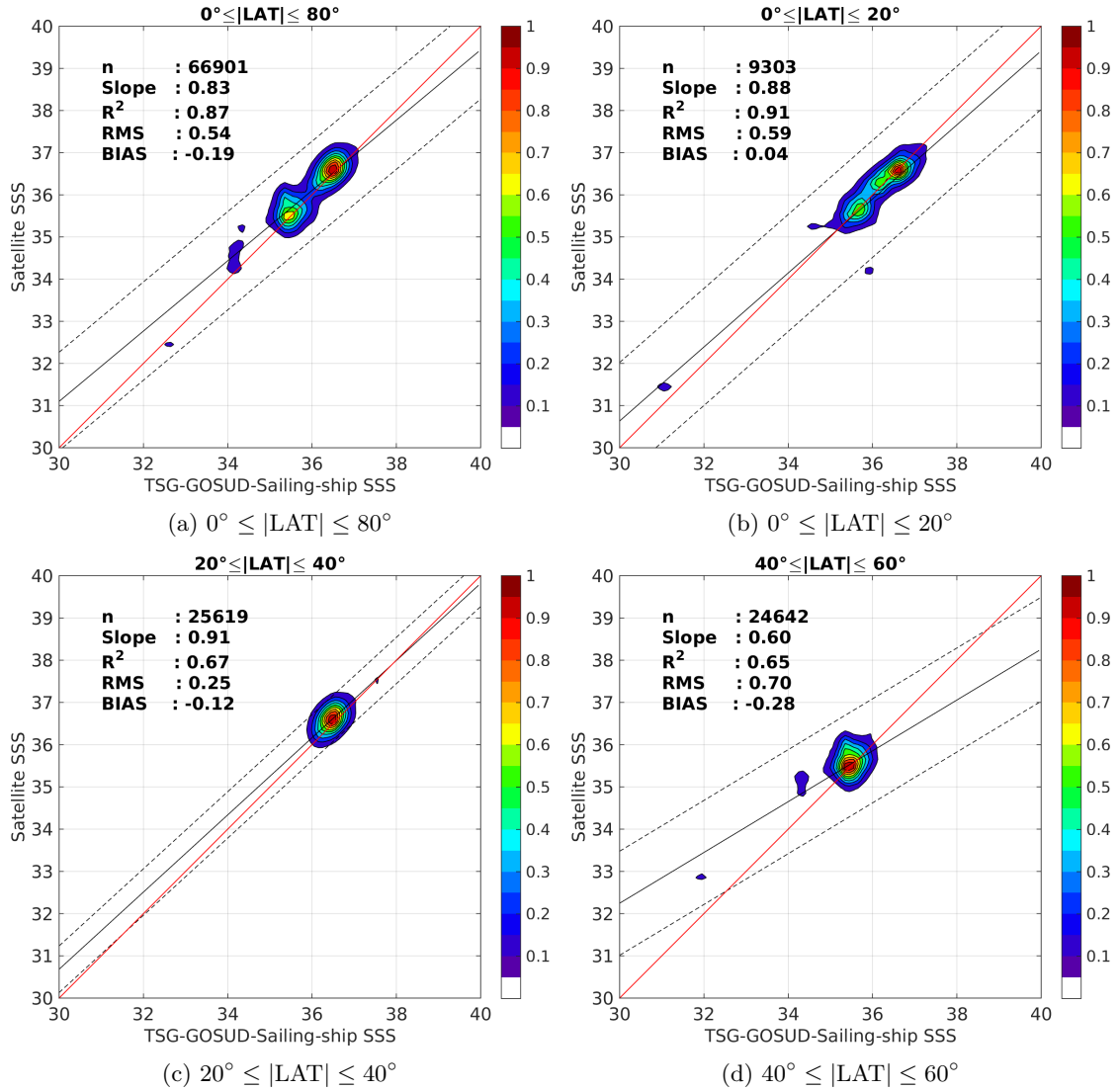
Figure 9: Contour maps of the concentration of Aquarius-L3-JPL-V4-7DAY-RUNNING SSS (y-axis) versus TSG-GOSUD-Sailing-ship SSS (x-axis) at match-up pairs for different latitude bands. For each plot, the red line shows x=y . The black thin and dashed lines indicate a linear fit through the data cloud and the \pm 95\% confidence levels, respectively. The number match-up pairs n , the slope and R^2 coefficient of the linear fit, the root mean square (RMS) and the mean bias between satellite and in situ data are indicated for each latitude band in each plots.
