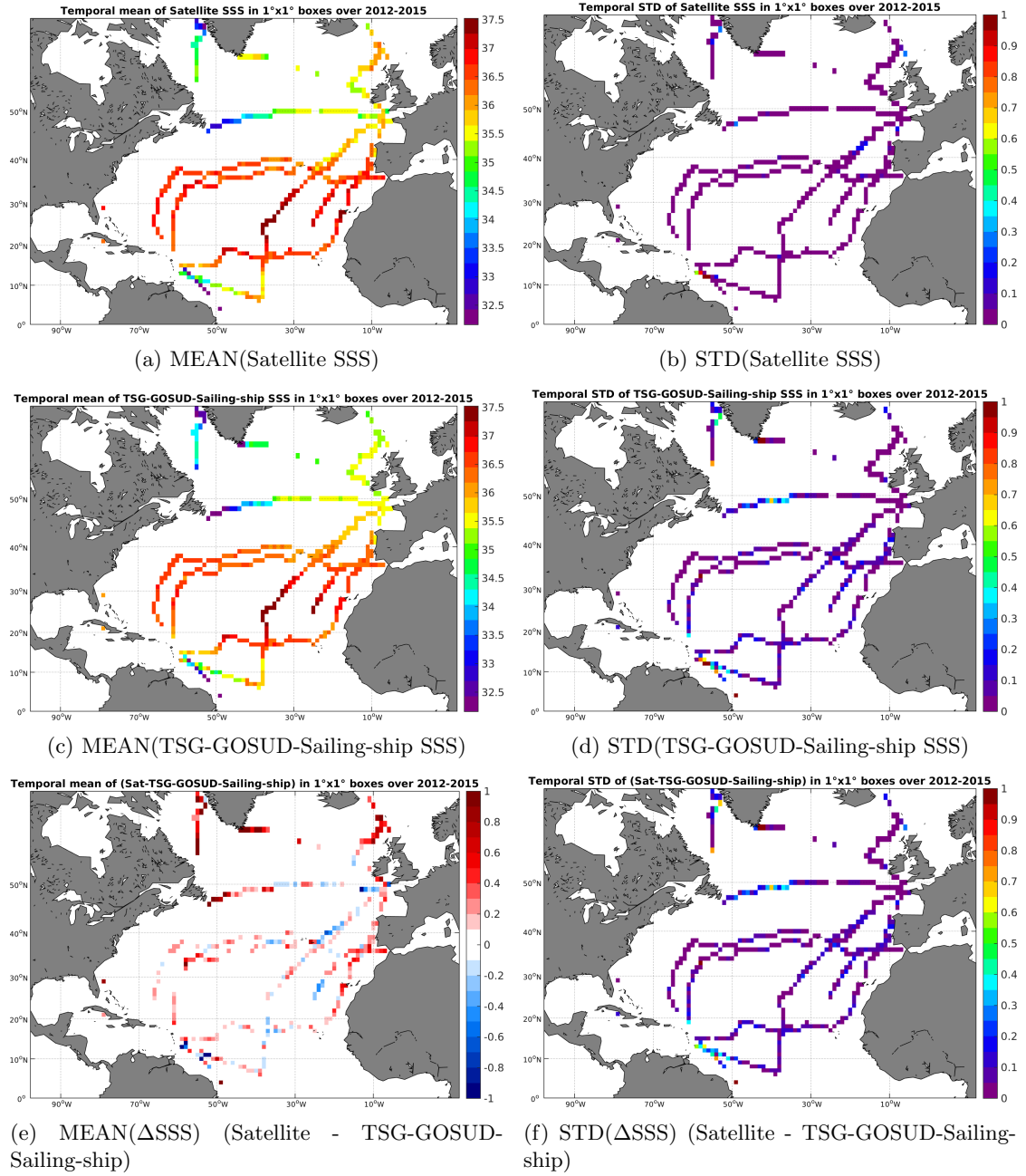
Figure 6: Temporal mean (left) and STD (right) of SSS from Aquarius-L3-JPL-V4-7DAY-RUNNING (top), TSG-GOSUD-Sailing-ship (middle), and of \Delta SSS (Satellite - TSG-GOSUD-Sailing-ship). Only match-up pairs are used to generate these maps.
