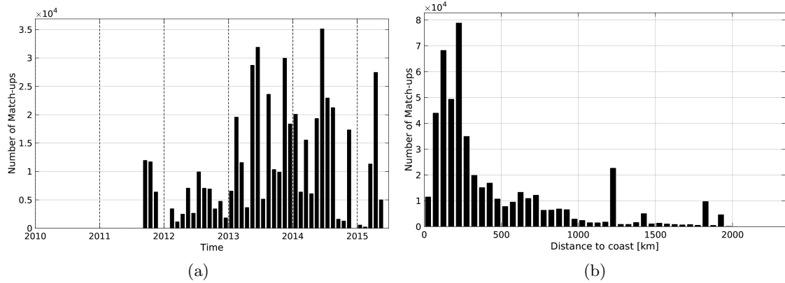
Figure 1: Number of match-ups between TSG-GOSUD-Research-vessel and Aquarius-L3-JPL-V4-7DAY-RUNNING SSS as a function of time (a) and as function of the distance to coast (b) over the North Atlantic Ocean Pi-MEP region and for the full satellite product period.
