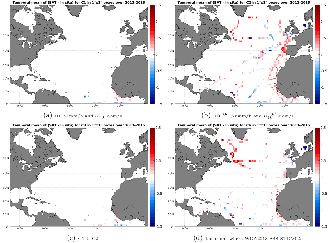
Figure 12: Temporal mean gridded over spatial boxes of size 1^\circ \times 1^\circ of \Delta SSS (Aquarius-L3-JPL-V4-7DAY-RUNNING - TSG-GOSUD-Research-vessel) for 4 different subdatasets corresponding to: RR > 1mm/h and U_{10} < 5 m/s (a), RR^{10d} > 5 mm/h and U_{10}^{10d} < 5 m/s (b), C1 U C2 (c), Locations where WOA2013 SSS STD > 0.2 (d).
