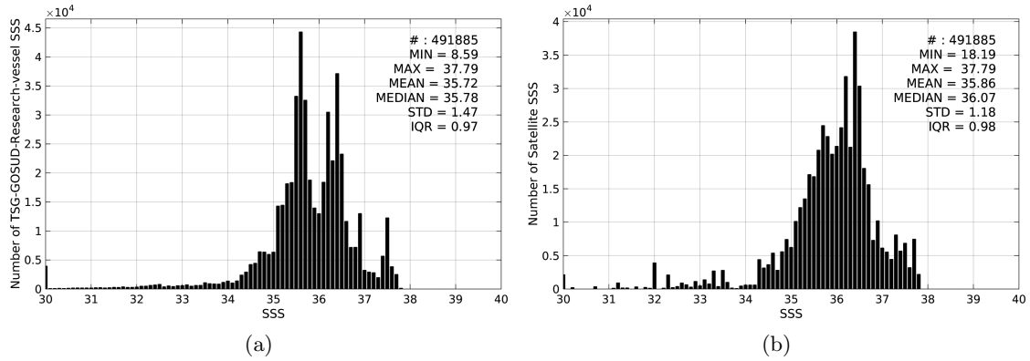
Figure 2: Histograms of SSS from TSG-GOSUD-Research-vessel (a) and Aquarius-L3-JPL-V4-7DAY-RUNNING (b) considering all match-up pairs per bins of 0.1 over the North Atlantic Ocean Pi-MEP region and for the full satellite product period.
