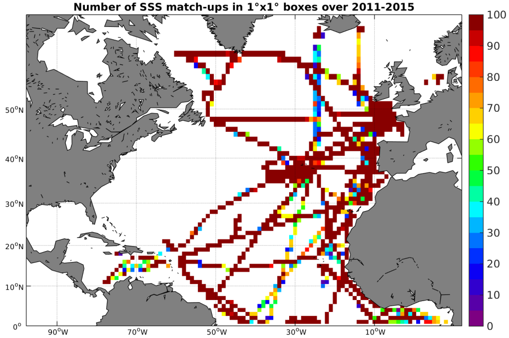
Figure 4: Number of SSS match-ups between TSG-GOSUD-Research-vessel SSS and the Aquarius-L3-JPL-V4-7DAY-RUNNING SSS product for the North Atlantic Ocean Pi-MEP region over 1^\circ \times 1^\circ boxes and for the full satellite product period.
