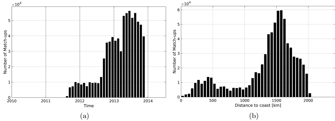
Figure 1: Number of match-ups between Surface drifters and Aquarius-L3-JPL-V4-7DAY-RUNNING SSS as a function of time (a) and as function of the distance to coast (b) over the North Atlantic Ocean Pi-MEP region and for the full satellite product period.
