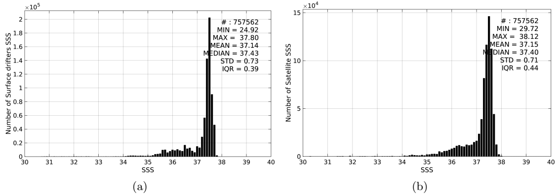
Figure 2: Histograms of SSS from Surface drifters (a) and Aquarius-L3-JPL-V4-7DAY-RUNNING (b) considering all match-up pairs per bins of 0.1 over the North Atlantic Ocean Pi-MEP region and for the full satellite product period.
