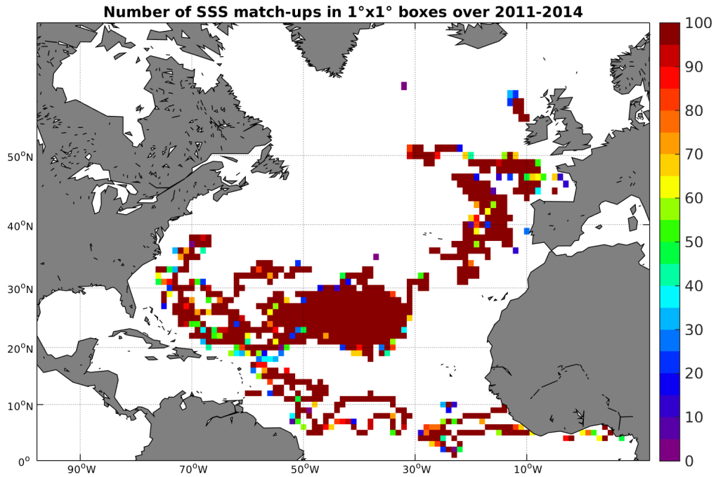
Figure 3: Number of SSS match-ups between Surface drifters SSS and the Aquarius-L3-JPL-V4-7DAY-RUNNING SSS product for the North Atlantic Ocean Pi-MEP region over 1°x1° boxes and for the full satellite product period.
