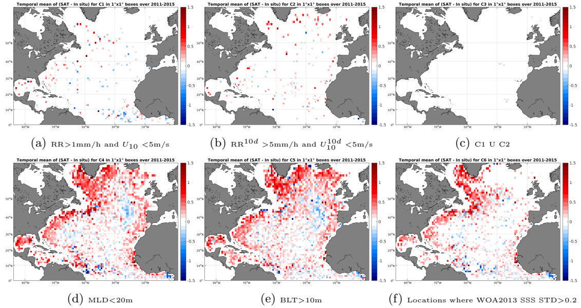
Figure 12: Temporal mean gridded over spatial boxes of size 1^\circ \times 1^\circ of \Delta SSS (Aquarius-L3-JPL-V4-7DAY-RUNNING - Argo) for 6 different subdatasets corresponding to: RR > 1mm/h and U_{10} < 5 m/s (a), RR^{10d} > 5 mm/h and U_{10}^{10d} < 5 m/s (b), C1 U C2 (c), MLD < 20m (d), BLT > 10m (e), Locations where WOA2013 SSS STD > 0.2 (f).
