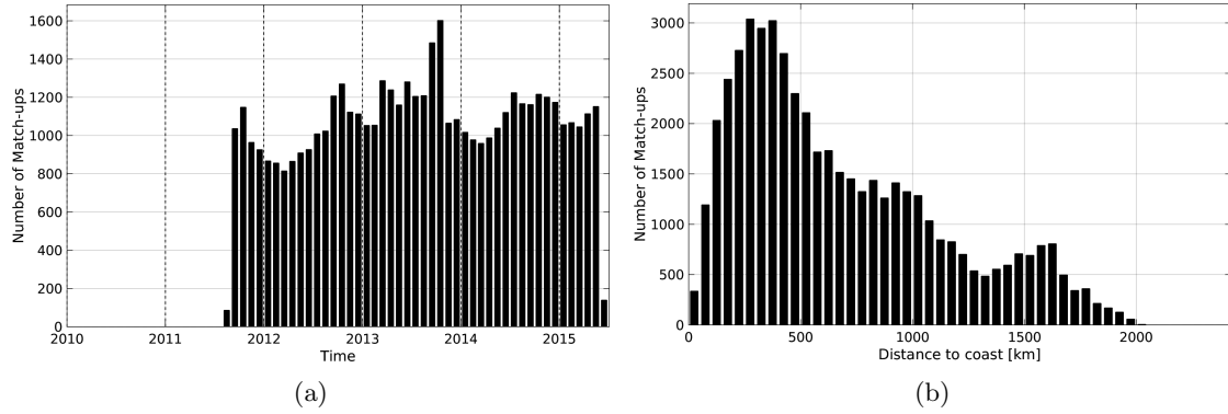
Figure 1: Number of match-ups between Argo and Aquarius-L3-JPL-V4-7DAY-RUNNING SSS as a function of time (a) and as function of the distance to coast (b) over the North Atlantic Ocean Pi-MEP region and for the full satellite product period.
