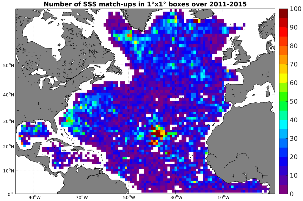
Figure 4: Number of SSS match-ups between Argo SSS and the Aquarius-L3-JPL-V4-7DAY-RUNNING SSS product for the North Atlantic Ocean Pi-MEP region over 1^\circ \times 1^\circ boxes and for the full satellite product period.
