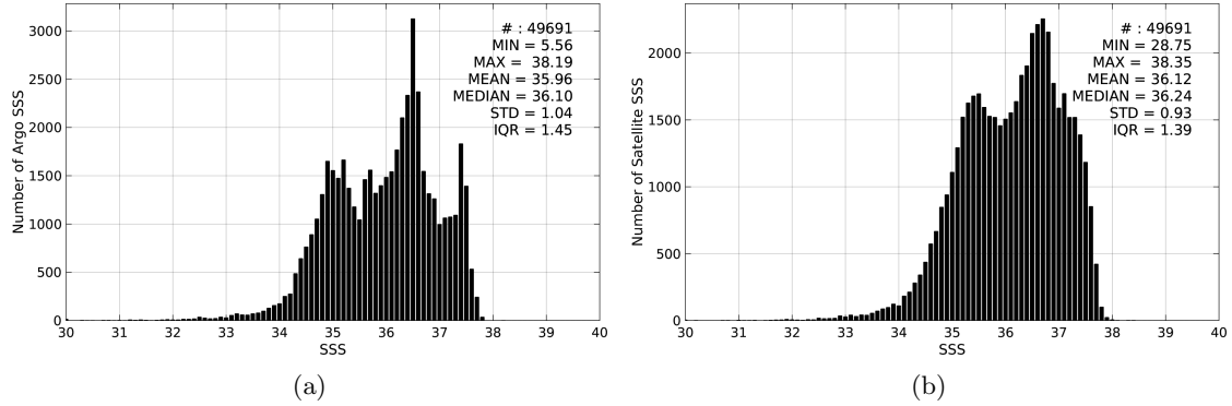
Figure 2: Histograms of SSS from Argo (a) and Aquarius-L3-JPL-V4-7DAY-RUNNING (b) considering all match-up pairs per bins of 0.1 over the North Atlantic Ocean Pi-MEP region and for the full satellite product period.
