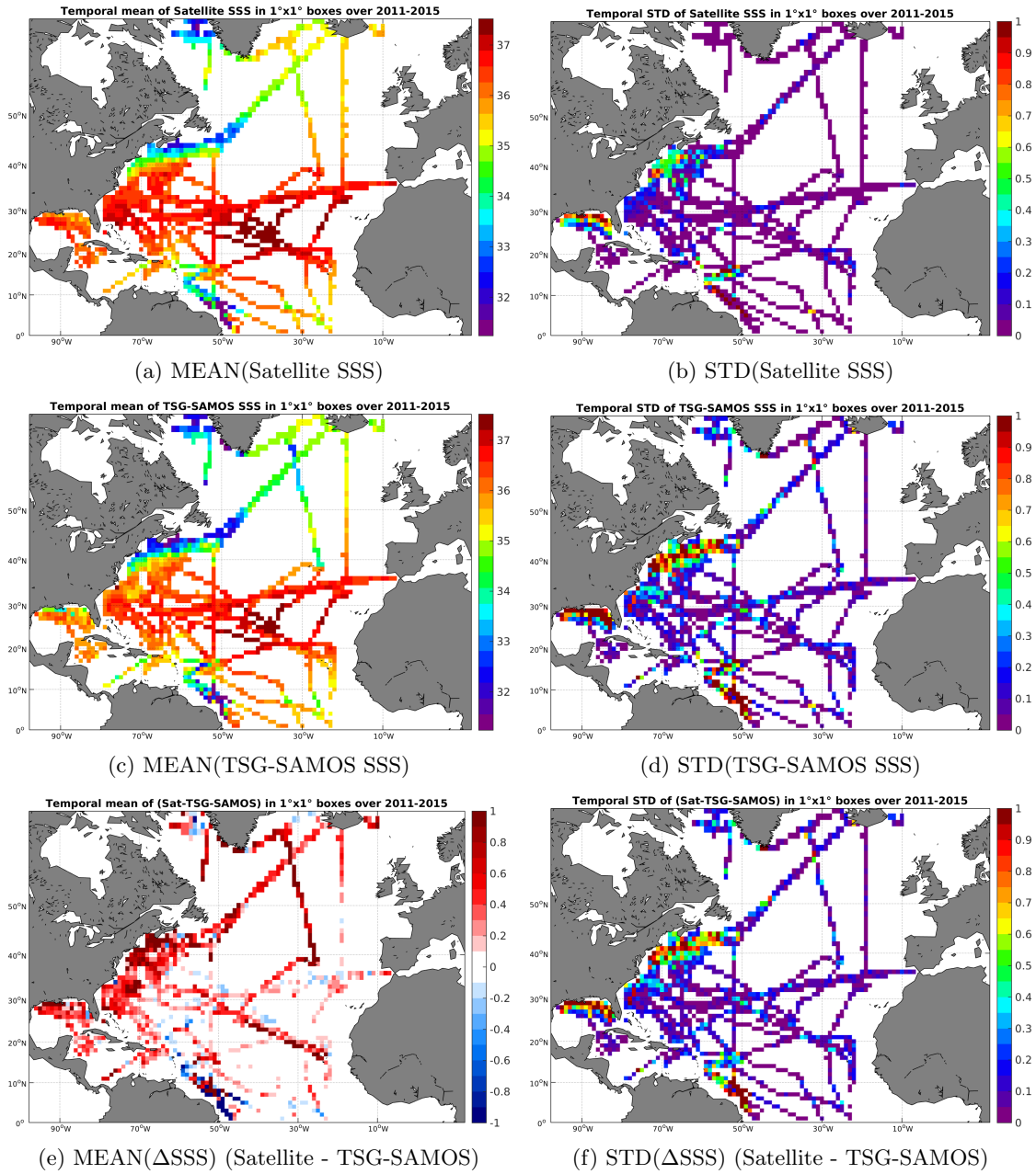
Figure 6: Temporal mean (left) and STD (right) of SSS from Aquarius-L3-JPL-V4-MONTHLY (top), TSG-SAMOS (middle), and of \Delta SSS (Satellite - TSG-SAMOS). Only match-up pairs are used to generate these maps.
