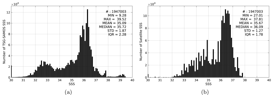
Figure 2: Histograms of SSS from TSG-SAMOS (a) and Aquarius-L3-JPL-V4-MONTHLY (b) considering all match-up pairs per bins of 0.1 over the North Atlantic Ocean Pi-MEP region and for the full satellite product period.
