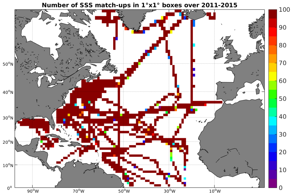
Figure 4: Number of SSS match-ups between TSG-SAMOS SSS and the Aquarius-L3-JPL-V4-MONTHLY SSS product for the North Atlantic Ocean Pi-MEP region over 1^\circ \times 1^\circ boxes and for the full satellite product period.
