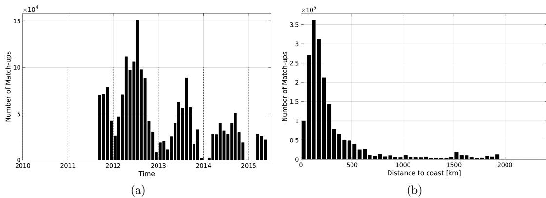
Figure 1: Number of match-ups between TSG-SAMOS and Aquarius-L3-JPL-V4-MONTHLY SSS as a function of time (a) and as function of the distance to coast (b) over the North Atlantic Ocean Pi-MEP region and for the full satellite product period.
