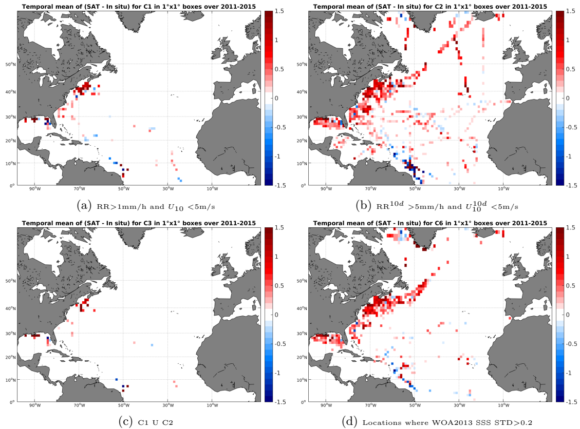
Figure 12: Temporal mean gridded over spatial boxes of size 1^\circ \times 1^\circ of \Delta SSS (Aquarius-L3-JPL-V4-MONTHLY - TSG-SAMOS) for 4 different subdatasets corresponding to: RR > 1 mm/h and U_{10} < 5 m/s (a), RR 10d > 5 mm/h and U_{10}^{10d} < 5 m/s (b), C1 U C2 (c), Locations where WOA2013 SSS STD > 0.2 (d).
