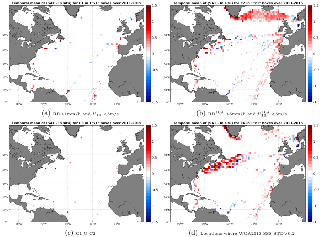
Figure 12: Temporal mean gridded over spatial boxes of size 1^\circ \times 1^\circ of \Delta SSS (Aquarius-L3-JPL-V4-MONTHLY - TSG-LEGOS-DM) for 4 different subdatasets corresponding to:RR>1mm/h and U_{10} < 5\text{m/s} (a), RR^{10d} > 5\text{mm/h} and U_{10}^{10d} < 5\text{m/s} (b), C1 U C2 (c),Locations where WOA2013 SSS STD>0.2 (d).
