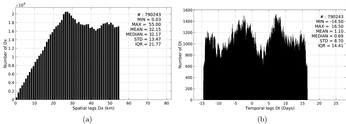
Figure 5: Histograms of the spatial (a) and temporal (b) lags between the time of the TSG-LEGOS-DM measurements and the date of the corresponding Aquarius-L3-JPL-V4-MONTHLY SSS product.
