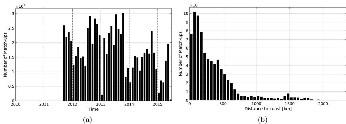
Figure 1: Number of match-ups between TSG-LEGOS-DM and Aquarius-L3-JPL-V4-MONTHLY SSS as a function of time (a) and as function of the distance to coast (b) over the North Atlantic Ocean Pi-MEP region and for the full satellite product period.
