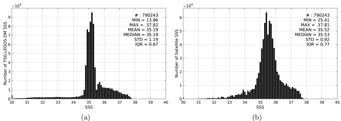
Figure 2: Histograms of SSS from TSG-LEGOS-DM (a) and Aquarius-L3-JPL-V4-MONTHLY (b) considering all match-up pairs per bins of 0.1 over the North Atlantic Ocean Pi-MEP region and for the full satellite product period.
