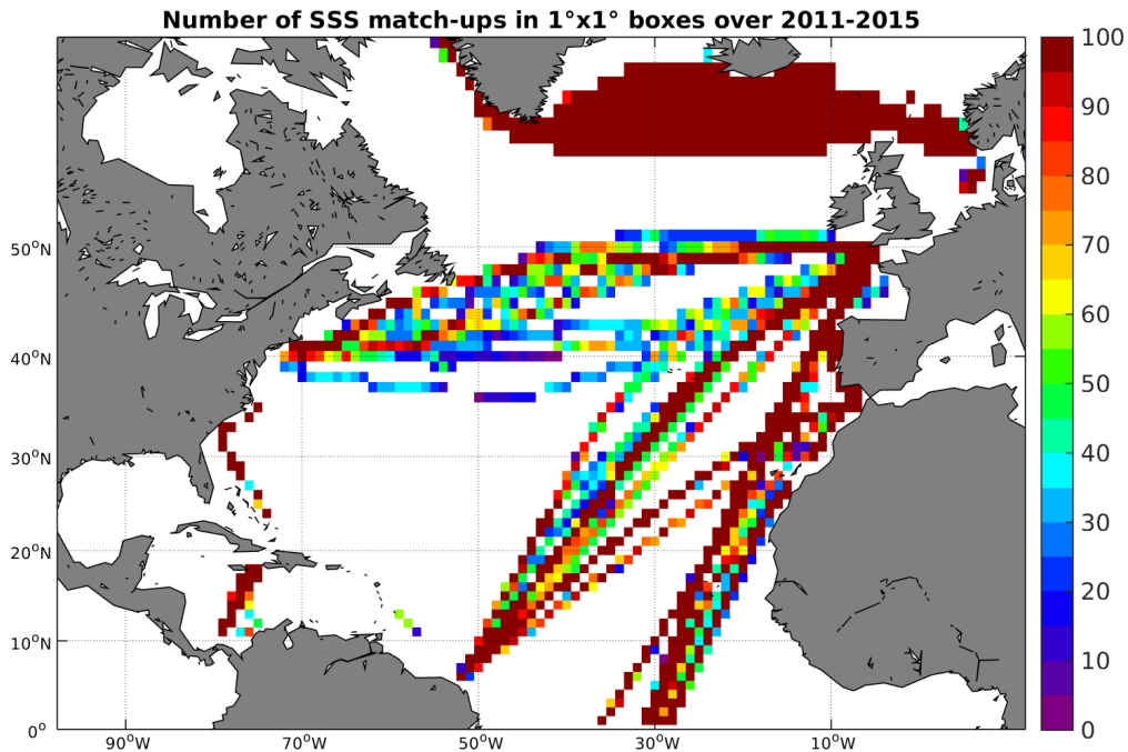
Figure 4: Number of SSS match-ups between TSG-LEGOS-DM SSS and the Aquarius-L3-JPL-V4-MONTHLY SSS product for the North Atlantic Ocean Pi-MEP region over 1^\circ \times 1^\circ boxes and for the full satellite product period.
