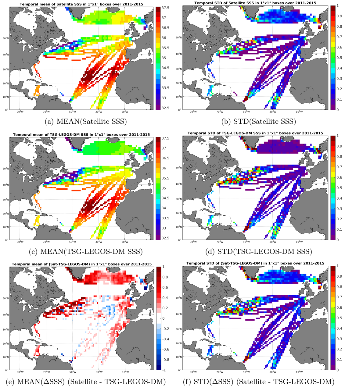
Figure 6: Temporal mean (left) and STD (right) of SSS from Aquarius-L3-JPL-V4-MONTHLY (top), TSG-LEGOS-DM (middle), and of \Delta SSS (Satellite - TSG-LEGOS-DM). Only match-up pairs are used to generate these maps.
