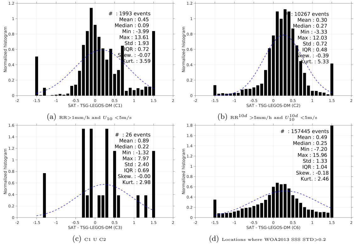
Figure 13: Normalized histogram of \Delta SSS (Aquarius-L3-JPL-V4-MONTHLY - TSG-LEGOS-DM) for 6 different subdatasets corresponding to: RR > 1mm/h and U_{10} < 5 m/s (a), RR^{10d} > 5 mm/h and U_{10}^{10d} < 5 m/s (b), C1 U C2 (c), Locations where WOA2013 SSS STD > 0.2 (d).
