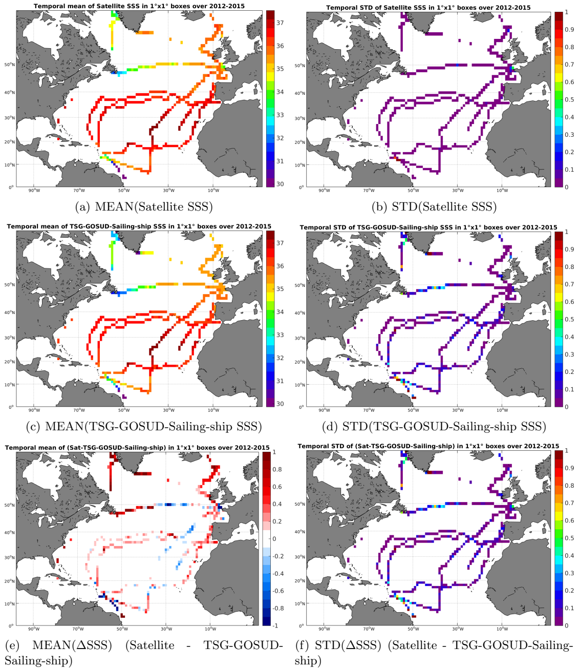
Figure 6: Temporal mean (left) and STD (right) of SSS from Aquarius-L3-JPL-V4-MONTHLY (top), TSG-GOSUD-Sailing-ship (middle), and of \Delta SSS (Satellite - TSG-GOSUD-Sailing-ship). Only match-up pairs are used to generate these maps.
