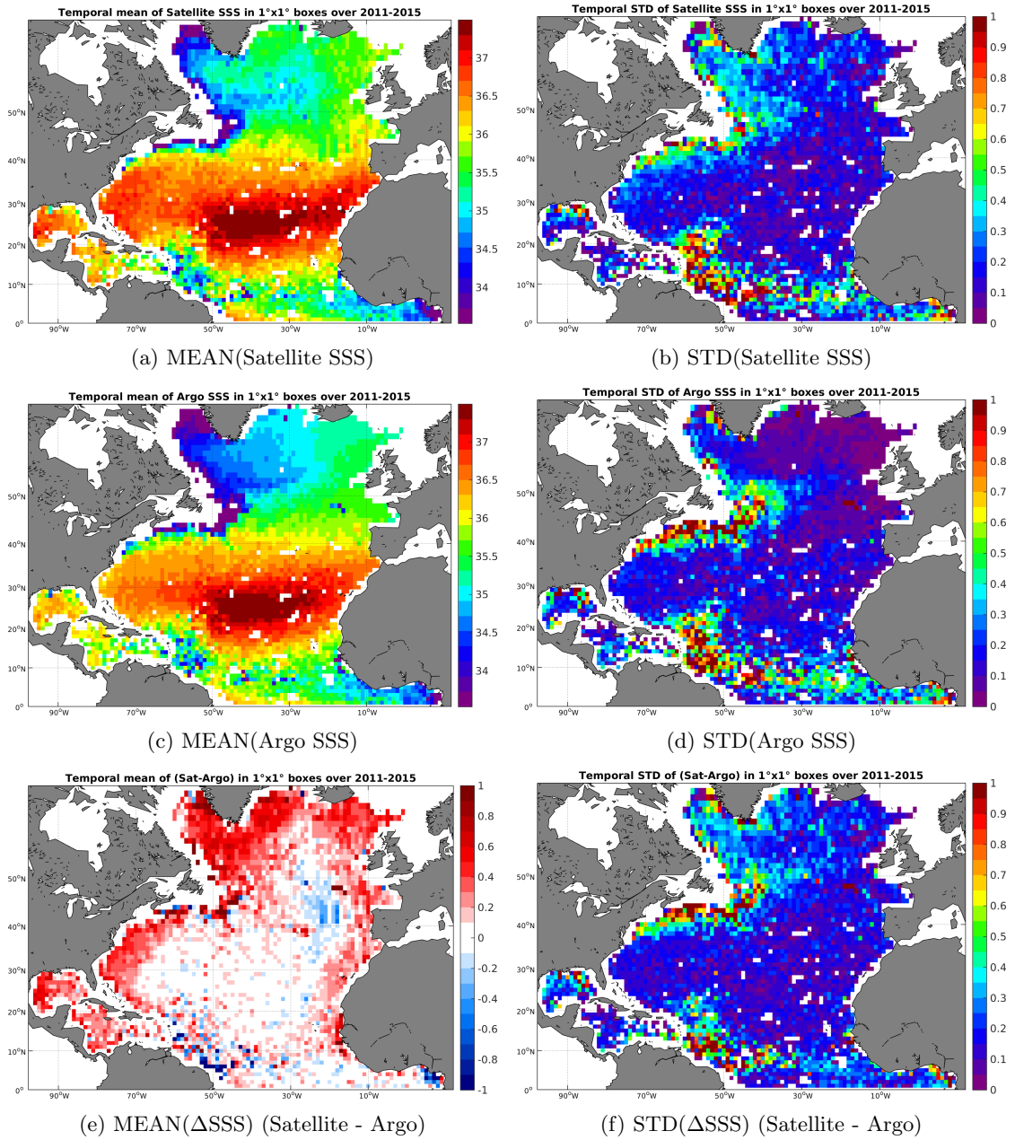
Figure 6: Temporal mean (left) and STD (right) of SSS from Aquarius-L3-JPL-V4-MONTHLY (top), Argo (middle), and of \Delta SSS (Satellite - Argo). Only match-up pairs are used to generate these maps.
