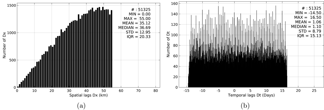
Figure 5: Histograms of the spatial (a) and temporal (b) lags between the time of the Argo measurements and the date of the corresponding Aquarius-L3-JPL-V4-MONTHLY SSS product.
