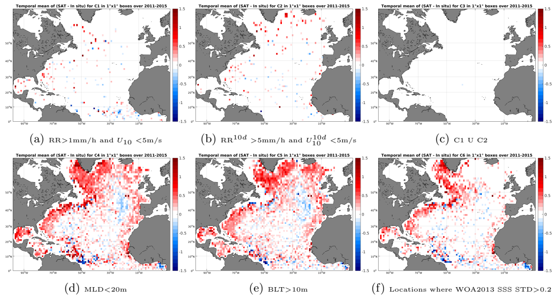
Figure 12: Temporal mean gridded over spatial boxes of size 1^\circ \times 1^\circ of \Delta SSS (Aquarius-L3-JPL-V4-MONTHLY - Argo) for 6 different subdatasets corresponding to: RR > 1\text{mm/h} and U_{10} < 5\text{m/s} (a), RR^{10d} > 5\text{mm/h} and U_{10}^{10d} < 5\text{m/s} (b), C1 U C2 (c), MLD < 20\text{m} (d), BLT > 10\text{m} (e), Locations where WOA2013 SSS STD > 0.2 (f).
