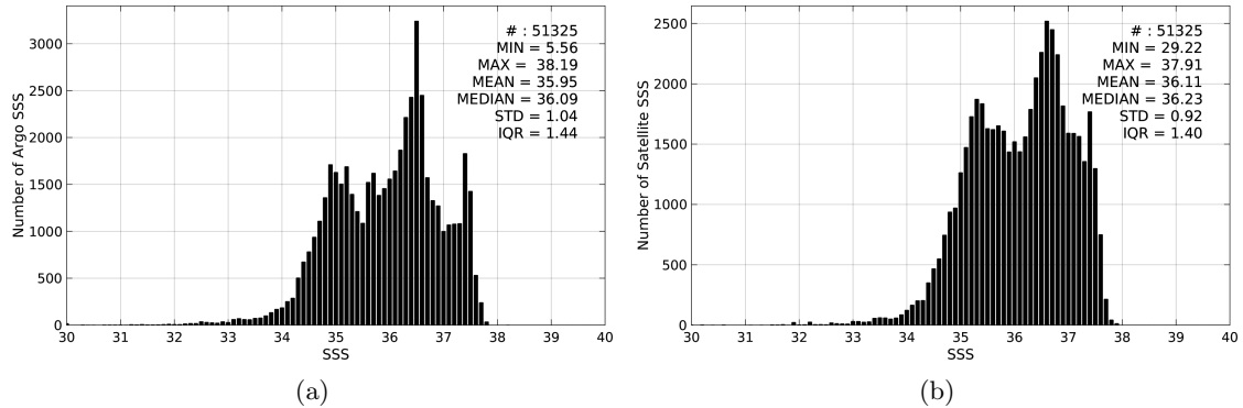
Figure 2: Histograms of SSS from Argo (a) and Aquarius-L3-JPL-V4-MONTHLY (b) considering all match-up pairs per bins of 0.1 over the North Atlantic Ocean Pi-MEP region and for the full satellite product period.
