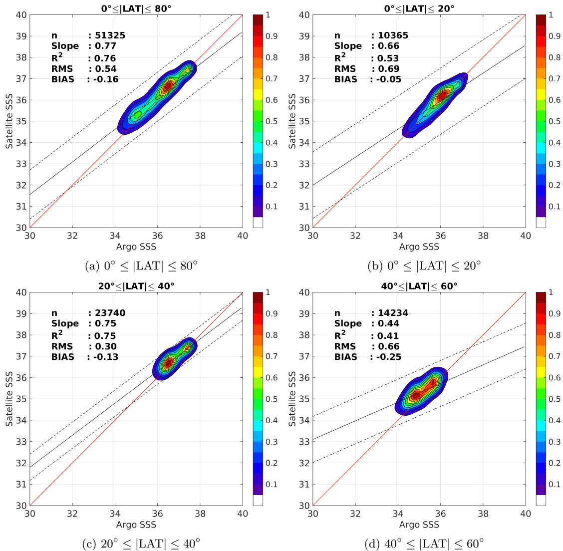
Figure 9: Contour maps of the concentration of Aquarius-L3-JPL-V4-MONTHLY SSS (y-axis) versus Argo SSS (x-axis) at match-up pairs for different latitude bands. For each plot, the red line shows x=y . The black thin and dashed lines indicate a linear fit through the data cloud and the \pm 95\% confidence levels, respectively. The number match-up pairs n , the slope and R^2 coefficient of the linear fit, the root mean square (RMS) and the mean bias between satellite and in situ data are indicated for each latitude band in each plots.
