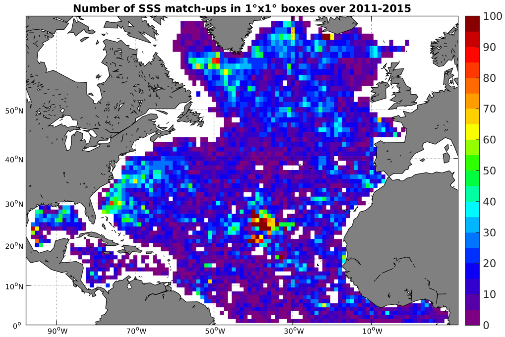
Figure 4: Number of SSS match-ups between Argo SSS and the Aquarius-L3-JPL-V4-MONTHLY SSS product for the North Atlantic Ocean Pi-MEP region over 1^\circ \times 1^\circ boxes and for the full satellite product period.
