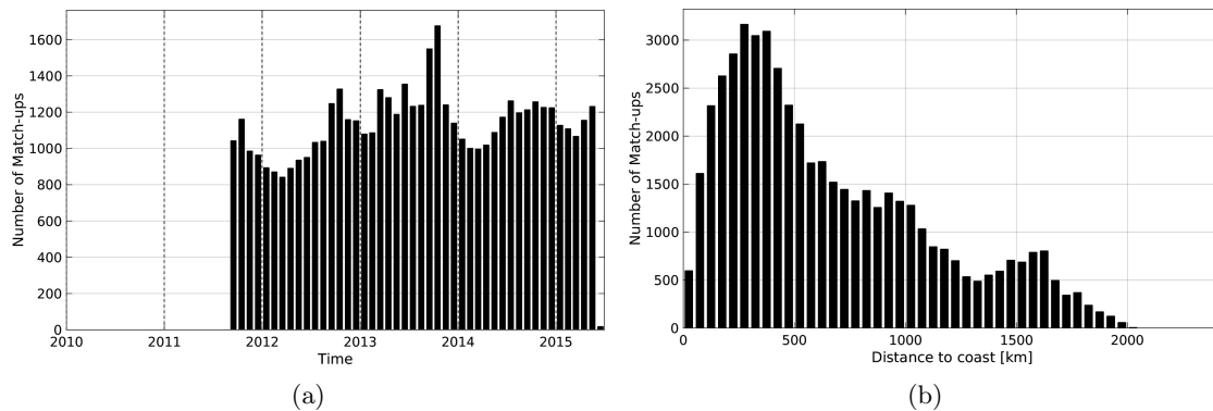
Figure 1: Number of match-ups between Argo and Aquarius-L3-JPL-V4-MONTHLY SSS as a function of time (a) and as function of the distance to coast (b) over the North Atlantic Ocean Pi-MEP region and for the full satellite product period.
