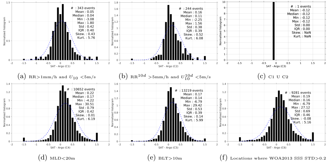
Figure 13: Normalized histogram of \Delta SSS (Aquarius-L3-JPL-V4-MONTHLY - Argo) for 6 different subdatasets corresponding to: RR>1mm/h and U_{10} < 5\text{m/s} (a), RR^{10d} > 5\text{mm/h} and U_{10}^{10d} < 5\text{m/s} (b), C1 U C2 (c), MLD<20m (d), BLT>10m (e), Locations where WOA2013 SSS STD>0.2 (f).
