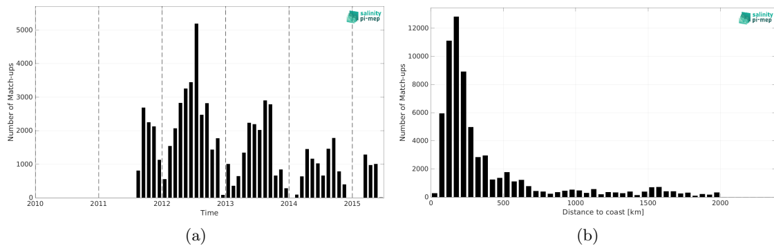
Figure 2: Number of match-ups between TSG (SAMOS) and Aquarius SSS L2 OR v5 (NASA-GSFC) SSS as a function of time (a) and as function of the distance to coast (b) over the North Atlantic Ocean Pi-MEP region and for the full satellite product period.
