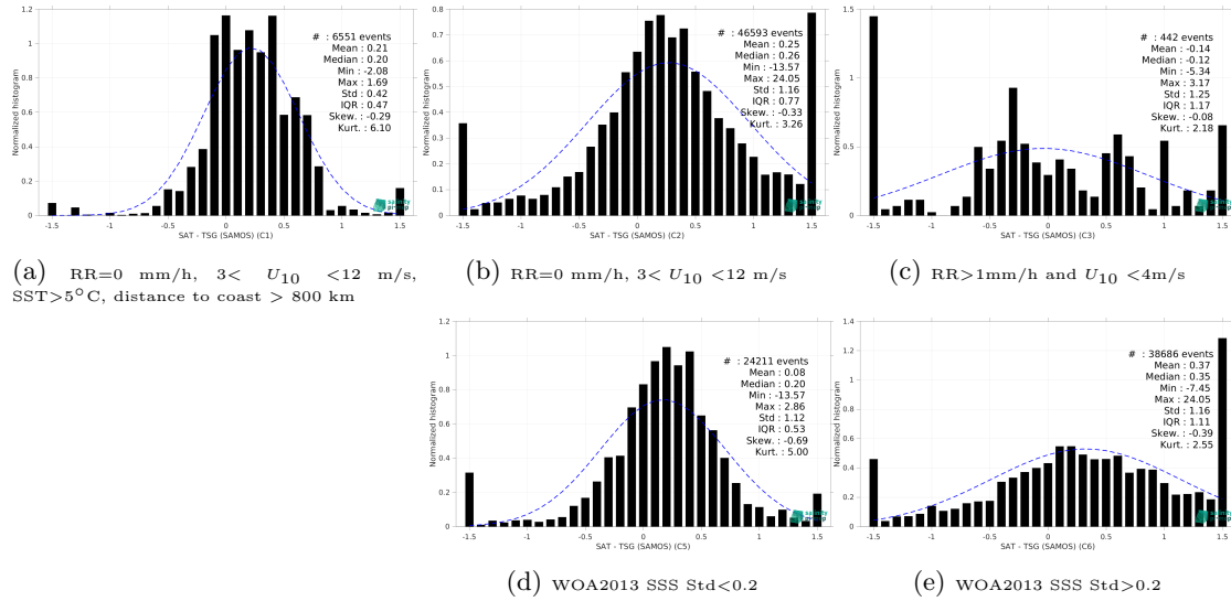
Figure 15: Normalized histogram of \Delta\text{SSS} (Aquarius SSS L2 OR v5 (NASA-GSFC) - TSG (SAMOS)) for 5 different subdatasets corresponding to: RR=0 mm/h, 3 < U_{10} < 12 m/s, SST>5°C, distance to coast > 800 km (a), RR=0 mm/h, 3 < U_{10} < 12 m/s (b), RR>1mm/h and U_{10} < 4 m/s (c), WOA2013 SSS Std<0.2 (d), WOA2013 SSS Std>0.2 (e).
