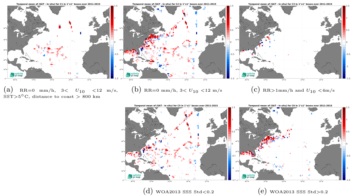
Figure 14: Temporal mean gridded over spatial boxes of size 1^\circ \times 1^\circ of \Delta SSS (Aquarius SSS L2 OR v5 (NASA-GSFC) - TSG (SAMOS)) for 5 different subdatasets corresponding to:RR=0 mm/h, 3 < U_{10} < 12 m/s, SST >5^\circ\text{C} , distance to coast > 800 km (a), RR=0 mm/h, 3 < U_{10} < 12 m/s (b), RR >1 mm/h and U_{10} < 4 m/s (c), WOA2013 SSS Std <0.2 (d), WOA2013 SSS Std >0.2 (e).
