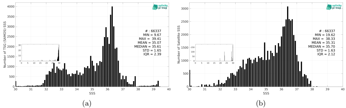
Figure 3: Histograms of SSS from TSG (SAMOS) (a) and Aquarius SSS L2 OR v5 (NASA-GSFC) (b) considering all match-up pairs per bins of 0.1 over the North Atlantic Ocean Pi-MEP region and for the full satellite product period.
