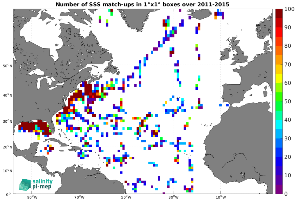
Figure 5: Number of SSS match-ups between TSG (SAMOS) SSS and the Aquarius SSS L2 OR v5 (NASA-GSFC) SSS product for the North Atlantic Ocean Pi-MEP region over 1°x1° boxes and for the full satellite product period.
