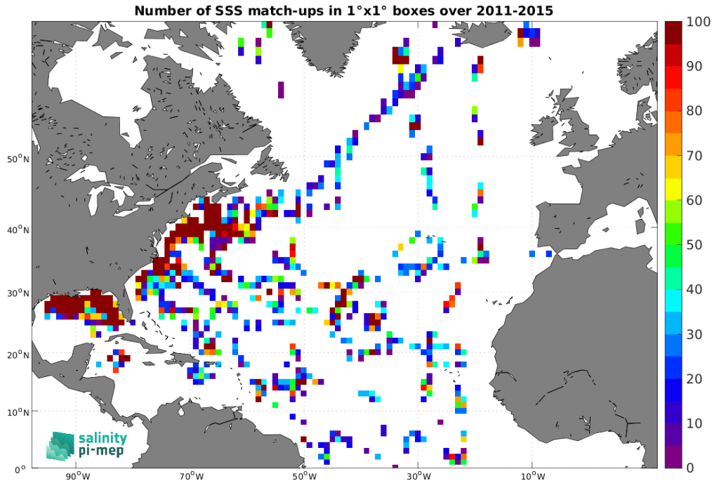
Figure 4: Number of SSS match-ups between TSG (SAMOS) SSS and the Aquarius SSS L2 OR v5 (NASA-GSFC) SSS product for the North Atlantic Ocean Pi-MEP region over 1^\circ \times 1^\circ boxes and for the full satellite product period.
