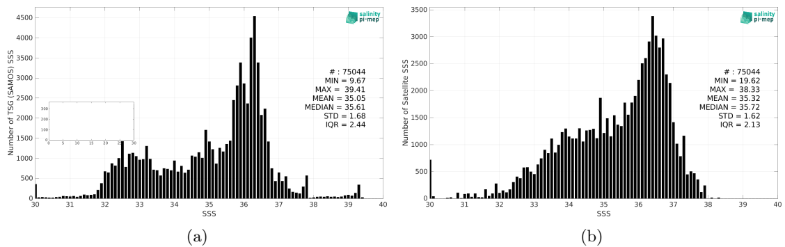
Figure 2: Histograms of SSS from TSG (SAMOS) (a) and Aquarius SSS L2 OR v5 (NASA-GSFC) (b) considering all match-up pairs per bins of 0.1 over the North Atlantic Ocean Pi-MEP region and for the full satellite product period.
