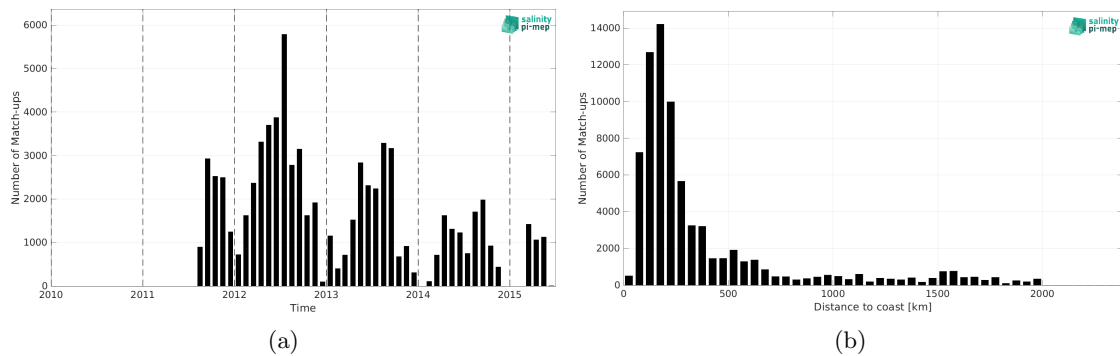
Figure 1: Number of match-ups between TSG (SAMOS) and Aquarius SSS L2 OR v5 (NASA-GSFC) SSS as a function of time (a) and as function of the distance to coast (b) over the North Atlantic Ocean Pi-MEP region and for the full satellite product period.
