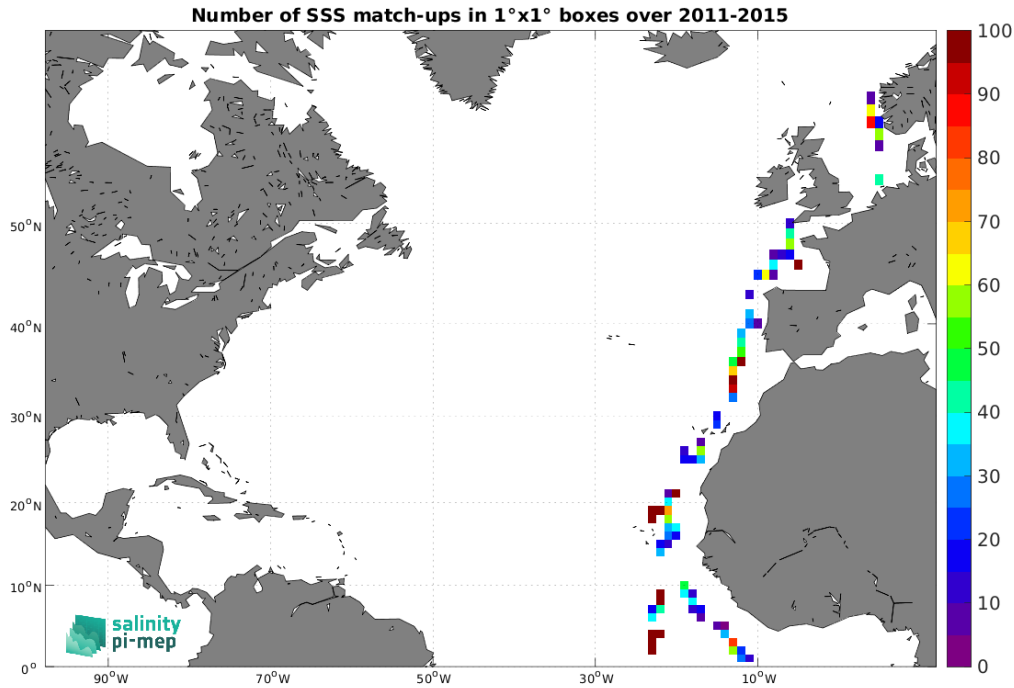
Figure 5: Number of SSS match-ups between TSG (Polarstern) SSS and the Aquarius SSS L2 OR v5 (NASA-GSFC) SSS product for the North Atlantic Ocean Pi-MEP region over 1^\circ \times 1^\circ boxes and for the full satellite product period.
