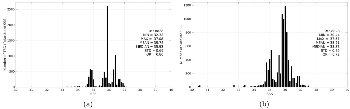
Figure 3: Histograms of SSS from TSG (Polarstern) (a) and Aquarius SSS L2 OR v5 (NASA-GSFC) (b) considering all match-up pairs per bins of 0.1 over the North Atlantic Ocean Pi-MEP region and for the full satellite product period.
