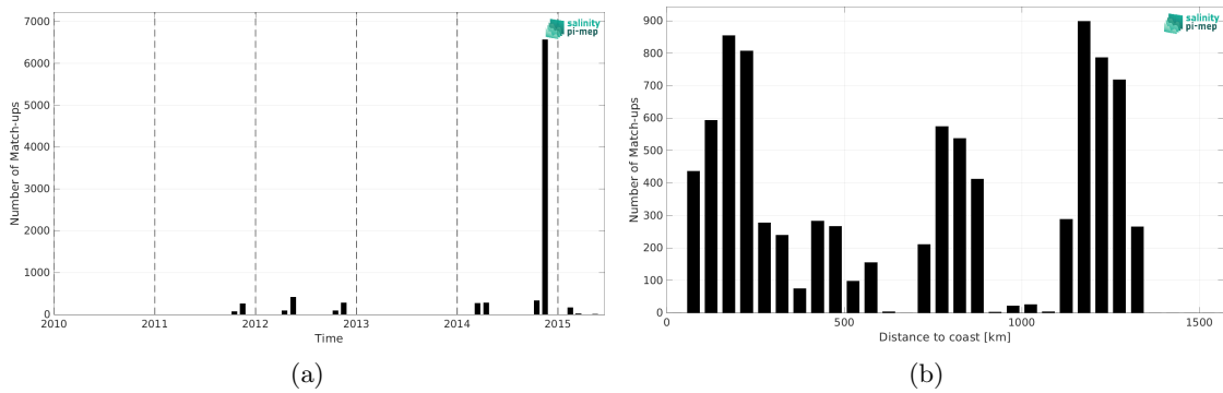
Figure 2: Number of match-ups between TSG (Polarstern) and Aquarius SSS L2 OR v5 (NASA-GSFC) SSS as a function of time (a) and as function of the distance to coast (b) over the North Atlantic Ocean Pi-MEP region and for the full satellite product period.
