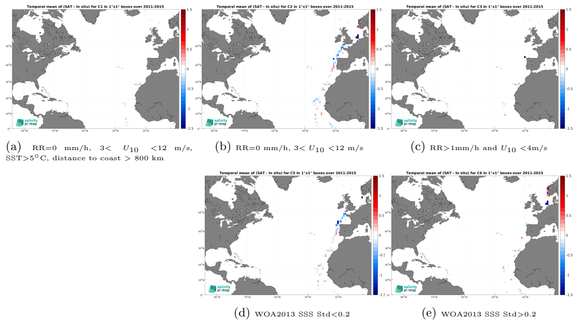
Figure 14: Temporal mean gridded over spatial boxes of size 1^\circ \times 1^\circ of \Delta\text{SSS} (Aquarius SSS L2 OR v5 (NASA-GSFC) - TSG (Polarstern)) for 5 different subdatasets corresponding to:RR=0 mm/h, 3 < U_{10} < 12 m/s, SST >5^\circ\text{C} , distance to coast > 800 km (a), RR=0 mm/h, 3 < U_{10} < 12 m/s (b), RR >1 mm/h and U_{10} < 4 m/s (c), WOA2013 SSS Std <0.2 (d), WOA2013 SSS Std >0.2 (e).
