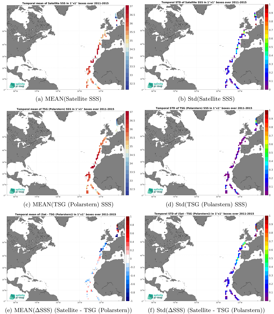
Figure 7: Temporal mean (left) and Std (right) of SSS from Aquarius SSS L2 OR v5 (NASA-GSFC) (top), TSG (Polarstern) (middle), and of \Delta SSS (Satellite - TSG (Polarstern)). Only match-up pairs are used to generate these maps.
