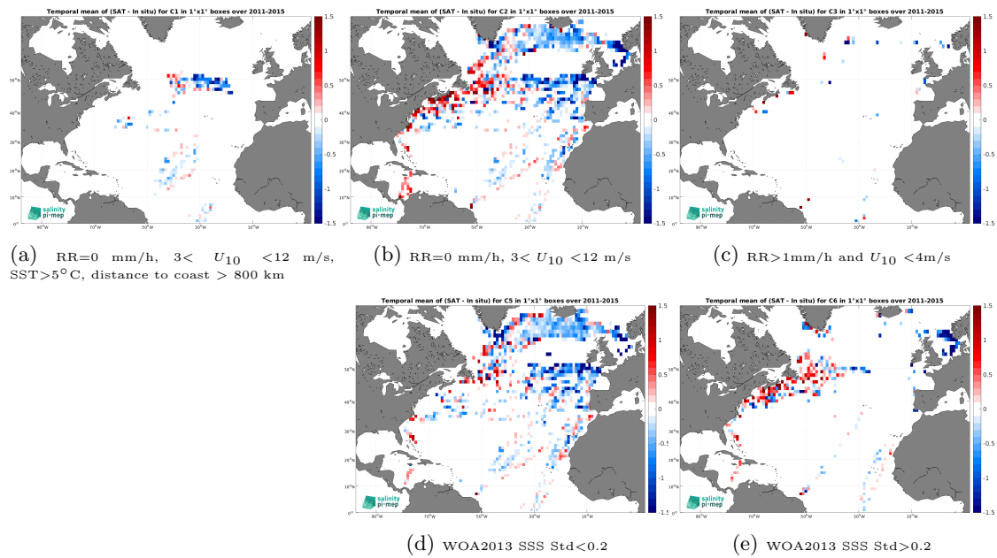
Figure 14: Temporal mean gridded over spatial boxes of size 1^\circ \times 1^\circ of \Delta\text{SSS} (Aquarius SSS L2 OR v5 (NASA-GSFC) - TSG (LEGOS-DM)) for 5 different subdatasets corresponding to:RR=0 mm/h, 3 < U_{10} < 12 m/s, SST >5^\circ\text{C} , distance to coast > 800 km (a), RR=0 mm/h, 3 < U_{10} < 12 m/s (b), RR >1 mm/h and U_{10} < 4 m/s (c), WOA2013 SSS Std <0.2 (d), WOA2013 SSS Std >0.2 (e).
