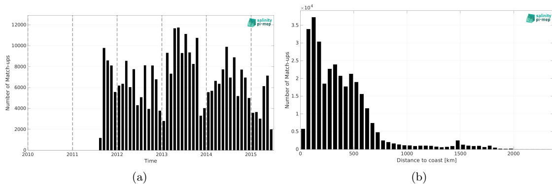
Figure 2: Number of match-ups between TSG (LEGOS-DM) and Aquarius SSS L2 OR v5 (NASA-GSFC) SSS as a function of time (a) and as function of the distance to coast (b) over the North Atlantic Ocean Pi-MEP region and for the full satellite product period.
