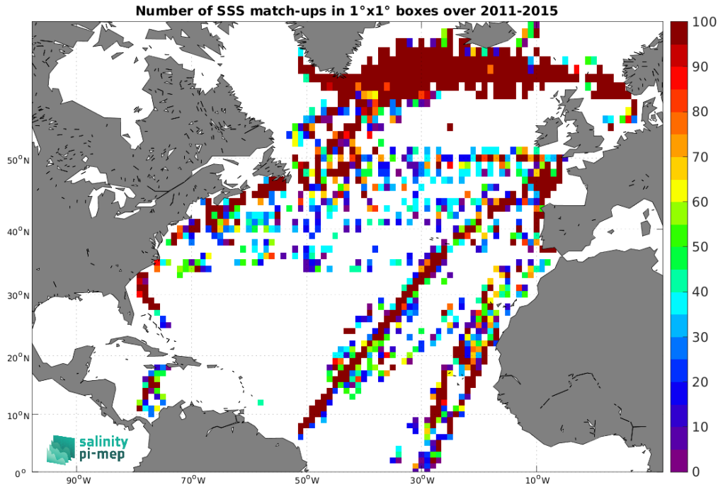
Figure 5: Number of SSS match-ups between TSG (LEGOS-DM) SSS and the Aquarius SSS L2 OR v5 (NASA-GSFC) SSS product for the North Atlantic Ocean Pi-MEP region over 1^\circ \times 1^\circ boxes and for the full satellite product period.
