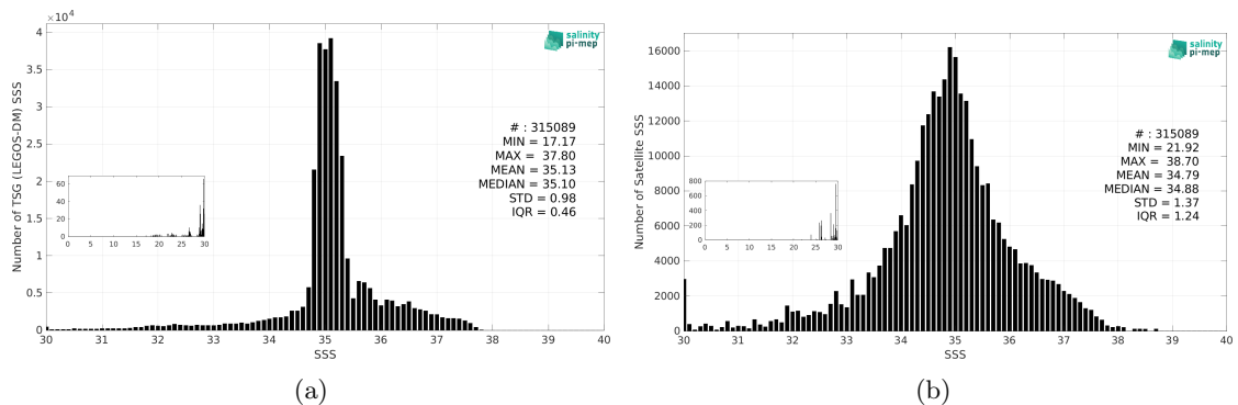
Figure 3: Histograms of SSS from TSG (LEGOS-DM) (a) and Aquarius SSS L2 OR v5 (NASA-GSFC) (b) considering all match-up pairs per bins of 0.1 over the North Atlantic Ocean Pi-MEP region and for the full satellite product period.
