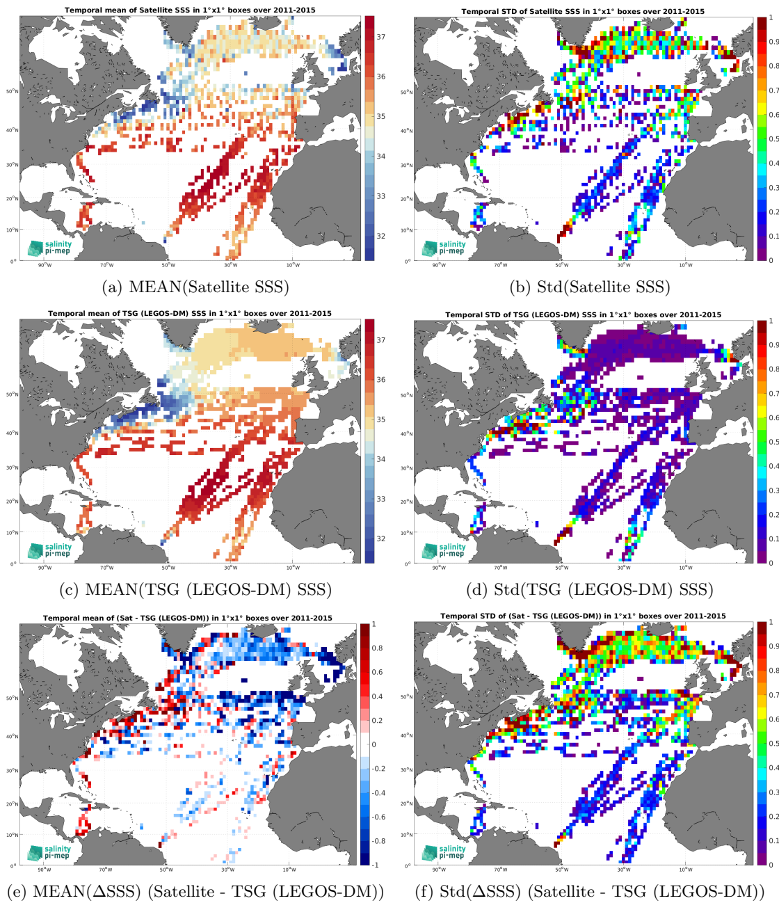
Figure 7: Temporal mean (left) and Std (right) of SSS from Aquarius SSS L2 OR v5 (NASA-GSFC) (top), TSG (LEGOS-DM) (middle), and of \Delta SSS (Satellite - TSG (LEGOS-DM)). Only match-up pairs are used to generate these maps.
