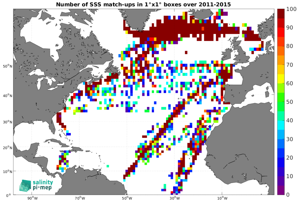
Figure 4: Number of SSS match-ups between TSG (LEGOS-DM) SSS and the Aquarius SSS L2 OR v5 (NASA-GSFC) SSS product for the North Atlantic Ocean Pi-MEP region over 1^\circ \times 1^\circ boxes and for the full satellite product period.
