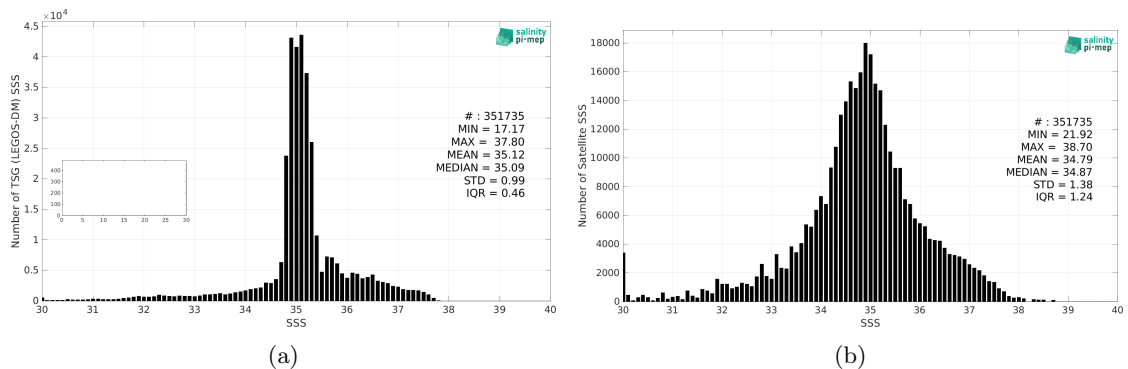
Figure 2: Histograms of SSS from TSG (LEGOS-DM) (a) and Aquarius SSS L2 OR v5 (NASA-GSFC) (b) considering all match-up pairs per bins of 0.1 over the North Atlantic Ocean Pi-MEP region and for the full satellite product period.
