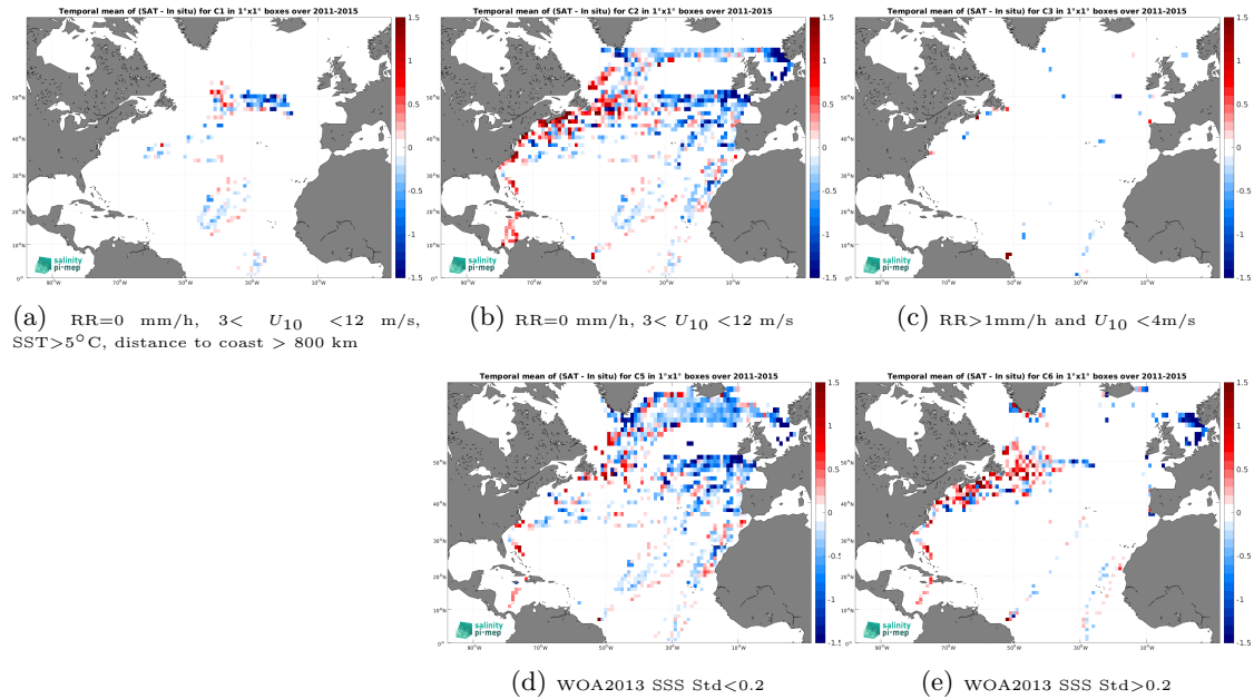
Figure 12: Temporal mean gridded over spatial boxes of size 1^\circ \times 1^\circ of \Delta\text{SSS} (Aquarius SSS L2 OR v5 (NASA-GSFC) - TSG (LEGOS-DM)) for 5 different subdatasets corresponding to:RR=0 mm/h, 3 < U_{10} < 12 m/s, SST >5^\circ\text{C} , distance to coast > 800 km (a), RR=0 mm/h, 3 < U_{10} < 12 m/s (b), RR >1 mm/h and U_{10} < 4 m/s (c), WOA2013 SSS Std <0.2 (d), WOA2013 SSS Std >0.2 (e).
