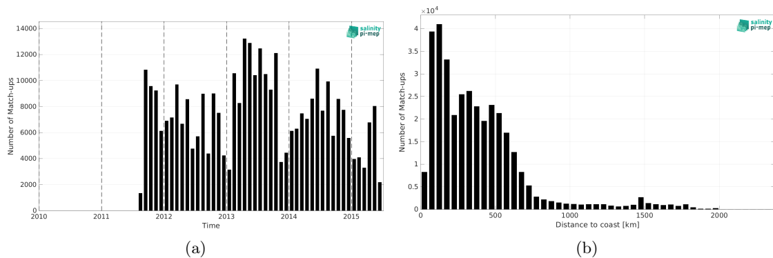
Figure 1: Number of match-ups between TSG (LEGOS-DM) and Aquarius SSS L2 OR v5 (NASA-GSFC) SSS as a function of time (a) and as function of the distance to coast (b) over the North Atlantic Ocean Pi-MEP region and for the full satellite product period.
