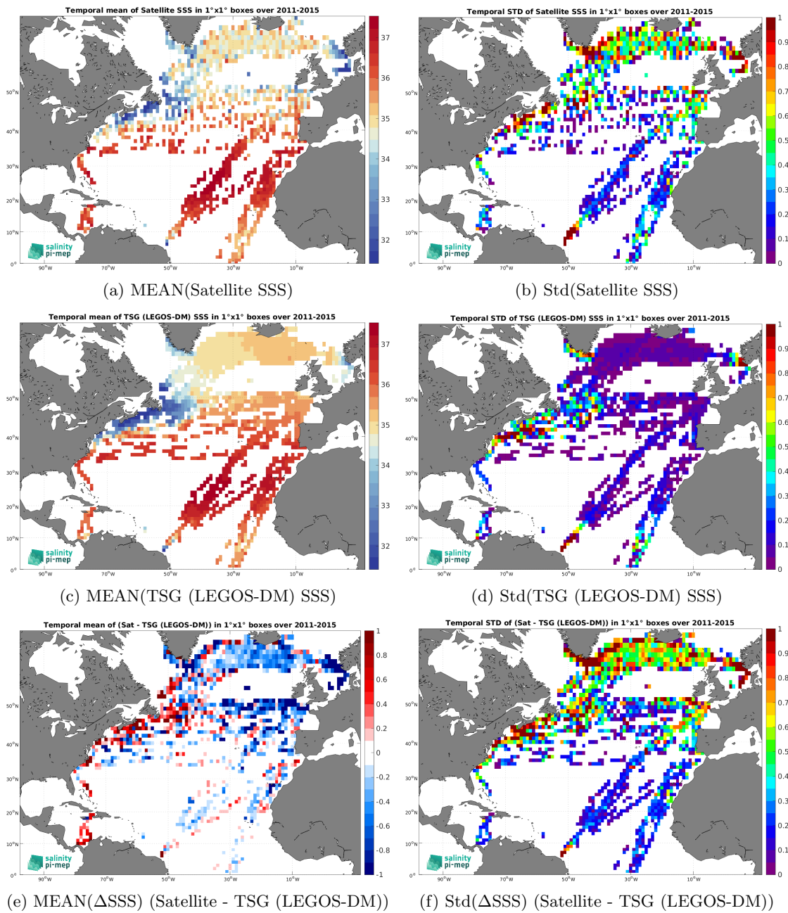
Figure 6: Temporal mean (left) and Std (right) of SSS from Aquarius SSS L2 OR v5 (NASA-GSFC) (top), TSG (LEGOS-DM) (middle), and of \Delta SSS (Satellite - TSG (LEGOS-DM)). Only match-up pairs are used to generate these maps.
