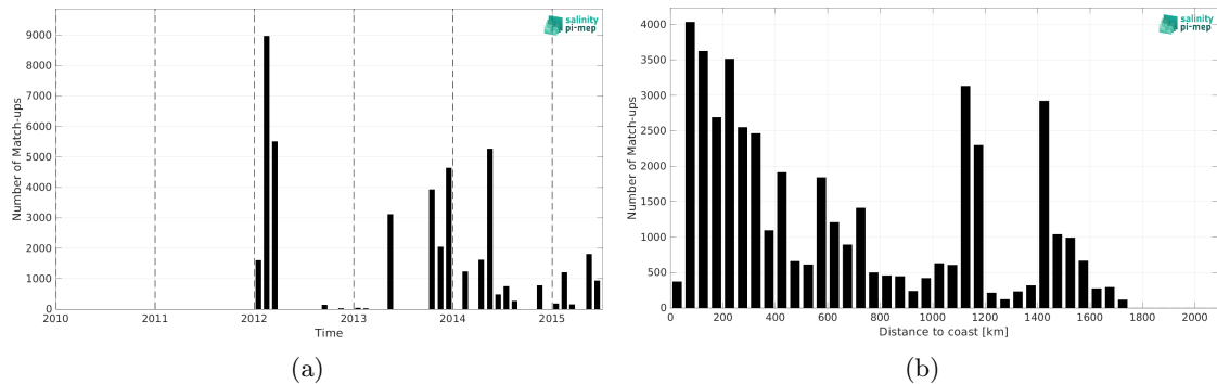
Figure 2: Number of match-ups between TSG (GOSUD-Sailing-ship) and Aquarius SSS L2 OR v5 (NASA-GSFC) SSS as a function of time (a) and as function of the distance to coast (b) over the North Atlantic Ocean Pi-MEP region and for the full satellite product period.
