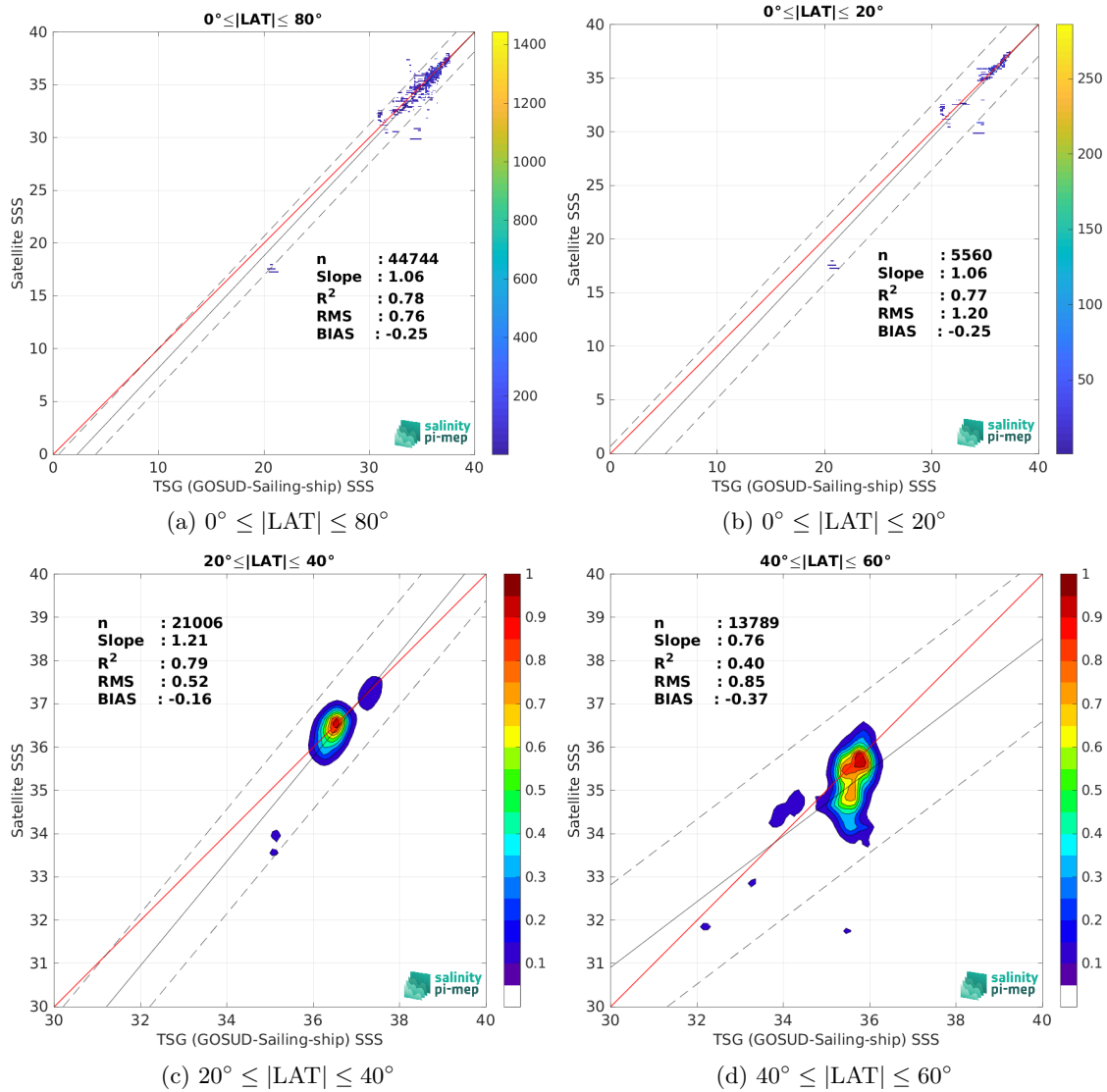
Figure 10: Contour maps of the concentration of Aquarius SSS L2 OR v5 (NASA-GSFC) SSS (y-axis) versus TSG (GOSUD-Sailing-ship) SSS (x-axis) at match-up pairs for different latitude bands. For each plot, the red line shows x=y . The black thin and dashed lines indicate a linear fit through the data cloud and the \pm 95\% confidence levels, respectively. The number match-up pairs n , the slope and R^2 coefficient of the linear fit, the root mean square (RMS) and the mean bias between satellite and in situ data are indicated for each latitude band in each plots.
