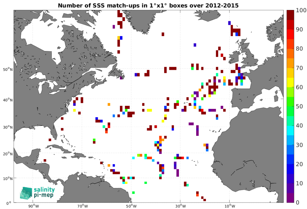
Figure 5: Number of SSS match-ups between TSG (GOSUD-Sailing-ship) SSS and the Aquarius SSS L2 OR v5 (NASA-GSFC) SSS product for the North Atlantic Ocean Pi-MEP region over 1°×1° boxes and for the full satellite product period.
