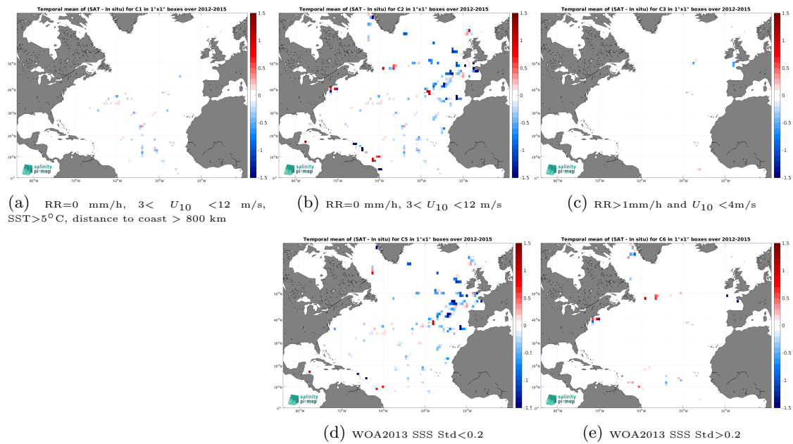
Figure 14: Temporal mean gridded over spatial boxes of size 1^\circ \times 1^\circ of \Delta\text{SSS} (Aquarius SSS L2 OR v5 (NASA-GSFC) - TSG (GOSUD-Sailing-ship)) for 5 different subdatasets corresponding to:RR=0 mm/h, 3 < U_{10} < 12 m/s, SST>5°C, distance to coast > 800 km (a), RR=0 mm/h, 3 < U_{10} < 12 m/s (b), RR>1mm/h and U_{10} < 4 m/s (c), WOA2013 SSS Std<0.2 (d), WOA2013 SSS Std>0.2 (e).
