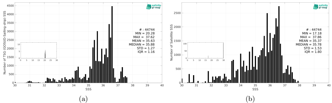
Figure 3: Histograms of SSS from TSG (GOSUD-Sailing-ship) (a) and Aquarius SSS L2 OR v5 (NASA-GSFC) (b) considering all match-up pairs per bins of 0.1 over the North Atlantic Ocean Pi-MEP region and for the full satellite product period.
