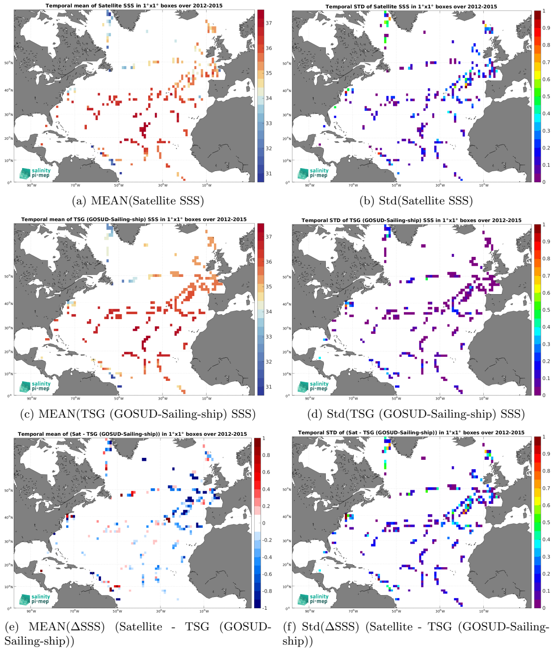
Figure 7: Temporal mean (left) and Std (right) of SSS from Aquarius SSS L2 OR v5 (NASA-GSFC) (top), TSG (GOSUD-Sailing-ship) (middle), and of \Delta SSS (Satellite - TSG (GOSUD-Sailing-ship)). Only match-up pairs are used to generate these maps.
