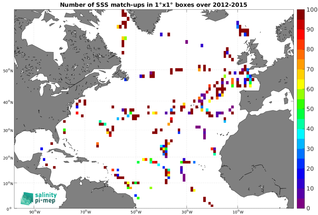
Figure 4: Number of SSS match-ups between TSG (GOSUD-Sailing-ship) SSS and the Aquarius SSS L2 OR v5 (NASA-GSFC) SSS product for the North Atlantic Ocean Pi-MEP region over 1^\circ \times 1^\circ boxes and for the full satellite product period.
