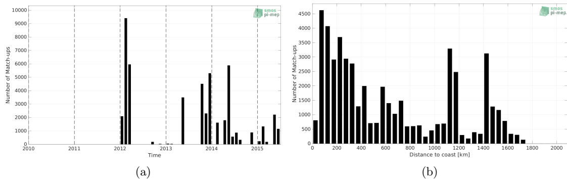
Figure 1: Number of match-ups between TSG (GOSUD-Sailing-ship) and Aquarius SSS L2 OR v5 (NASA-GSFC) SSS as a function of time (a) and as function of the distance to coast (b) over the North Atlantic Ocean Pi-MEP region and for the full satellite product period.
