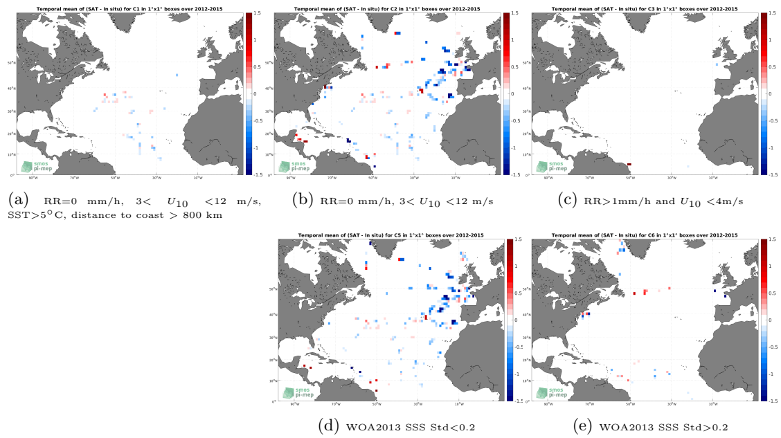
Figure 12: Temporal mean gridded over spatial boxes of size 1^\circ \times 1^\circ of \Delta\text{SSS} (Aquarius SSS L2 OR v5 (NASA-GSFC) - TSG (GOSUD-Sailing-ship)) for 5 different subdatasets corresponding to:RR=0 mm/h, 3 < U_{10} < 12 m/s, SST>5°C, distance to coast > 800 km (a), RR=0 mm/h, 3 < U_{10} < 12 m/s (b), RR>1mm/h and U_{10} < 4 m/s (c), WOA2013 SSS Std<0.2 (d), WOA2013 SSS Std>0.2 (e).
