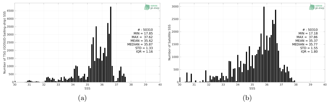
Figure 2: Histograms of SSS from TSG (GOSUD-Sailing-ship) (a) and Aquarius SSS L2 OR v5 (NASA-GSFC) (b) considering all match-up pairs per bins of 0.1 over the North Atlantic Ocean Pi-MEP region and for the full satellite product period.
