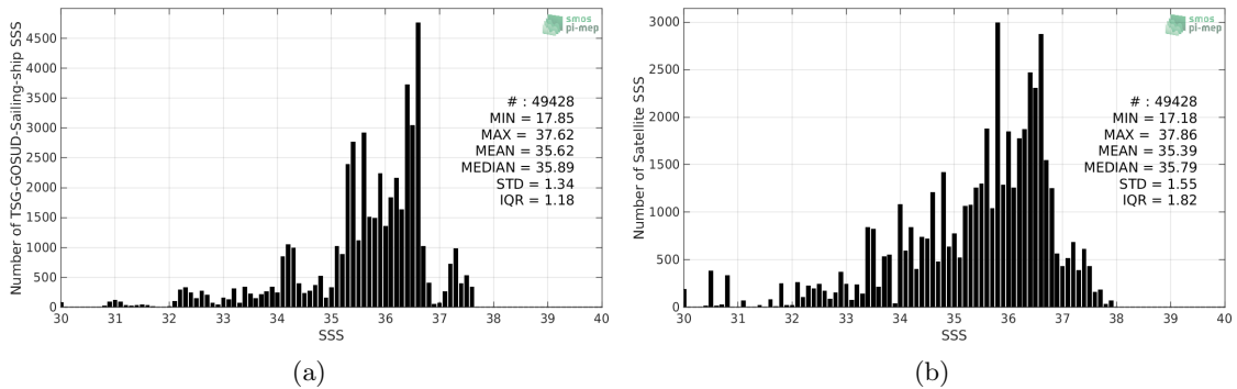
Figure 2: Histograms of SSS from TSG-GOSUD-Sailing-ship (a) and Aquarius-L2-OR-V5 (b) considering all match-up pairs per bins of 0.1 over the North Atlantic Ocean Pi-MEP region and for the full satellite product period.
