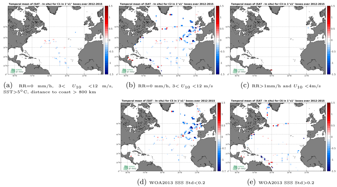
Figure 12: Temporal mean gridded over spatial boxes of size 1^\circ \times 1^\circ of \Delta SSS (Aquarius-L2-OR-V5 - TSG-GOSUD-Sailing-ship) for 5 different subdatasets corresponding to: RR=0 mm/h, 3 < U_{10} < 12 m/s, SST > 5°C, distance to coast > 800 km (a), RR=0 mm/h, 3 < U_{10} < 12 m/s (b), RR > 1mm/h and U_{10} < 4 m/s (c), WOA2013 SSS Std < 0.2 (d), WOA2013 SSS Std > 0.2 (e).
