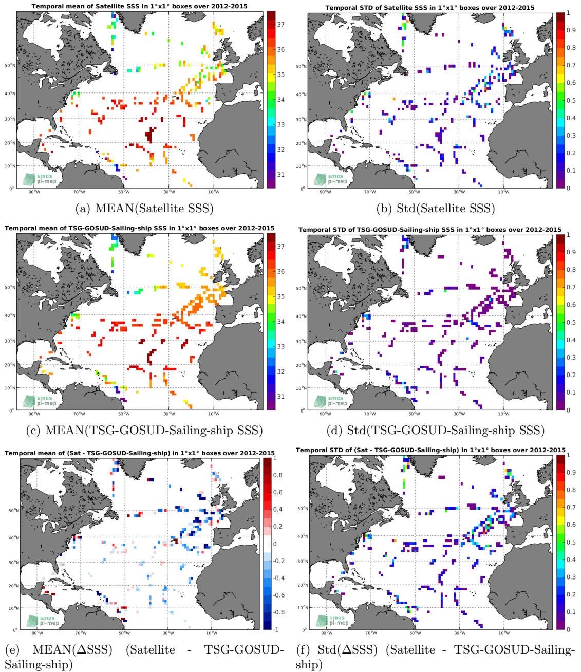
Figure 6: Temporal mean (left) and Std (right) of SSS from Aquarius-L2-OR-V5 (top), TSG-GOSUD-Sailing-ship (middle), and of \Delta SSS (Satellite - TSG-GOSUD-Sailing-ship). Only match-up pairs are used to generate these maps.
