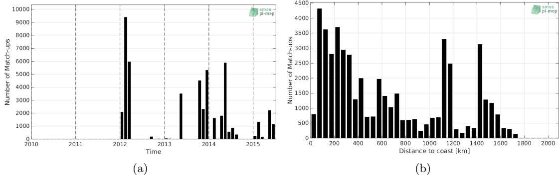
Figure 1: Number of match-ups between TSG-GOSUD-Sailing-ship and Aquarius-L2-OR-V5 SSS as a function of time (a) and as function of the distance to coast (b) over the North Atlantic Ocean Pi-MEP region and for the full satellite product period.
