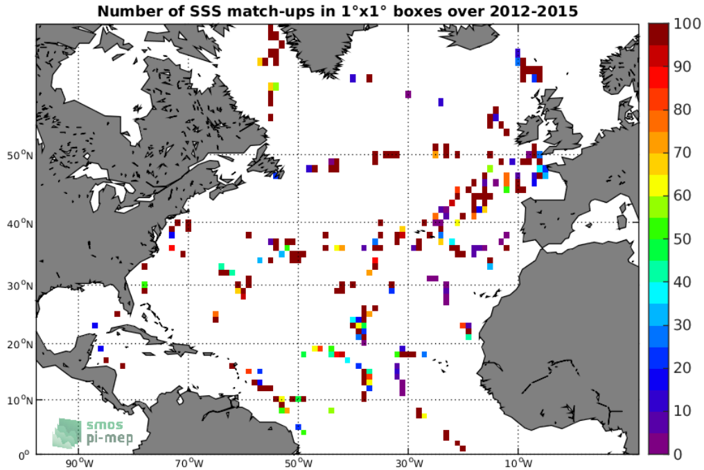
Figure 4: Number of SSS match-ups between TSG-GOSUD-Sailing-ship SSS and the Aquarius-L2-OR-V5 SSS product for the North Atlantic Ocean Pi-MEP region over 1^\circ \times 1^\circ boxes and for the full satellite product period.
