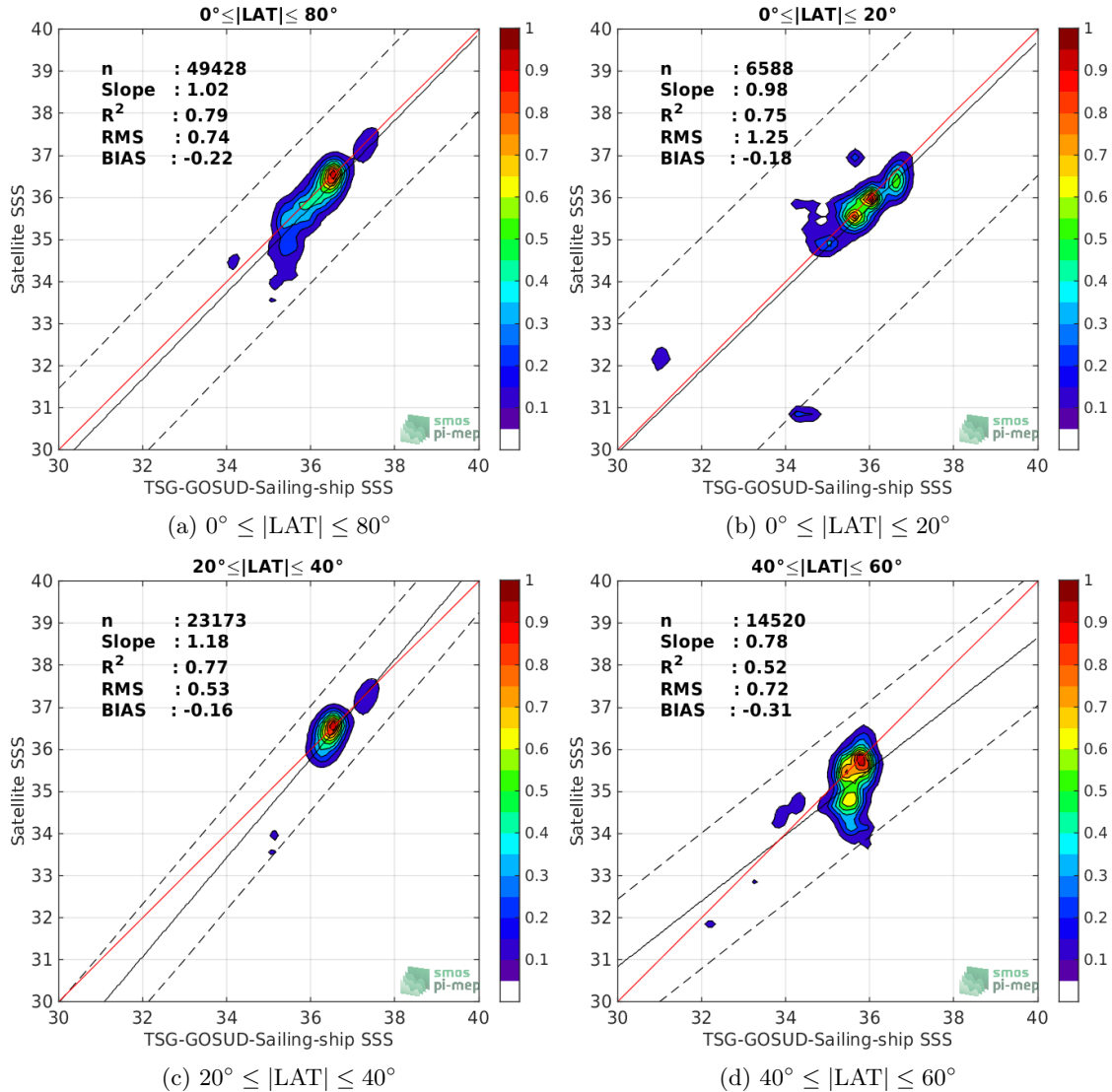
Figure 9: Contour maps of the concentration of Aquarius-L2-OR-V5 SSS (y-axis) versus TSG-GOSUD-Sailing-ship SSS (x-axis) at match-up pairs for different latitude bands. For each plot, the red line shows x=y . The black thin and dashed lines indicate a linear fit through the data cloud and the \pm 95\% confidence levels, respectively. The number match-up pairs n , the slope and R^2 coefficient of the linear fit, the root mean square (RMS) and the mean bias between satellite and in situ data are indicated for each latitude band in each plots.
