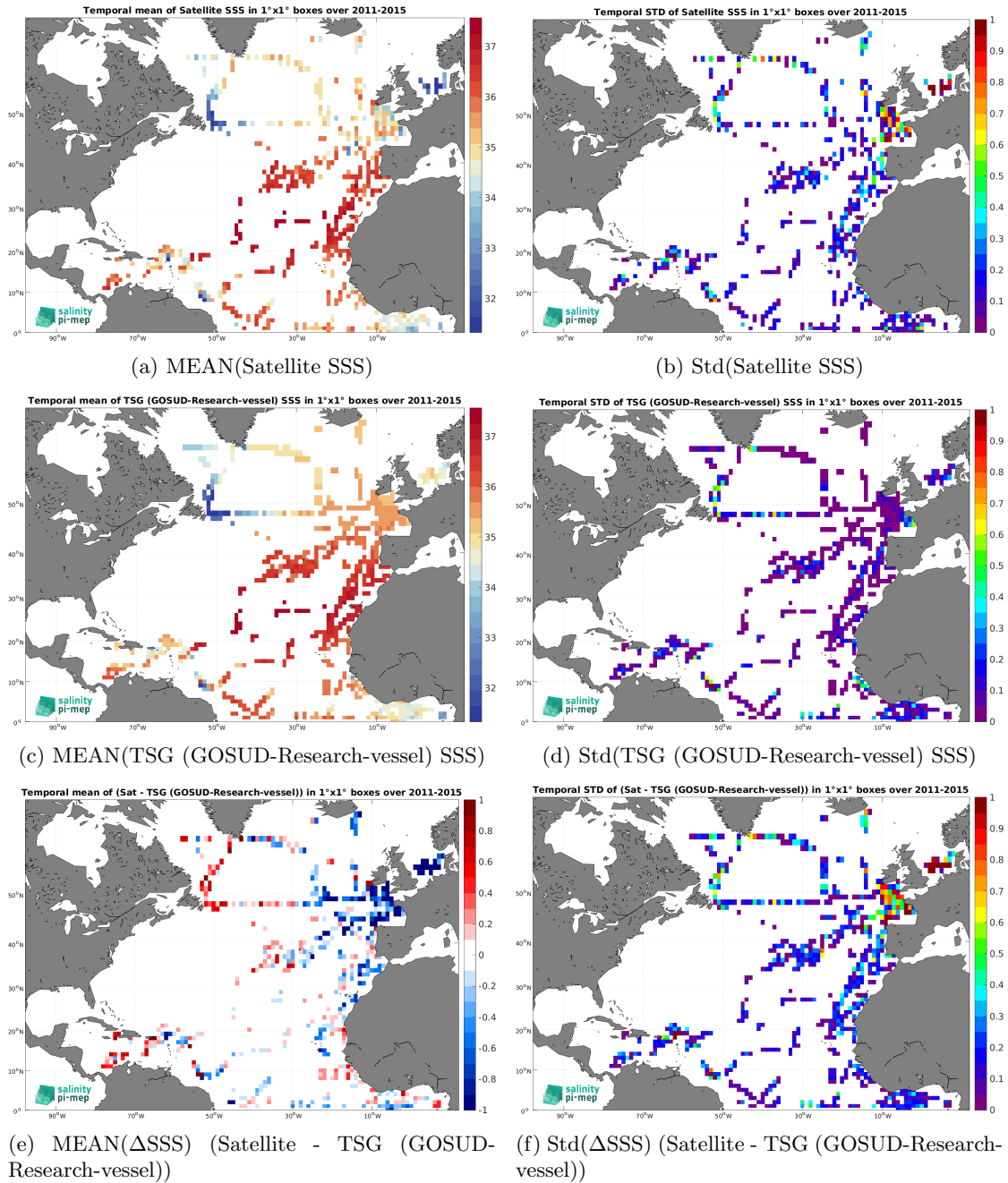
Figure 7: Temporal mean (left) and Std (right) of SSS from Aquarius SSS L2 OR v5 (NASA-GSFC) (top), TSG (GOSUD-Research-vessel) (middle), and of \Delta SSS (Satellite - TSG (GOSUD-Research-vessel)). Only match-up pairs are used to generate these maps.
