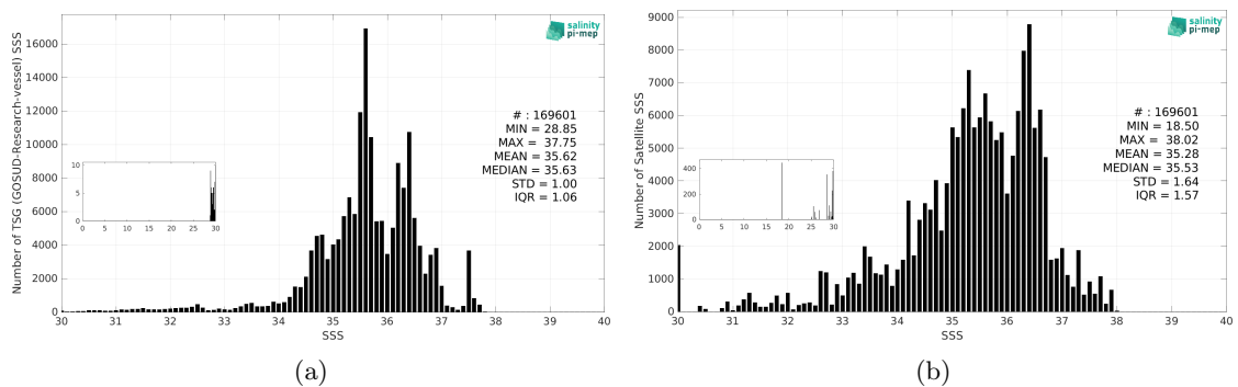
Figure 3: Histograms of SSS from TSG (GOSUD-Research-vessel) (a) and Aquarius SSS L2 OR v5 (NASA-GSFC) (b) considering all match-up pairs per bins of 0.1 over the North Atlantic Ocean Pi-MEP region and for the full satellite product period.
