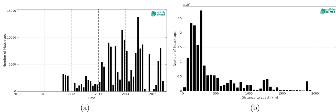
Figure 2: Number of match-ups between TSG (GOSUD-Research-vessel) and Aquarius SSS L2 OR v5 (NASA-GSFC) SSS as a function of time (a) and as function of the distance to coast (b) over the North Atlantic Ocean Pi-MEP region and for the full satellite product period.
