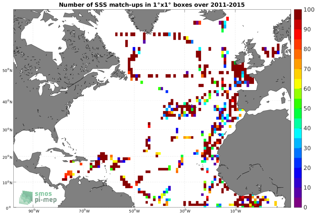
Figure 4: Number of SSS match-ups between TSG (GOSUD-Research-vessel) SSS and the Aquarius SSS L2 OR v5 (NASA-GSFC) SSS product for the North Atlantic Ocean Pi-MEP region over 1^\circ \times 1^\circ boxes and for the full satellite product period.
