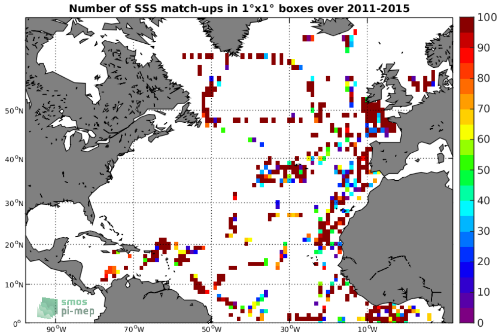
Figure 4: Number of SSS match-ups between TSG-GOSUD-Research-vessel SSS and the Aquarius-L2-OR-V5 SSS product for the North Atlantic Ocean Pi-MEP region over 1°x1° boxes and for the full satellite product period.
