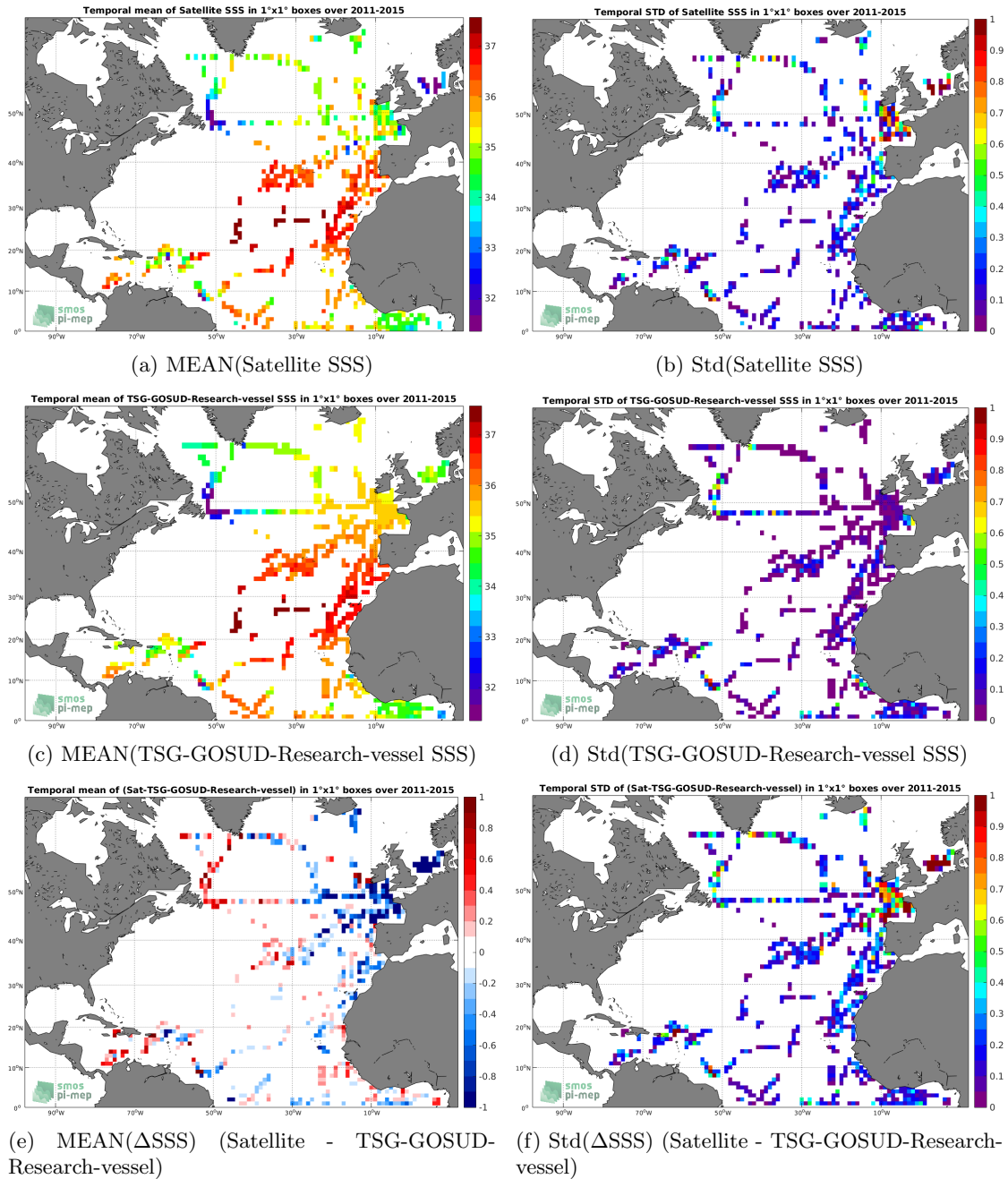
Figure 6: Temporal mean (left) and Std (right) of SSS from Aquarius-L2-OR-V5 (top), TSG-GOSUD-Research-vessel (middle), and of \Delta SSS (Satellite - TSG-GOSUD-Research-vessel). Only match-up pairs are used to generate these maps.
