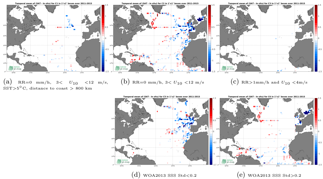
Figure 12: Temporal mean gridded over spatial boxes of size 1^\circ \times 1^\circ of \Delta SSS (Aquarius-L2-OR-V5 - TSG-GOSUD-Research-vessel) for 5 different subdatasets corresponding to:RR=0 mm/h, 3 < U_{10} < 12 m/s, SST >5^\circ\text{C} , distance to coast > 800 km (a), RR=0 mm/h, 3 < U_{10} < 12 m/s (b), RR >1 mm/h and U_{10} < 4 m/s (c), WOA2013 SSS Std <0.2 (d), WOA2013 SSS Std >0.2 (e).
