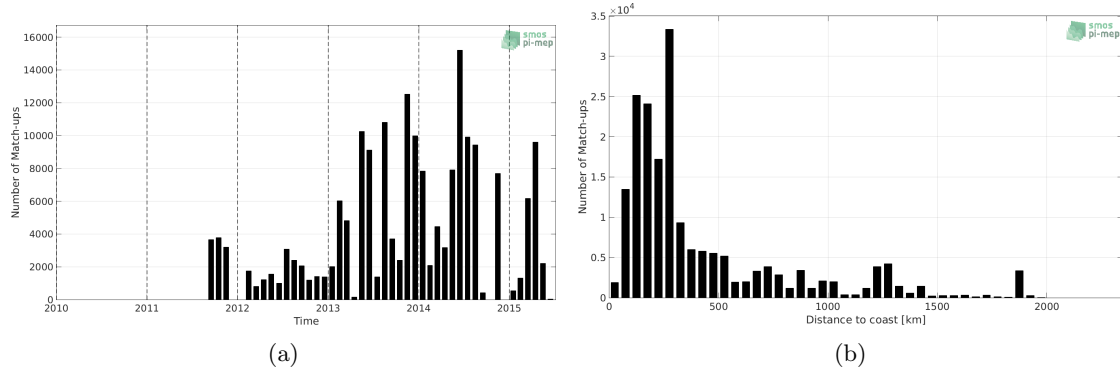
Figure 1: Number of match-ups between TSG-GOSUD-Research-vessel and Aquarius-L2-OR-V5 SSS as a function of time (a) and as function of the distance to coast (b) over the North Atlantic Ocean Pi-MEP region and for the full satellite product period.
