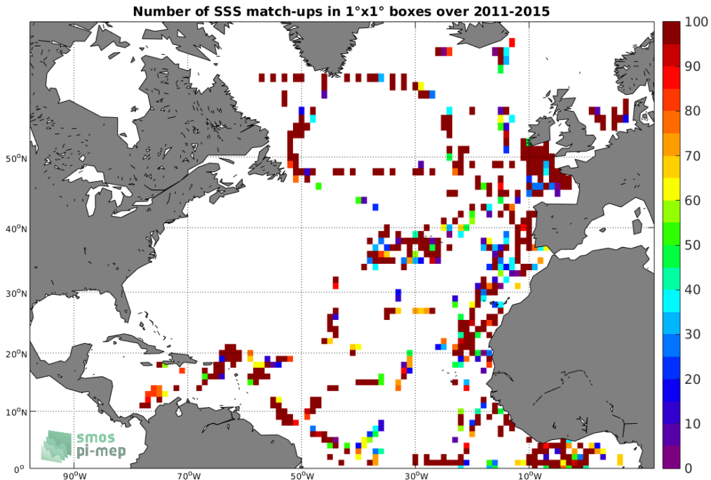
Figure 4: Number of SSS match-ups between TSG-GOSUD-Research-vessel SSS and the Aquarius-L2-OR-V5 SSS product for the North Atlantic Ocean Pi-MEP region over 1^\circ \times 1^\circ boxes and for the full satellite product period.
