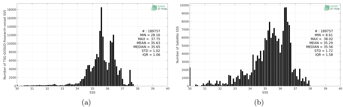
Figure 2: Histograms of SSS from TSG-GOSUD-Research-vessel (a) and Aquarius-L2-OR-V5 (b) considering all match-up pairs per bins of 0.1 over the North Atlantic Ocean Pi-MEP region and for the full satellite product period.
