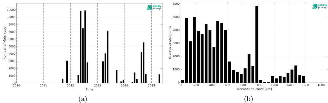
Figure 2: Number of match-ups between TSG (CSIC-UTM) and Aquarius SSS L2 OR v5 (NASA-GSFC) SSS as a function of time (a) and as function of the distance to coast (b) over the North Atlantic Ocean Pi-MEP region and for the full satellite product period.
