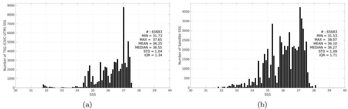
Figure 3: Histograms of SSS from TSG (CSIC-UTM) (a) and Aquarius SSS L2 OR v5 (NASA-GSFC) (b) considering all match-up pairs per bins of 0.1 over the North Atlantic Ocean Pi-MEP region and for the full satellite product period.
