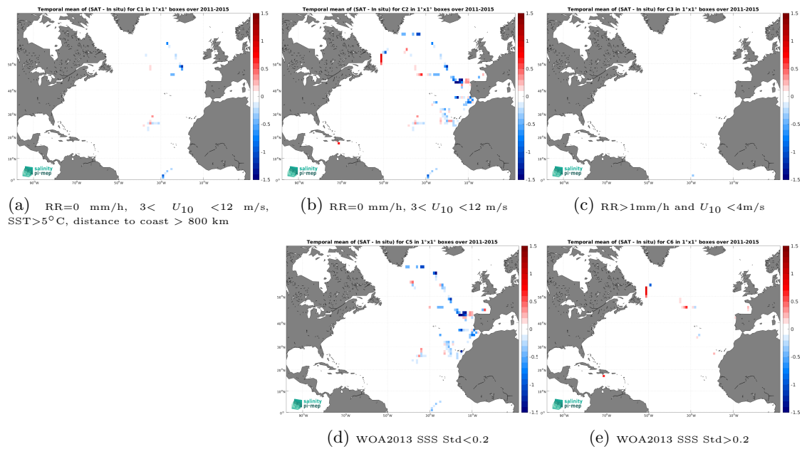
Figure 14: Temporal mean gridded over spatial boxes of size 1^\circ \times 1^\circ of \Delta\text{SSS} (Aquarius SSS L2 OR v5 (NASA-GSFC) - TSG (CSIC-UTM)) for 5 different subdatasets corresponding to:RR=0 mm/h, 3 < U_{10} < 12 m/s, SST >5^\circ\text{C} , distance to coast > 800 km (a), RR=0 mm/h, 3 < U_{10} < 12 m/s (b), RR >1 mm/h and U_{10} < 4 m/s (c), WOA2013 SSS Std <0.2 (d), WOA2013 SSS Std >0.2 (e).
