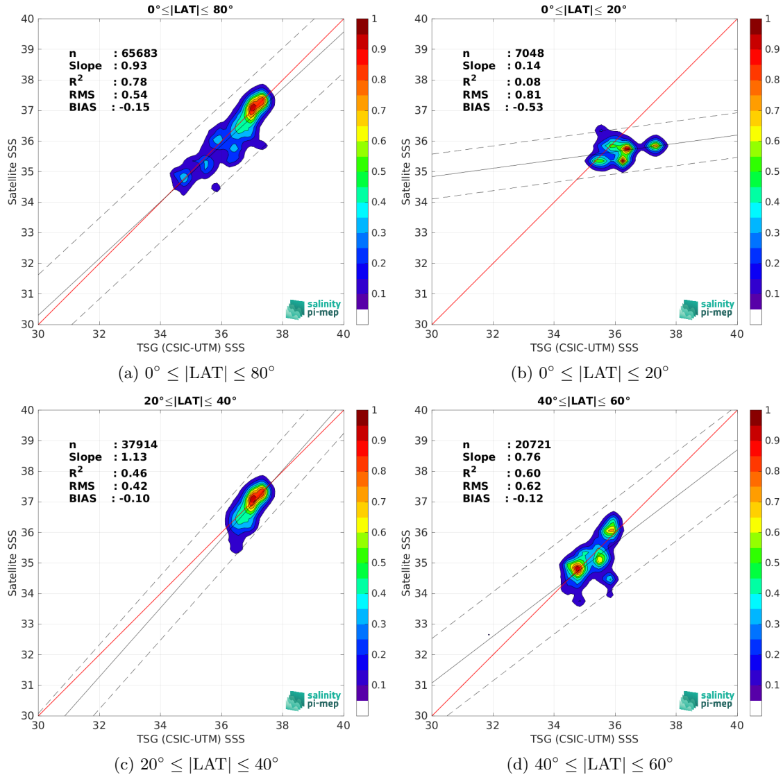
Figure 10: Contour maps of the concentration of Aquarius SSS L2 OR v5 (NASA-GSFC) SSS (y-axis) versus TSG (CSIC-UTM) SSS (x-axis) at match-up pairs for different latitude bands. For each plot, the red line shows x=y . The black thin and dashed lines indicate a linear fit through the data cloud and the \pm 95\% confidence levels, respectively. The number match-up pairs n , the slope and R^2 coefficient of the linear fit, the root mean square (RMS) and the mean bias between satellite and in situ data are indicated for each latitude band in each plots.
