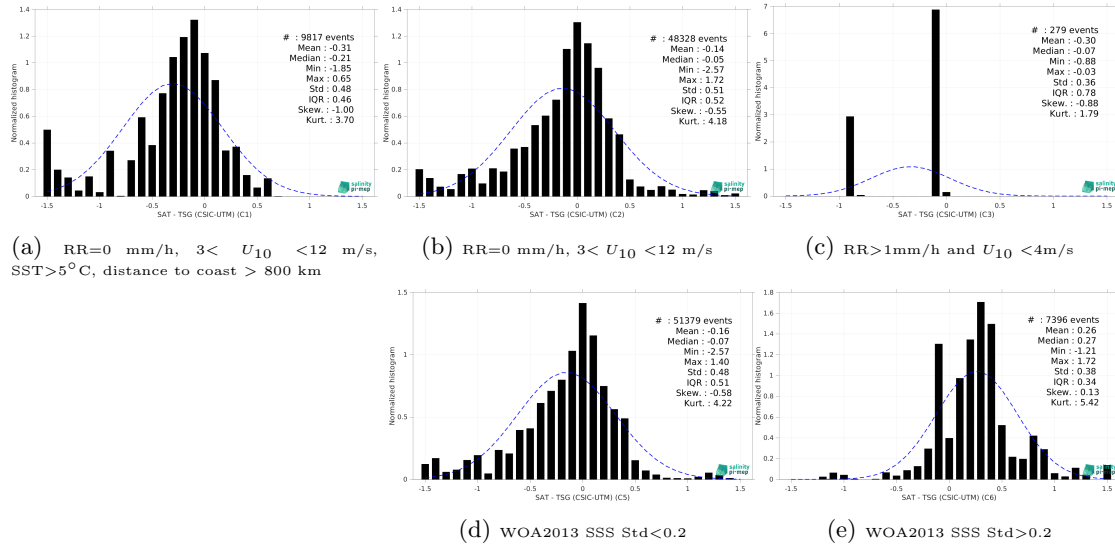
Figure 15: Normalized histogram of \Delta SSS (Aquarius SSS L2 OR v5 (NASA-GSFC) - TSG (CSIC-UTM)) for 5 different subdatasets corresponding to: RR=0 mm/h, 3 < U_{10} < 12 m/s, SST > 5°C, distance to coast > 800 km (a), RR=0 mm/h, 3 < U_{10} < 12 m/s (b), RR > 1mm/h and U_{10} < 4 m/s (c), WOA2013 SSS Std < 0.2 (d), WOA2013 SSS Std > 0.2 (e).
