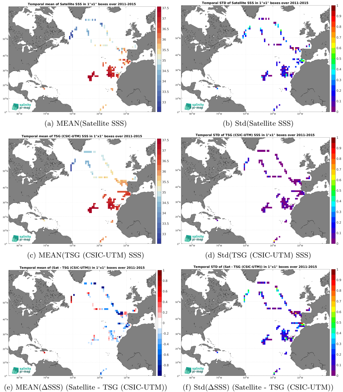
Figure 7: Temporal mean (left) and Std (right) of SSS from Aquarius SSS L2 OR v5 (NASA-GSFC) (top), TSG (CSIC-UTM) (middle), and of \Delta SSS (Satellite - TSG (CSIC-UTM)). Only match-up pairs are used to generate these maps.
