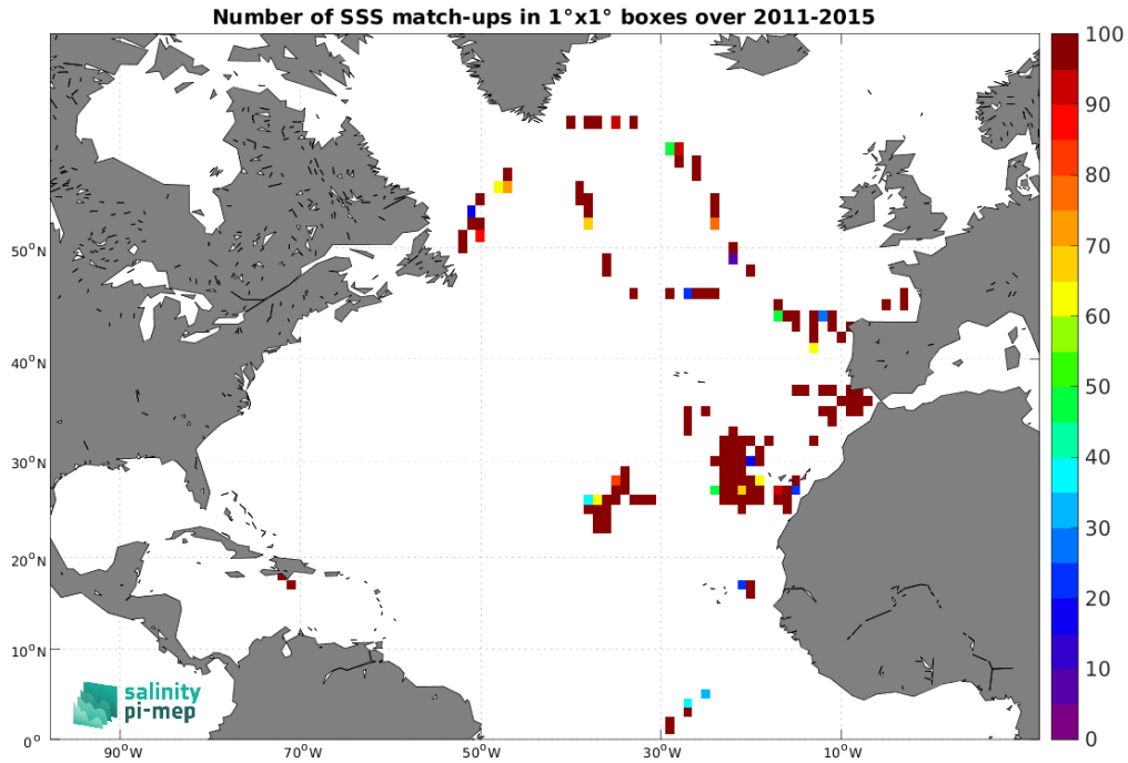
Figure 5: Number of SSS match-ups between TSG (CSIC-UTM) SSS and the Aquarius SSS L2 OR v5 (NASA-GSFC) SSS product for the North Atlantic Ocean Pi-MEP region over 1^\circ \times 1^\circ boxes and for the full satellite product period.
