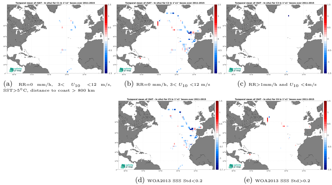
Figure 12: Temporal mean gridded over spatial boxes of size 1^\circ \times 1^\circ of \Delta\text{SSS} (Aquarius SSS L2 OR v5 (NASA-GSFC) - TSG (CSIC-UTM)) for 5 different subdatasets corresponding to:RR=0 mm/h, 3 < U_{10} < 12 m/s, SST >5^\circ\text{C} , distance to coast > 800 km (a), RR=0 mm/h, 3 < U_{10} < 12 m/s (b), RR >1 mm/h and U_{10} < 4 m/s (c), WOA2013 SSS Std <0.2 (d), WOA2013 SSS Std >0.2 (e).
