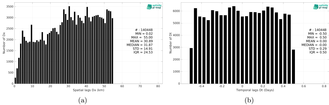
Figure 5: Histograms of the spatial (a) and temporal (b) lags between the location/time of the ICES measurement and the date of the corresponding Aquarius SSS L2 OR v5 (NASA-GSFC) SSS pixel.
