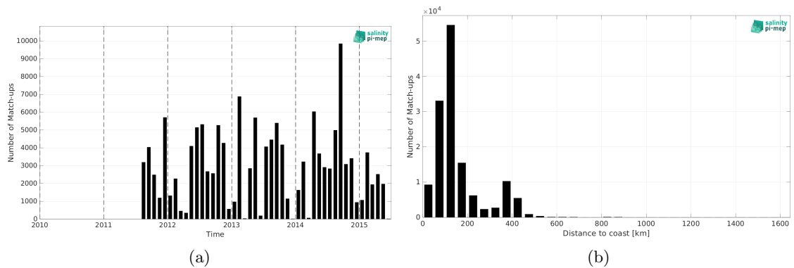
Figure 1: Number of match-ups between ICES and Aquarius SSS L2 OR v5 (NASA-GSFC) SSS as a function of time (a) and as function of the distance to coast (b) over the North Atlantic Ocean Pi-MEP region and for the full satellite product period.
