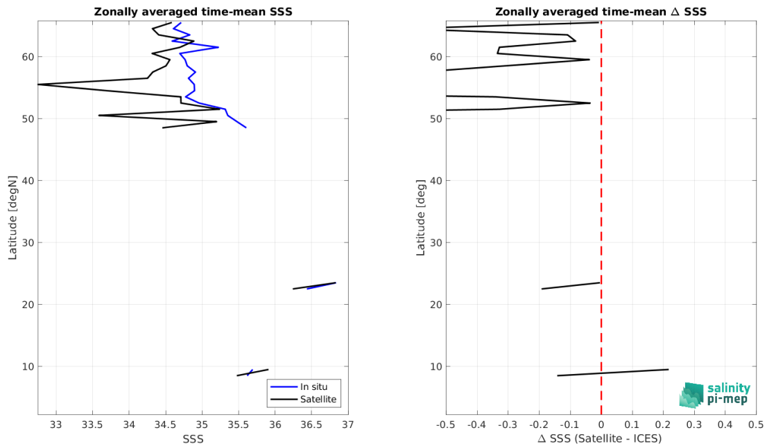
Figure 8: Left panel: Zonal mean SSS from Aquarius SSS L2 OR v5 (NASA-GSFC) satellite product (black) and from ICES (blue). Right panel: Zonal mean of \Delta SSS (Satellite - ICES) for all the collected Pi-MEP match-up pairs estimated over the full satellite product period.
