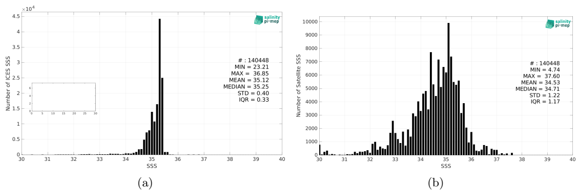
Figure 2: Histograms of SSS from ICES (a) and Aquarius SSS L2 OR v5 (NASA-GSFC) (b) considering all match-up pairs per bins of 0.1 over the North Atlantic Ocean Pi-MEP region and for the full satellite product period.
