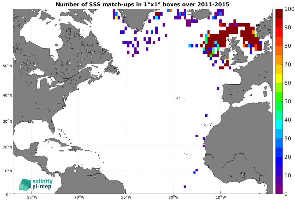
Figure 4: Number of SSS match-ups between ICES SSS and the Aquarius SSS L2 OR v5 (NASA-GSFC) SSS product for the North Atlantic Ocean Pi-MEP region over 1^\circ \times 1^\circ boxes and for the full satellite product period.
