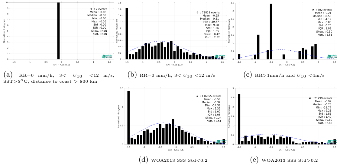
Figure 13: Normalized histogram of \Delta SSS (Aquarius SSS L2 OR v5 (NASA-GSFC) - ICES) for 5 different subdatasets corresponding to: RR=0 mm/h, 3 < U_{10} < 12 m/s, SST > 5°C, distance to coast > 800 km (a), RR=0 mm/h, 3 < U_{10} < 12 m/s (b), RR > 1mm/h and U_{10} < 4 m/s (c), WOA2013 SSS Std < 0.2 (d), WOA2013 SSS Std > 0.2 (e).
