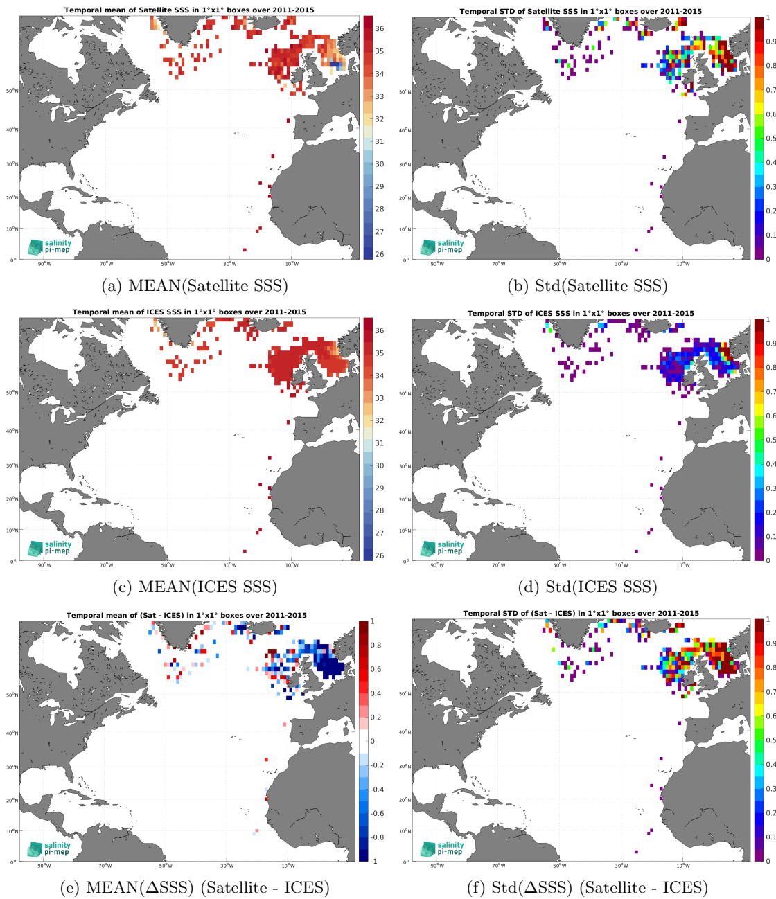
Figure 6: Temporal mean (left) and Std (right) of SSS from Aquarius SSS L2 OR v5 (NASA-GSFC) (top), ICES (middle), and of \Delta SSS (Satellite - ICES). Only match-up pairs are used to generate these maps.
