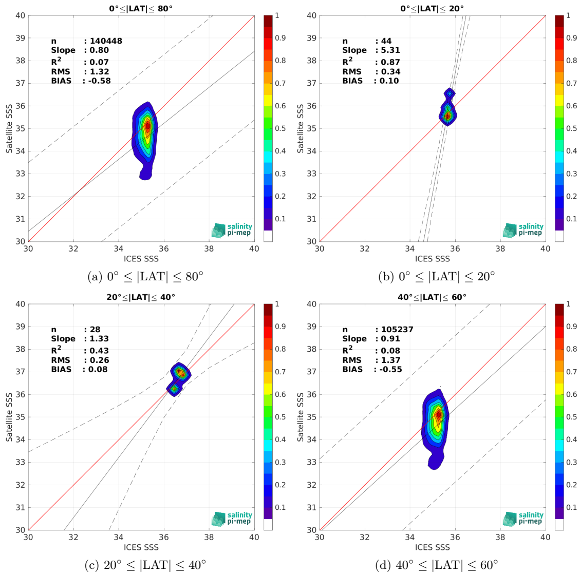
Figure 9: Contour maps of the concentration of Aquarius SSS L2 OR v5 (NASA-GSFC) SSS (y-axis) versus ICES SSS (x-axis) at match-up pairs for different latitude bands. For each plot, the red line shows x=y . The black thin and dashed lines indicate a linear fit through the data cloud and the \pm 95\% confidence levels, respectively. The number match-up pairs n , the slope and R^2 coefficient of the linear fit, the root mean square (RMS) and the mean bias between satellite and in situ data are indicated for each latitude band in each plots.
