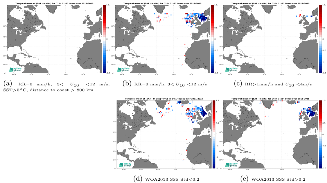
Figure 12: Temporal mean gridded over spatial boxes of size 1^\circ \times 1^\circ of \Delta\text{SSS} (Aquarius SSS L2 OR v5 (NASA-GSFC) - ICES) for 5 different subdatasets corresponding to:RR=0 mm/h, 3 < U_{10} < 12 m/s, SST >5^\circ\text{C} , distance to coast > 800 km (a), RR=0 mm/h, 3 < U_{10} < 12 m/s (b), RR >1 mm/h and U_{10} < 4 m/s (c), WOA2013 SSS Std <0.2 (d), WOA2013 SSS Std >0.2 (e).
