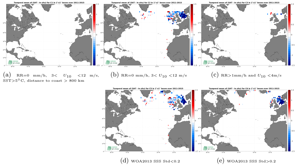
Figure 12: Temporal mean gridded over spatial boxes of size 1^\circ \times 1^\circ of \Delta SSS (Aquarius SSS L2 OR v5 (NASA-GSFC) - ICES) for 5 different subdatasets corresponding to:RR=0 mm/h, 3 < U_{10} < 12 m/s, SST >5^\circ\text{C} , distance to coast > 800 km (a), RR=0 mm/h, 3 < U_{10} < 12 m/s (b), RR >1 mm/h and U_{10} < 4 m/s (c), WOA2013 SSS Std <0.2 (d), WOA2013 SSS Std >0.2 (e).
