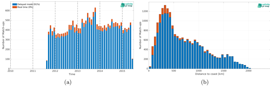
Figure 1: Number of match-ups between Argo and Aquarius SSS L2 OR v5 (NASA-GSFC) SSS as a function of time (a) and as function of the distance to coast (b) over the North Atlantic Ocean Pi-MEP region and for the full satellite product period.
