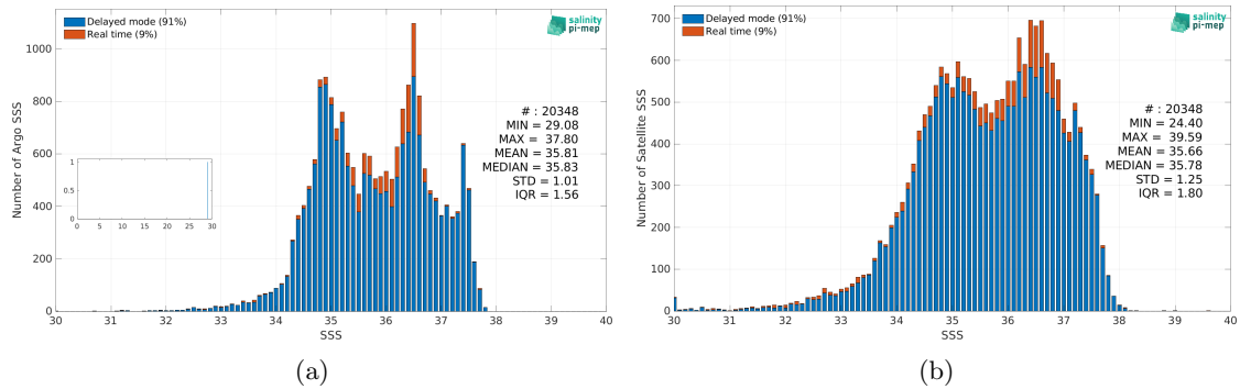
Figure 2: Histograms of SSS from Argo (a) and Aquarius SSS L2 OR v5 (NASA-GSFC) (b) considering all match-up pairs per bins of 0.1 over the North Atlantic Ocean Pi-MEP region and for the full satellite product period.
