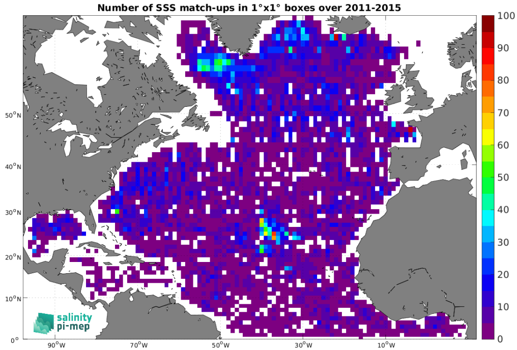
Figure 4: Number of SSS match-ups between Argo SSS and the Aquarius SSS L2 OR v5 (NASA-GSFC) SSS product for the North Atlantic Ocean Pi-MEP region over 1^\circ \times 1^\circ boxes and for the full satellite product period.
