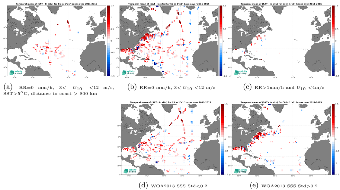
Figure 14: Temporal mean gridded over spatial boxes of size 1^\circ \times 1^\circ of \Delta SSS (Aquarius SSS L2 CAP v5 (JPL) - TSG (SAMOS)) for 5 different subdatasets corresponding to: RR=0 mm/h, 3 < U_{10} < 12 m/s, SST > 5°C, distance to coast > 800 km (a), RR=0 mm/h, 3 < U_{10} < 12 m/s (b), RR > 1mm/h and U_{10} < 4 m/s (c), WOA2013 SSS Std < 0.2 (d), WOA2013 SSS Std > 0.2 (e).
