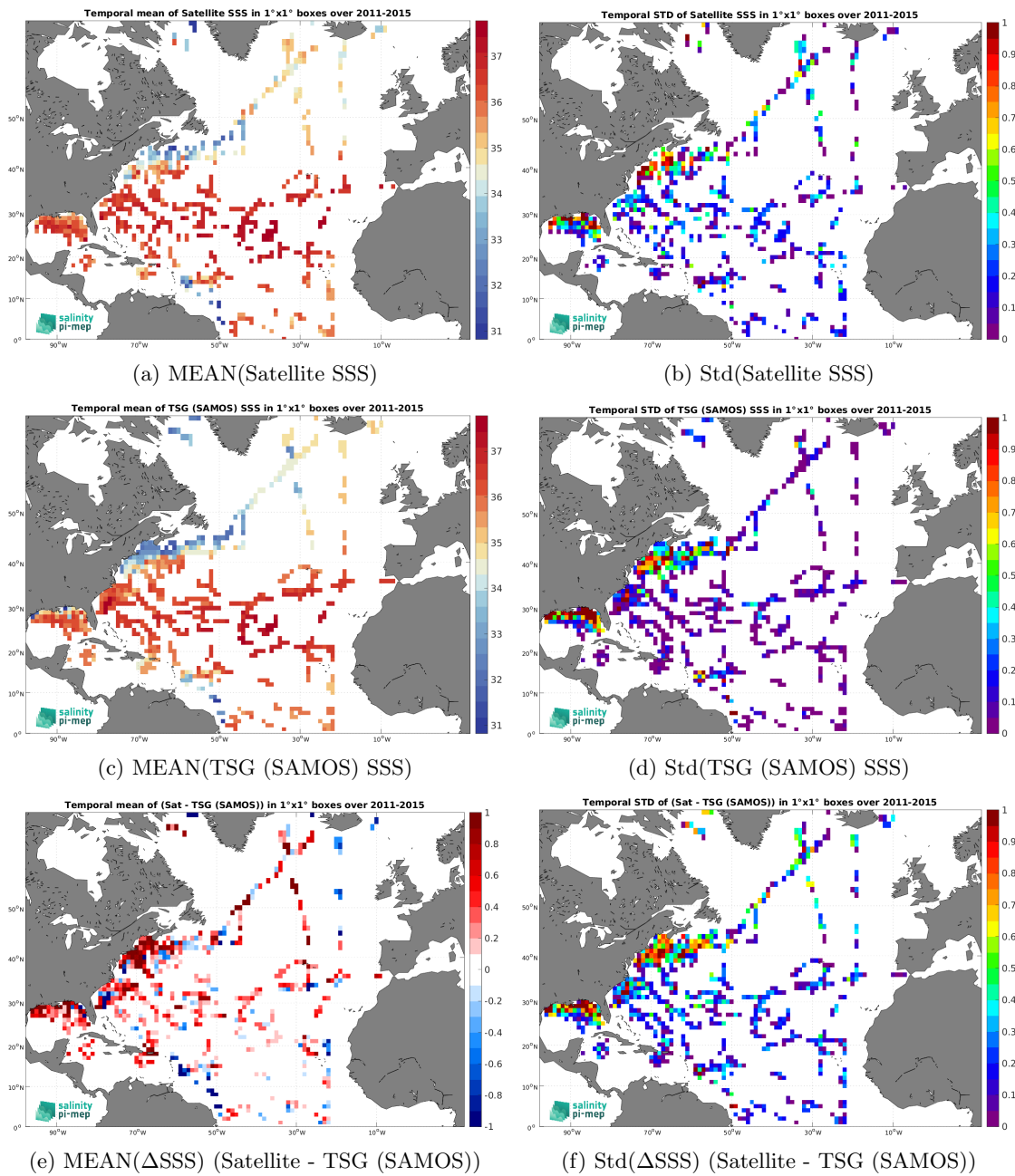
Figure 7: Temporal mean (left) and Std (right) of SSS from Aquarius SSS L2 CAP v5 (JPL) (top), TSG (SAMOS) (middle), and of \Delta SSS (Satellite - TSG (SAMOS)). Only match-up pairs are used to generate these maps.
