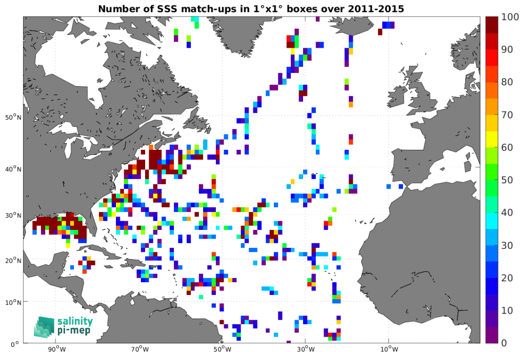
Figure 5: Number of SSS match-ups between TSG (SAMOS) SSS and the Aquarius SSS L2 CAP v5 (JPL) SSS product for the North Atlantic Ocean Pi-MEP region over 1^\circ \times 1^\circ boxes and for the full satellite product period.
