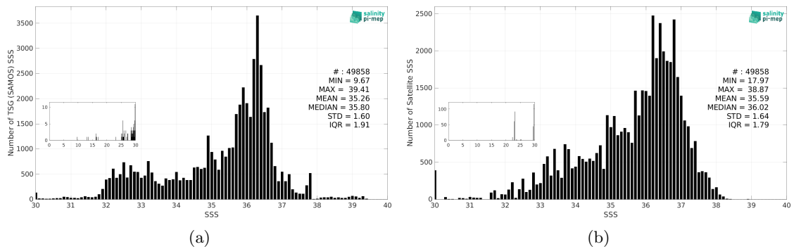
Figure 3: Histograms of SSS from TSG (SAMOS) (a) and Aquarius SSS L2 CAP v5 (JPL) (b) considering all match-up pairs per bins of 0.1 over the North Atlantic Ocean Pi-MEP region and for the full satellite product period.
