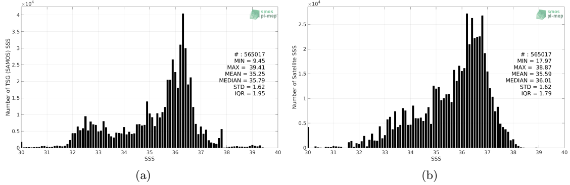
Figure 2: Histograms of SSS from TSG (SAMOS) (a) and Aquarius SSS L2 CAP v5 (JPL) (b) considering all match-up pairs per bins of 0.1 over the North Atlantic Ocean Pi-MEP region and for the full satellite product period.
