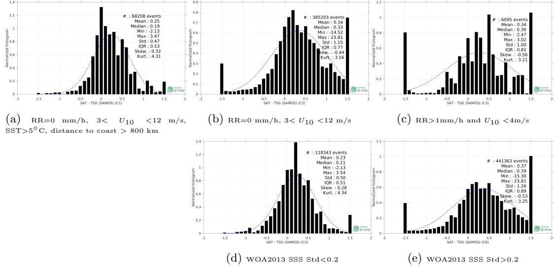
Figure 13: Normalized histogram of \Delta SSS (Aquarius SSS L2 CAP v5 (JPL) - TSG (SAMOS)) for 5 different subdatasets corresponding to: RR=0 mm/h, 3 < U_{10} < 12 m/s, SST > 5^\circ\text{C} , distance to coast > 800 km (a), RR=0 mm/h, 3 < U_{10} < 12 m/s (b), RR > 1 mm/h and U_{10} < 4 m/s (c), WOA2013 SSS Std < 0.2 (d), WOA2013 SSS Std > 0.2 (e).
