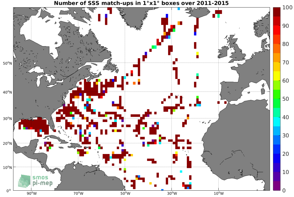
Figure 4: Number of SSS match-ups between TSG (SAMOS) SSS and the Aquarius SSS L2 CAP v5 (JPL) SSS product for the North Atlantic Ocean Pi-MEP region over 1^\circ \times 1^\circ boxes and for the full satellite product period.
