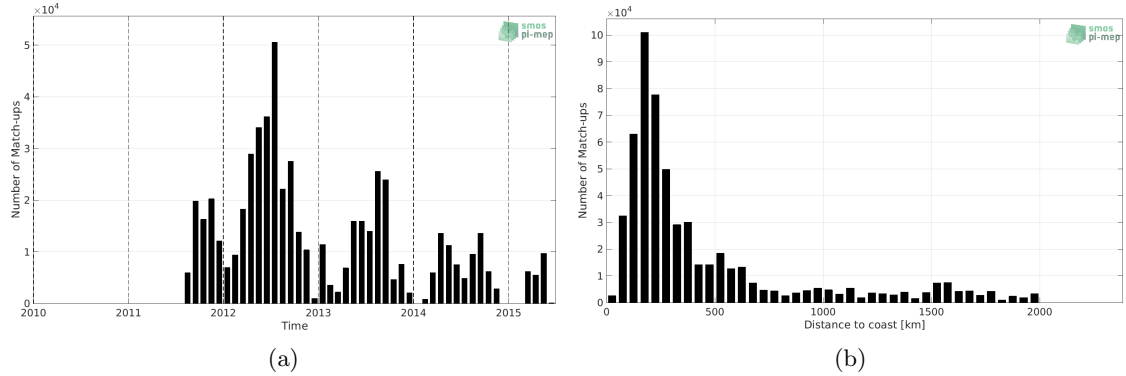
Figure 1: Number of match-ups between TSG (SAMOS) and Aquarius SSS L2 CAP v5 (JPL) SSS as a function of time (a) and as function of the distance to coast (b) over the North Atlantic Ocean Pi-MEP region and for the full satellite product period.
