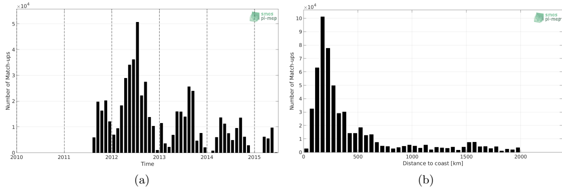
Figure 1: Number of match-ups between TSG-SAMOS and Aquarius-L2-JPL-V5 SSS as a function of time (a) and as function of the distance to coast (b) over the North Atlantic Ocean Pi-MEP region and for the full satellite product period.
