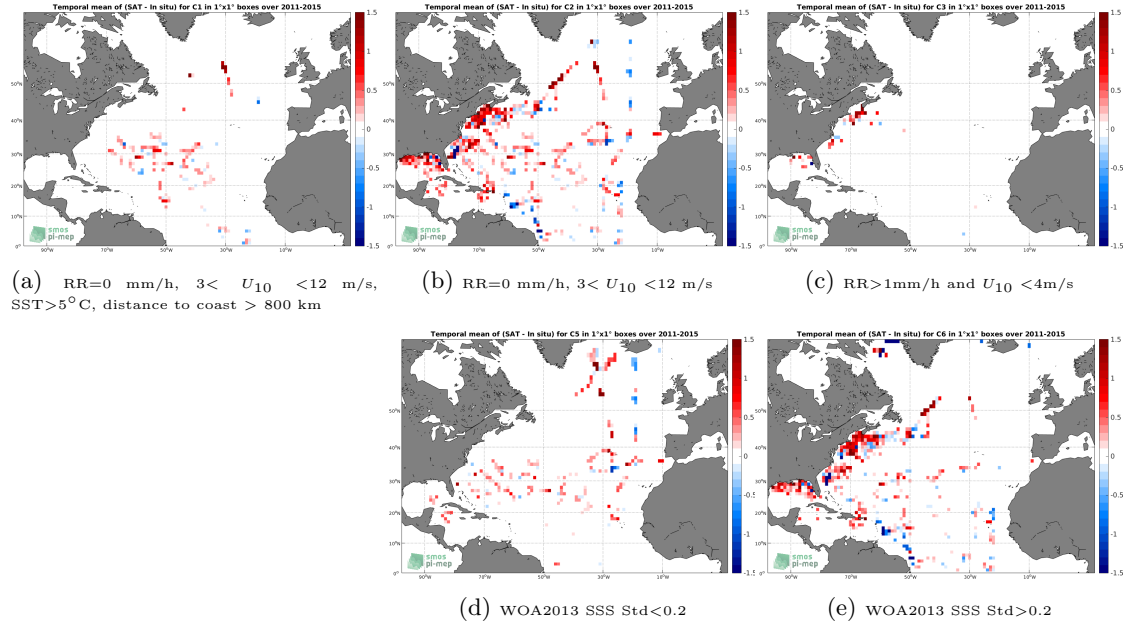
Figure 12: Temporal mean gridded over spatial boxes of size 1^\circ \times 1^\circ of \Delta SSS (Aquarius-L2-JPL-V5 - TSG-SAMOS) for 5 different subdatasets corresponding to: RR=0 mm/h, 3 < U_{10} < 12 m/s, SST >5^\circ C, distance to coast > 800 km (a), RR=0 mm/h, 3 < U_{10} < 12 m/s (b), RR >1 mm/h and U_{10} < 4 m/s (c), WOA2013 SSS Std <0.2 (d), WOA2013 SSS Std >0.2 (e).
